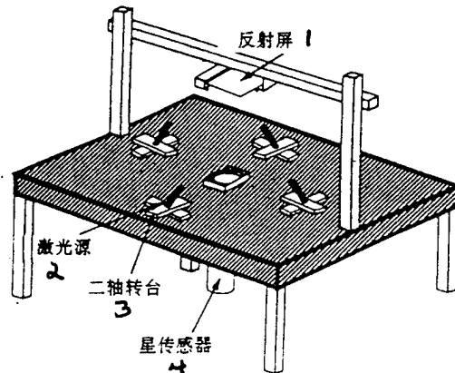
Fig. 5 Stellar simulator
