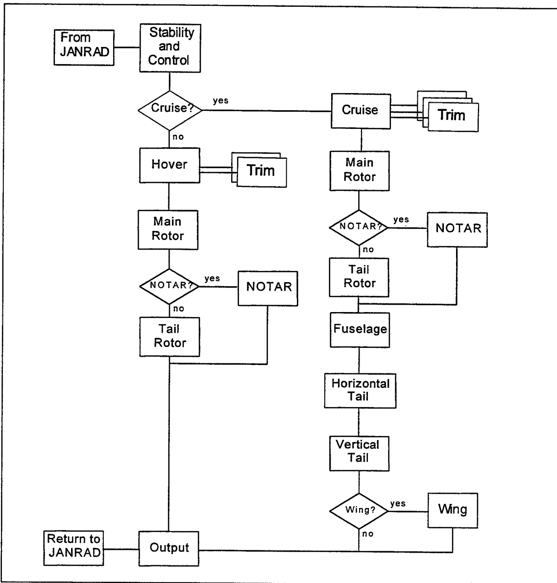
Figure 2.1 JANRAD Architecture
