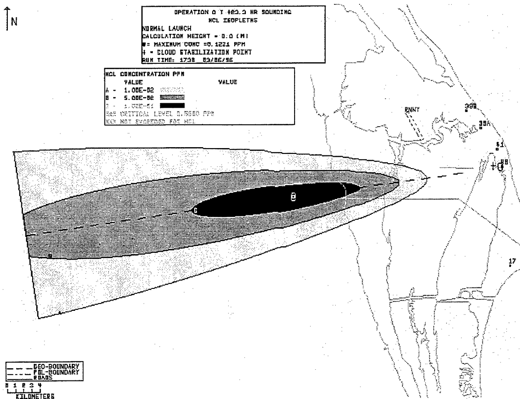
Figure 5: REEDM's Surface Impact Prediction for Cloud Isopleths Using T-0.7h Rawinsonde Data
