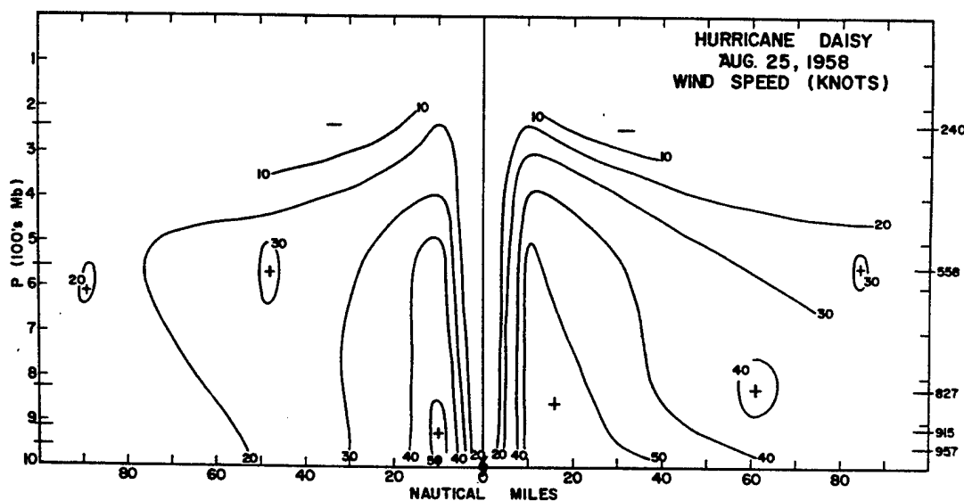
Figure 6.5: Vertical cross-section of v_t of Hurricane Daisy on 12 UTC 25 August 1958. Winds include storm motion. Cross-section is perpendicular to direction of storm motion. From Colón (1961).
