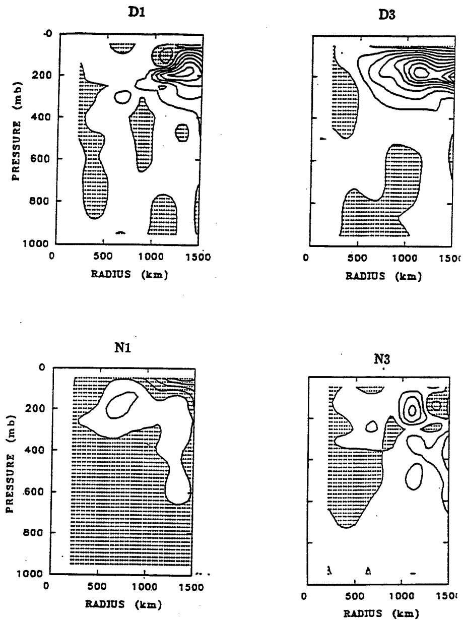
Figure 2.6: Calculations of inward eddy flux of momentum -ru'_r v'_\theta for prehurricane cloud cluster (D1), intensifying tropical storm or depression (D3), nondeveloping cloud cluster (N1), and nondeveloping depression (N3). Shading is outward flux. Contour interval is 80 \text{deg m}^2 \text{s}^{-2} . From Challa and Pfeffer (1990) as classified by McBride (1981).
