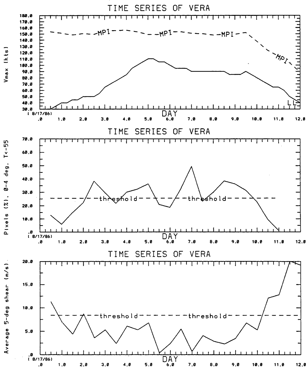
Figure 8.9: Time series of MPI and V_{max} (kts, top figure), PX0455 with its threshold value for reference (%; middle figure), and VWS5 with its threshold value for reference ( \text{m s}^{-1} ; bottom figure) for Typhoon Vera (1986). "L" denotes land interaction on Days 11.5 and 11.75.
