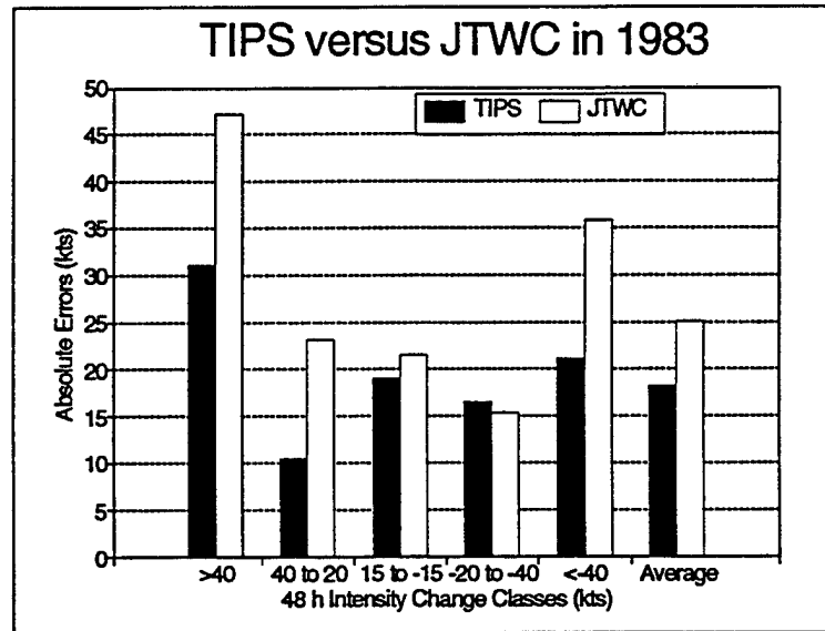
Figure 8.6: Absolute 48-h errors for TIPS and JTWC on the independent data set (1983) for different \Delta V_{max} classes and overall average. TIPS is developed on perfect-prog forecasts of shear and track, so this figure does not imply that TIPS can outperform JTWC.
