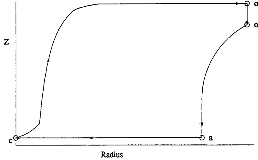
Figure 3.12: The hurricane Carnot Cycle. Air spirals in toward the storm center from point a , acquiring moist entropy from the ocean surface at fixed T_{sea} . It then ascends adiabatically from point c flowing out near the storm top to some large radius (point o ). The excess entropy is lost by isothermal radiational cooling between point o and o' at a much cooler mean outflow temperature \bar{T}_{out} . The cycle is closed by traveling along the path dry adiabatically from point o' to a . The adiabatic paths are also assumed to be along constant absolute angular momentum lines, and therefore the eyewall motion represents slantwise convection. Adapted from Emanuel (1991).
