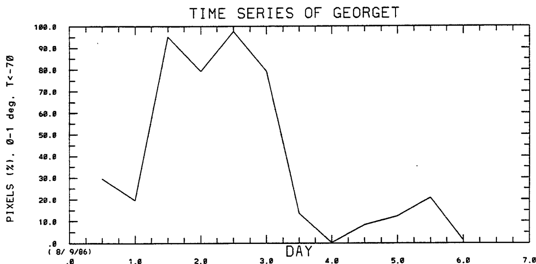
Figure 5.3: Example of pixel count time series expressed as percentage of pixels with T_b < -70^\circ\text{C} in a 0-1-deg area. Storm is Typhoon Georget (1986).
