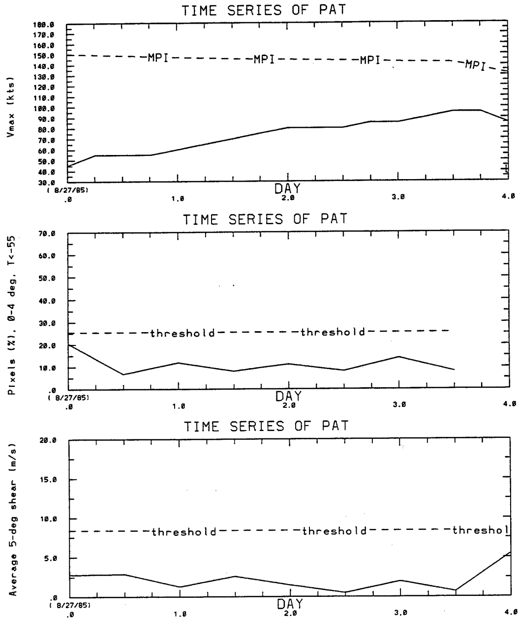
Figure 8.11: Time series of MPI and V_{max} (kts, top figure), PX0455 with its threshold value for reference (%) middle figure), and VWS5 with its threshold value for reference ( \text{m s}^{-1} ; bottom figure) for Typhoon Pat (1985). "L" denotes land interaction on Day 4.
