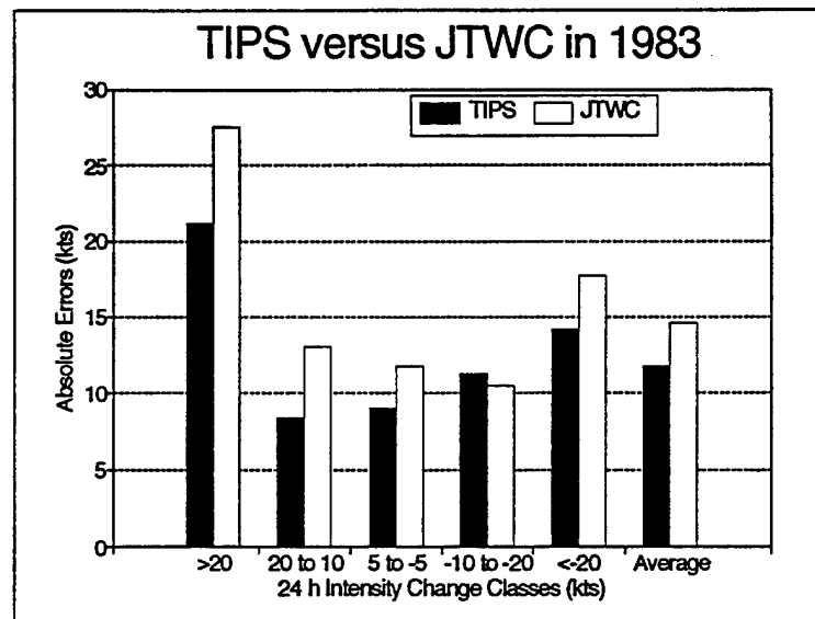
Figure 8.5: Absolute 24-h errors for TIPS and JTWC on the independent data set (1983) for different \Delta V_{max} classes and overall average. TIPS is developed on perfect-prog forecasts of shear and track, so this figure does not imply that TIPS can outperform JTWC.
