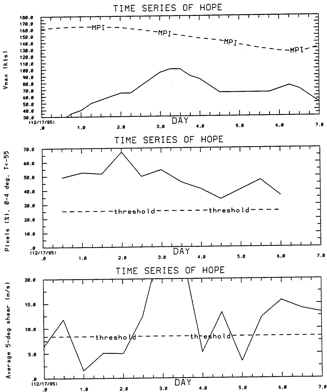
Figure 8.10: Time series of MPI and V_{max} (kts, top figure), PX0455 with its threshold value for reference (%; middle figure), and VWS5 with its threshold value for reference ( \text{m s}^{-1} ; bottom figure) for Typhoon Hope (1985).
