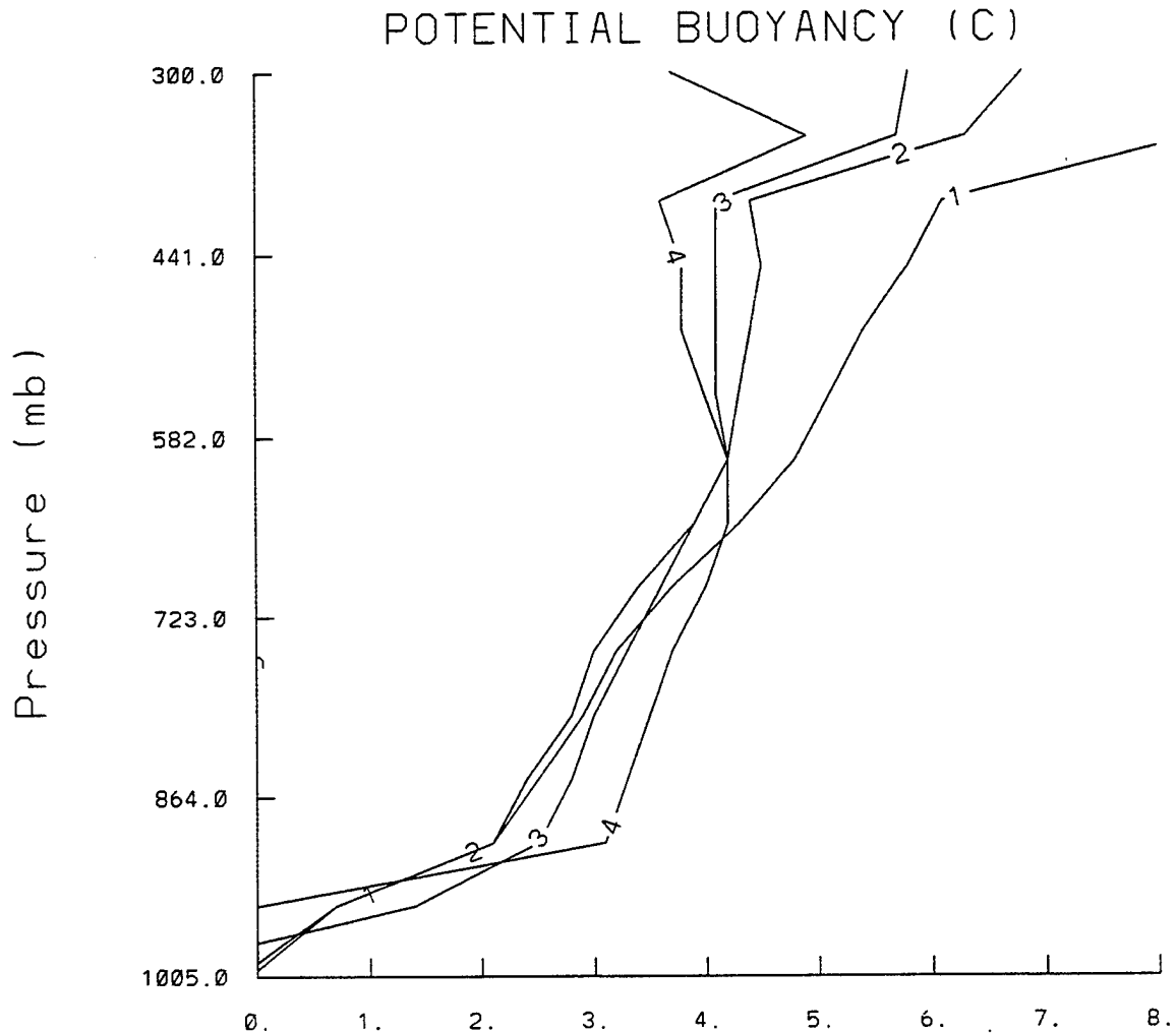
Figure 7.9: Potential buoyancy (defined as \tilde{T}_p(p) minus T_v(p) ) of the eyewall environment for the four stages shown in Fig. 7.8. Stages 1–4 represent buoyancy calculations from the weak to strongest TC intensity regimes. CAPE values upon integration from the surface to 300 mb are 864, 753, 764, and 782 \text{J kg}^{-1} . Computations are shown only to 300 mb, since above this level the eyewall slopes outwards away from the temperature anomaly, and calculations based on vertical ascent of air parcels would not be representative of buoyancy in the eyewall. These profiles are labeled “potential buoyancy” because undilute ascent is assumed.
