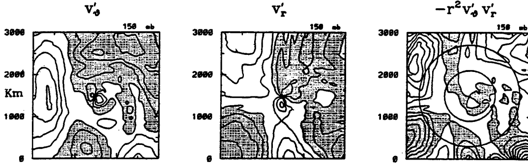
Figure 2.7: Horizontal distributions of v'_t , u'_r , and -r^2 v'_t u'_r for the prehurricane cloud cluster D1 which is centered in the middle of each box. Contour interval for v'_t and u'_r is 4 \text{ m s}^{-1} . Contour interval for -r^2 v'_t u'_r is 4000 \text{ deg}^2 \text{ m}^2 \text{ s}^{-2} . The shaded region represents anticyclonic tangential velocity, outward radial velocity, and outward eddy flux of angular momentum. From Pfeffer and Challa (1993).
