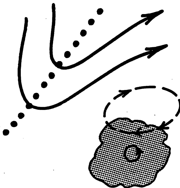
Figure 2.18: Illustration of the minimal shear associated with an anticyclone downstream of a trough. The location of a trough to the northwest of a TC may just indicate a favorable shear environment downstream, with minimal environmental interaction in the vicinity of the TC.
