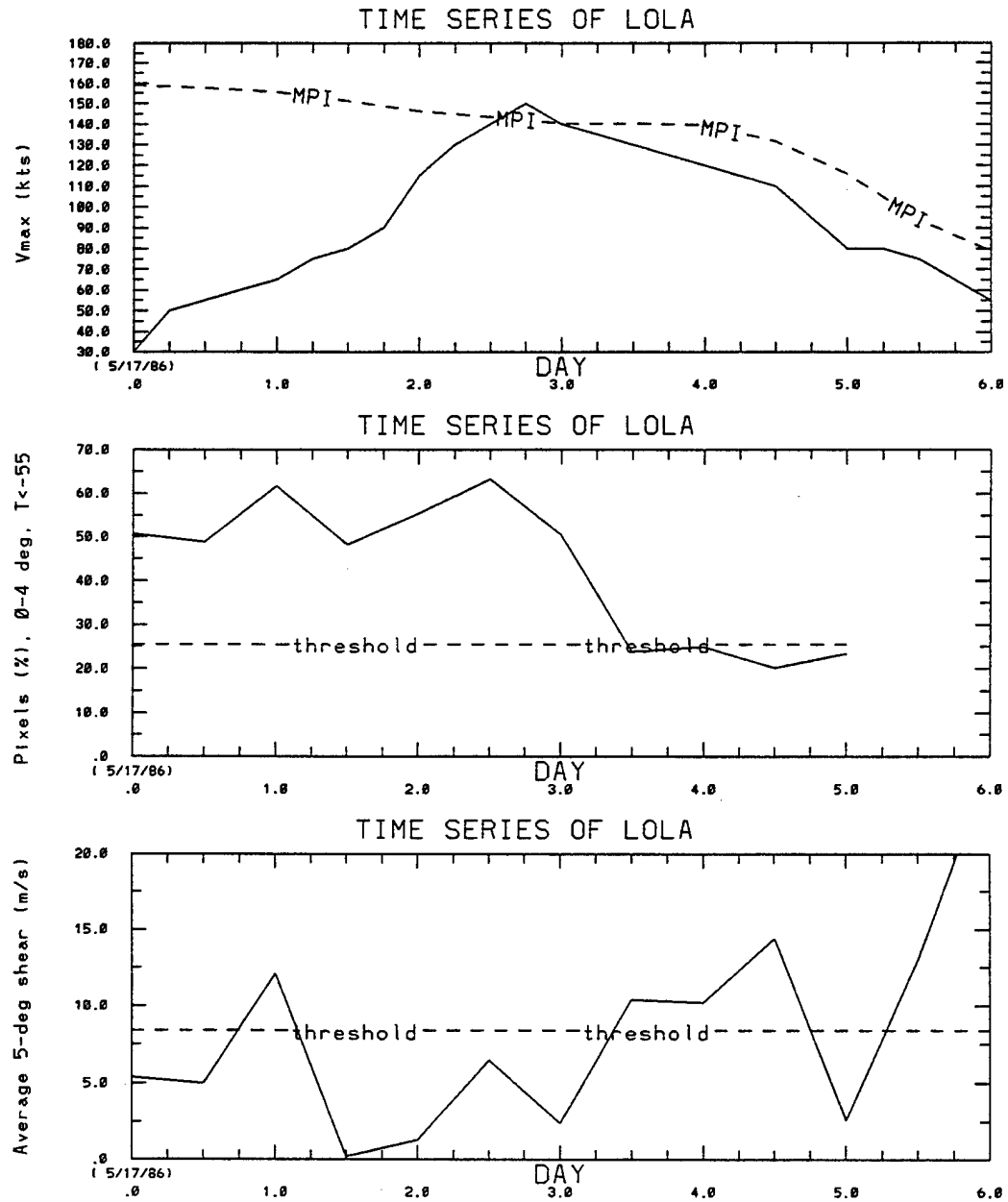
Figure 8.8: Time series of MPI and V_{max} (kts, top figure), PX0455 with its threshold value for reference (%; middle figure), and VWS5 with its threshold value for reference ( \text{m s}^{-1} ; bottom figure) for Typhoon Lola (1986).
