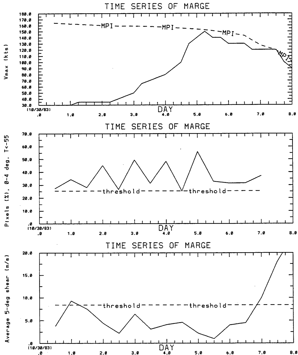
Figure 8.13: Time series of MPI and V_{max} (kts, top figure), PX0455 with its threshold value for reference (%; middle figure), and VWS5 with its threshold value for reference ( \text{m s}^{-1} ; bottom figure) for Typhoon Marge (1983).
