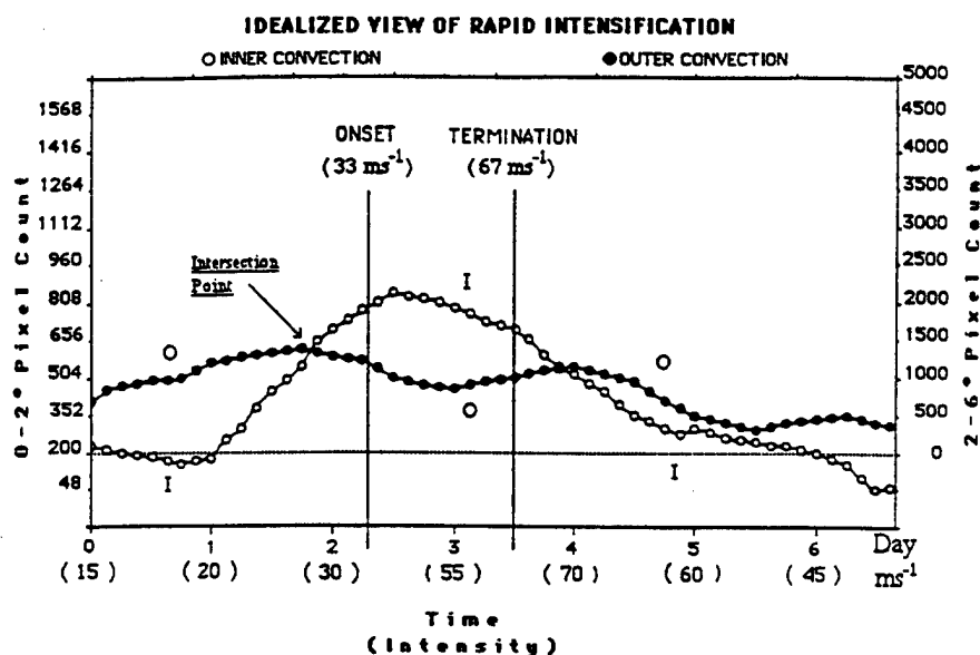
Figure 4.2: Illustration of an idealized rapid intensification event predicted by the intersection of the relative concentrations of inner (0 to 2-deg radii) pixels colder than -75^{\circ}C versus outer (2 to 6-deg radii) pixels colder than -65^{\circ}C . According to Mundell (1990), as long as all climatological parameters are favorable, the onset of rapid intensity change is likely within 12 h. Taken from Mundell (1990).
