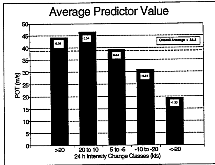
Figure 8.3: Average POT values for different 24-h \Delta V_{max} classes. Numbers on the bars are normalized standard deviations ( NSD ) defined by (\bar{x}c - \bar{x})/\sigma , where \bar{x}c is the average POT value for each class and \sigma is POT's standard deviation in the sample. The sample average ( \bar{x} ; denoted by the dashed line) is shown for comparison.
