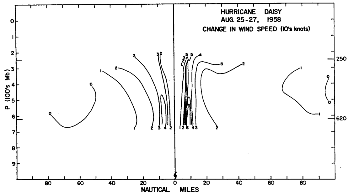
Figure 6.7: Changes in v_i between 12 UTC 25 August (Fig. 6.5) and 18 UTC 27 August (Fig. 6.6) 1958 for Hurricane Daisy. From Colón (1961).
