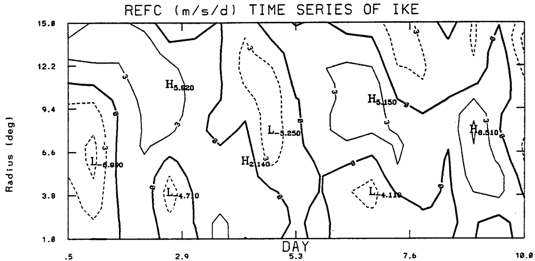
Figure 8.7: Radius-time series (Hovmoeller) diagram of 1-15 deg REFC for Typhoon Ike from Day 0.5 (12 UTC 26 August 1984) to Day 10 (00 UTC 5 September 1984). The REFC event on Day 3 preceded the rapid intensification of Ike on Day 5. However, small vertical wind shear, warm SSTs, and favorable 0-4 deg convection probably played the dominant intensification role. Contour interval is 3 \text{ ms}^{-1} \text{ d}^{-1} .
