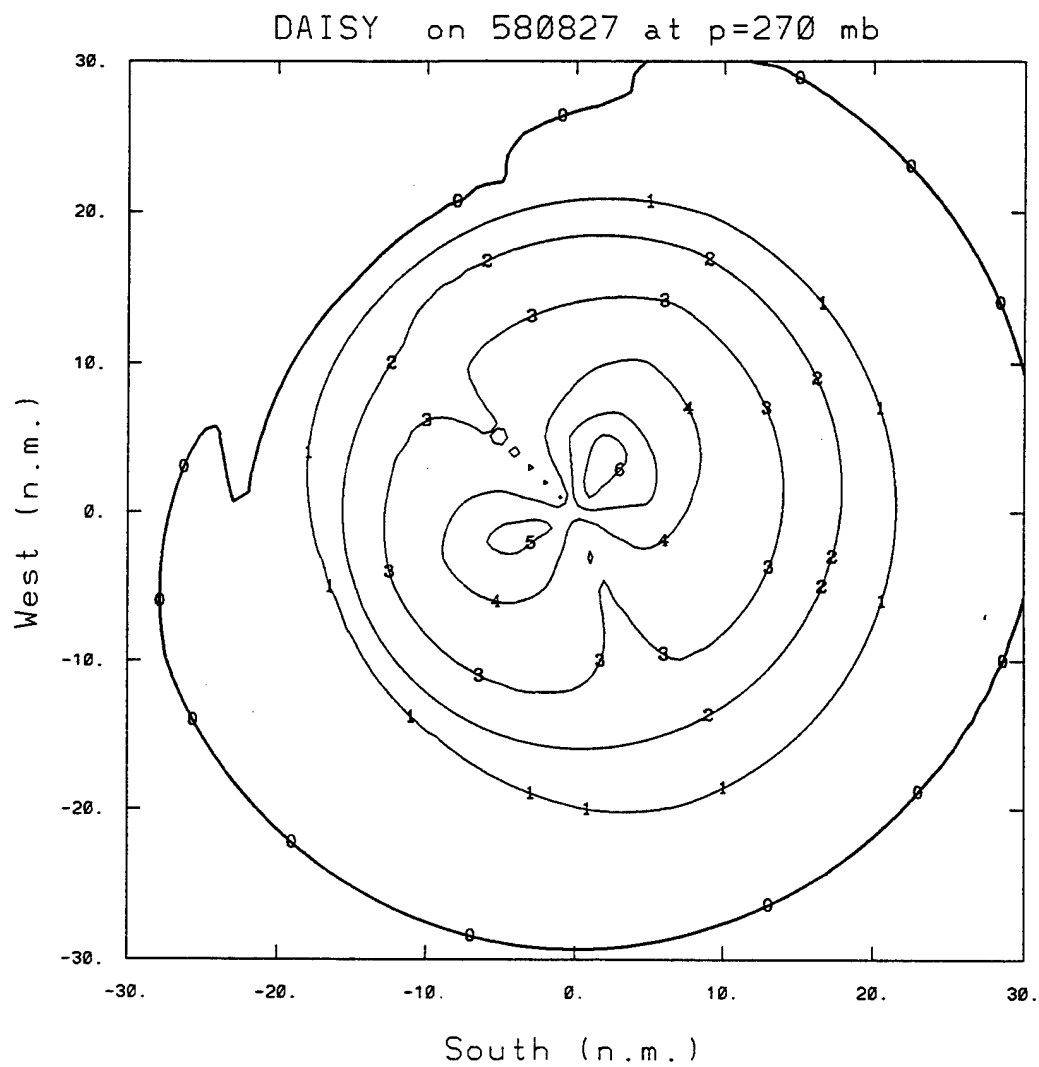
Figure 6.26: Plan-view of temperature deviations for deepening Hurricane Daisy on 1730 UTC 27 August 1958. Pressure level is 270 mb. Contour interval is 1°C.
