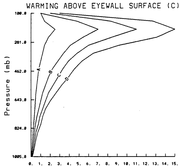
Figure 7.7: Hypothetical development of the eyewall temperature perturbation relative to the western North Pacific mean tropical sounding (Frank 1977b; Gray and Frank 1977). The corresponding surface pressures under the eyewall are 994.3 (A), 979.1 (B), 965.9 (C), and 949.7 mb (D). These temperature profiles represent the TC from its minimal tropical storm stage to its MPI stage.
