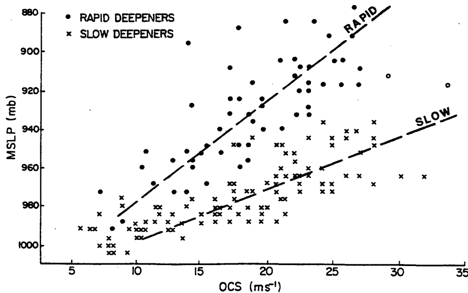
Figure 4.1: Scatter diagram of intensity (MSLP) versus OCS at onset of rapid deepening (denoted by circles) and at onset of slow deepening (denoted by X's). Taken from Weatherford and Gray (1989).
