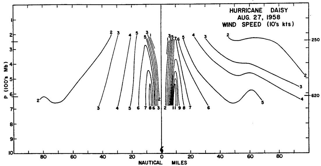
Figure 6.6: Same as Fig. 6.5, but for 18 UTC 27 August 1958. From Colón (1961).
