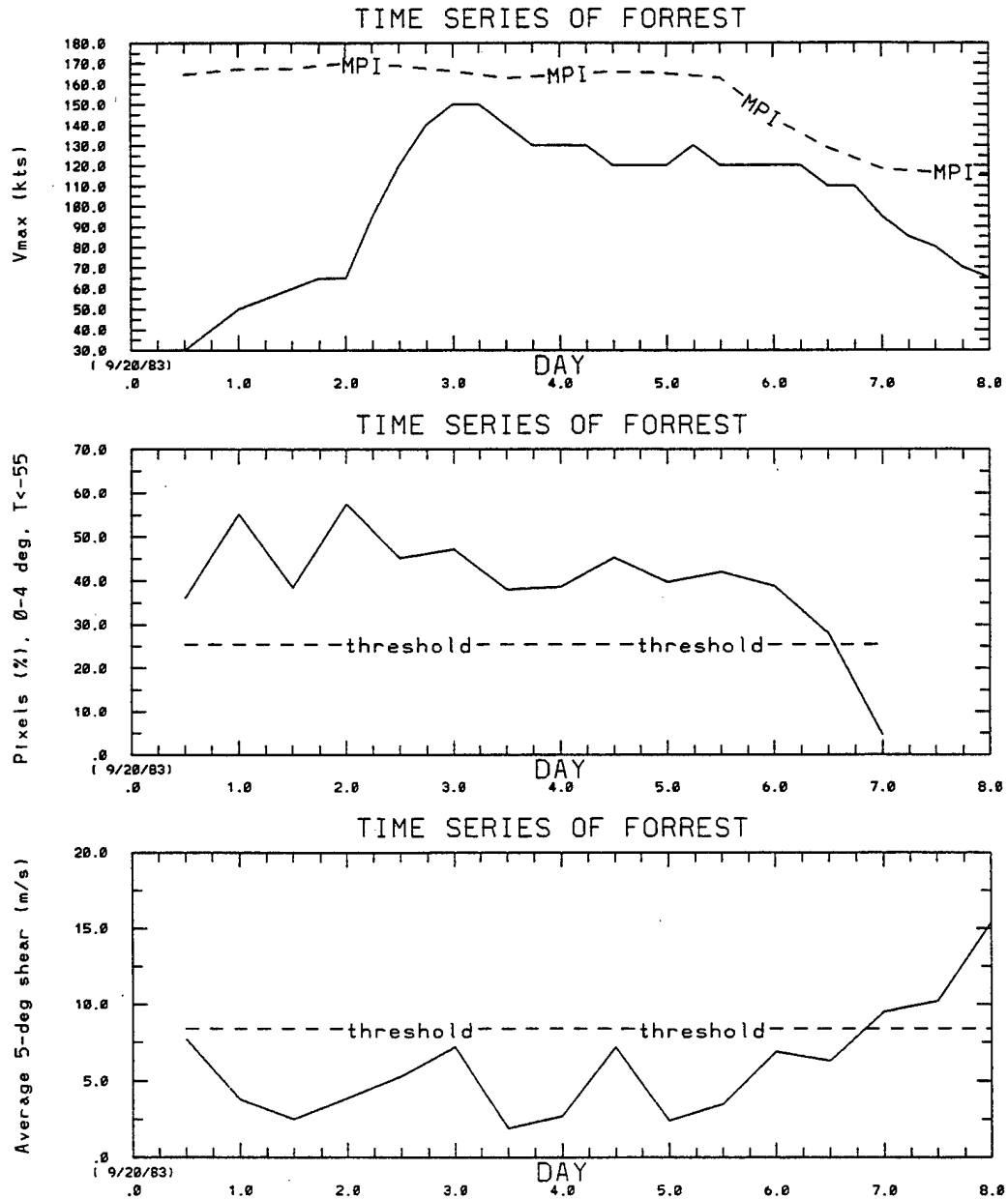
Figure 8.14: Time series of MPI and V_{max} (kts, top figure), PX0455 with its threshold value for reference (%; middle figure), and VWS5 with its threshold value for reference ( \text{m s}^{-1} ; bottom figure) for Typhoon Forrest (1983).
