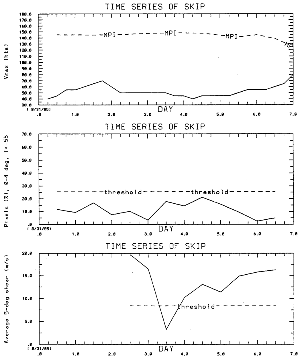
Figure 8.12: Time series of MPI and V_{max} (kts, top figure), PX0455 with its threshold value for reference (%) middle figure), and VWS5 with its threshold value for reference ( m s^{-1} ; bottom figure) for Typhoon Skip (1985). VWS5 was not available on Days 0-2.0 and on Day 7 since the TC was located east of 175 deg E, and 5-deg areally averaged shear could not be computed in the BMRC data set (which is restricted to 180 deg E).
