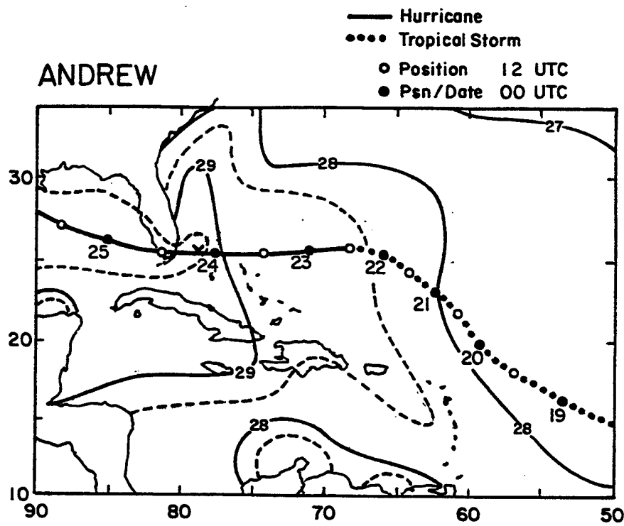
Figure 3.1: SSTs ( ^{\circ}\text{C} ) for August 1992 (Reynolds and Smith 1994). Andrew's path is also shown.
