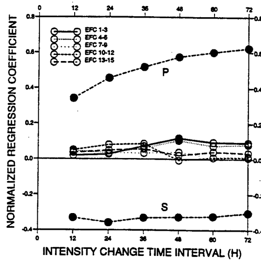
Figure 2.14: Normalized regression coefficients for areally averaged vertical shear (S), a potential intensity change variable based on SST ( P = VSST - V_{max} ), and the relative eddy angular momentum flux convergence (EFC) in each radial band (1-3 denotes the 100-300-km average, 4-6 denotes the 400-600-km average, etc.). A multiple regression was performed that included three independent variables (EFC in a given radial band, P, and S) for each intensity change time interval (12, 24, 36, 48, 60, and 72 h). The circles are filled for coefficients that were significant at the 95% level. P is a significant positive predictor at all time intervals (regression coefficient between 0.4 and 0.6), S is a significant negative predictor at all time intervals (regression coefficient between -0.3 and -0.4), and EFC is a slight positive contributor at all time levels and at all radii (regression coefficient between 0 and 0.1) but only significant within 600 km at 48 h. From DeMaria et al. (1993).
