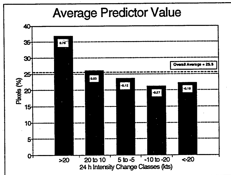
Figure 8.4: Average PX0455 values for different 24-h \Delta V_{max} classes. Numbers on the bars are normalized standard deviations ( NSD ) defined by (\bar{x}c - \bar{x})/\sigma , where \bar{x}c is the average PX0455 value for each class and \sigma is PX0455's standard deviation in the sample. The sample average ( \bar{x} ; denoted by the dashed line) is shown for comparison.
