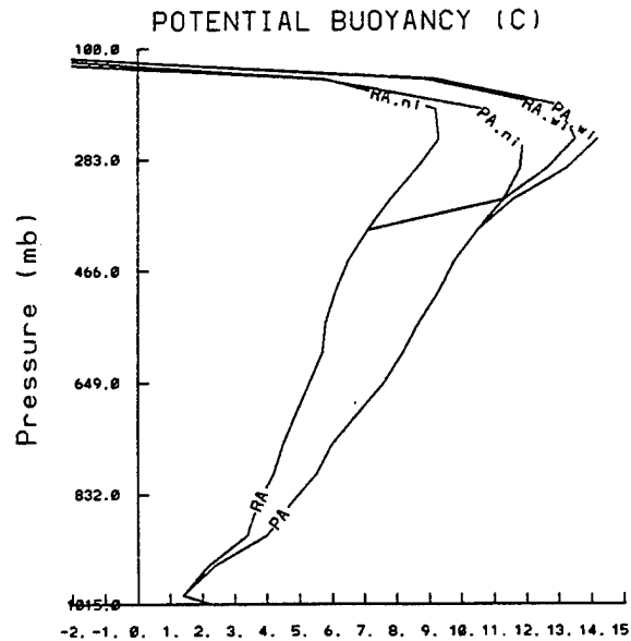
Figure 7.5: Potential buoyancy profiles (defined as T_p - T_{v_{env}} ) relative to the Jordan (1958) mean "hurricane season" sounding. A surface temperature of 28°C is assumed with a surface relative humidity of 90%. RA.ni represents the reversible process with no ice, and PA.ni represents the pseudoadiabatic process with no ice. The processes with "wi" contain ice. The freezing level is assumed at T = -10^\circ\text{C} . These profiles are labeled "potential buoyancy" because undilute ascent is assumed.
