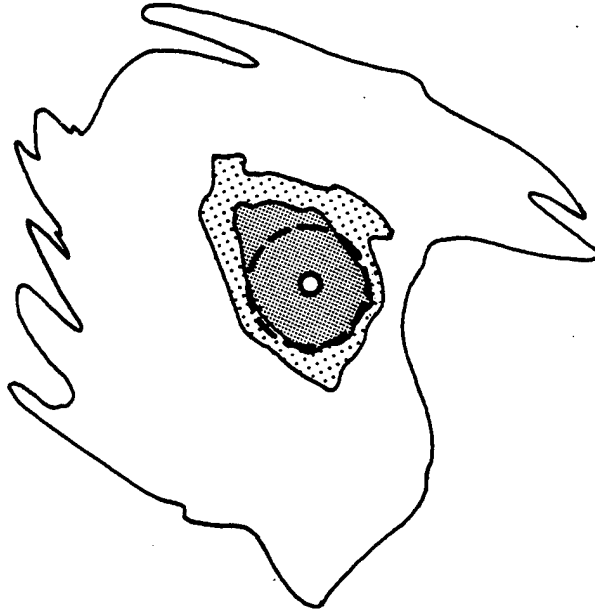
Figure 3.6: Draft of Hurricane Andrew on 21 UTC 22 August 1995. The light shading denotes cloud tops with brightness temperature colder than -55^{\circ}\text{C} , and dark shading colder than -65^{\circ}\text{C} . The outline represents the edge of the warmer clouds. An eye is also evident inside the cloud canopy. The circle denotes 1 deg radius.
