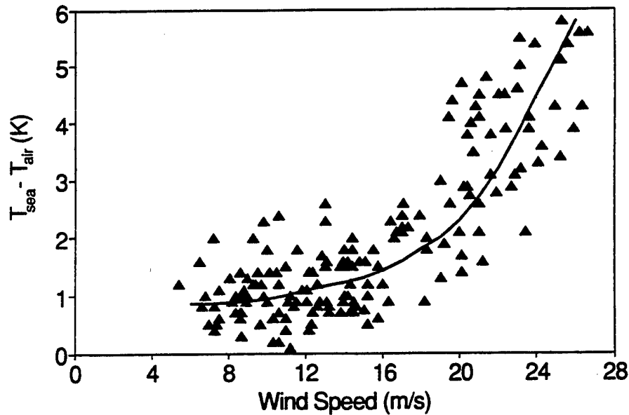
Figure 7.1: Measurements taken aboard the research ship Priliv in 1988. The plot shows the SST minus air temperature difference ( ^{\circ}\text{K} ) versus wind speed ( \text{m s}^{-1} ) in TCs Tess and Skip. Taken from Fairall et al. (1994), who adapted the figure from Pudov (1992).
