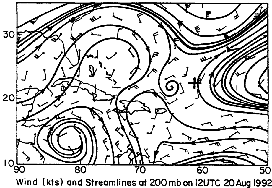
Figure 3.2: Aviation model 200-mb wind barbs and streamlines on 12 UTC 20 August 1992. Andrew is located at +.
