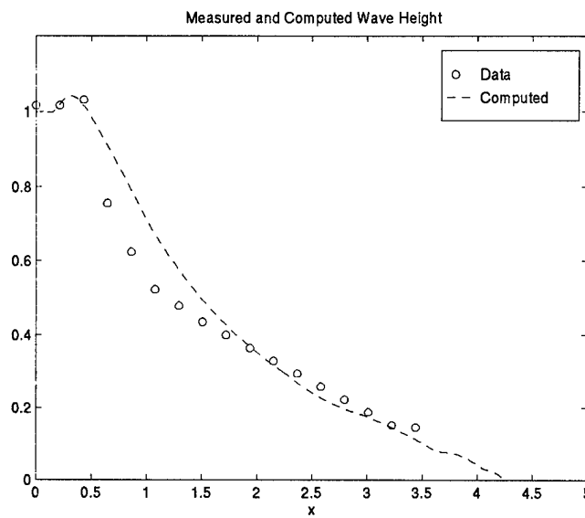
Figure 4.14: Cross-shore variation of the measured and computed normalized wave height.
