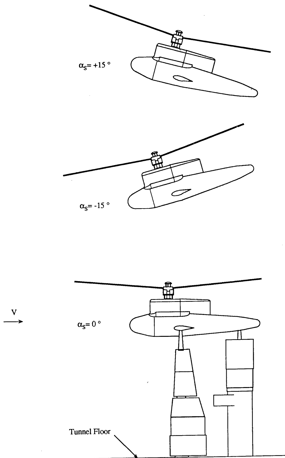
Figure 3(c). Sideview of model in tunnel test section \alpha_s = 0 deg, -15 deg and 15 deg.
