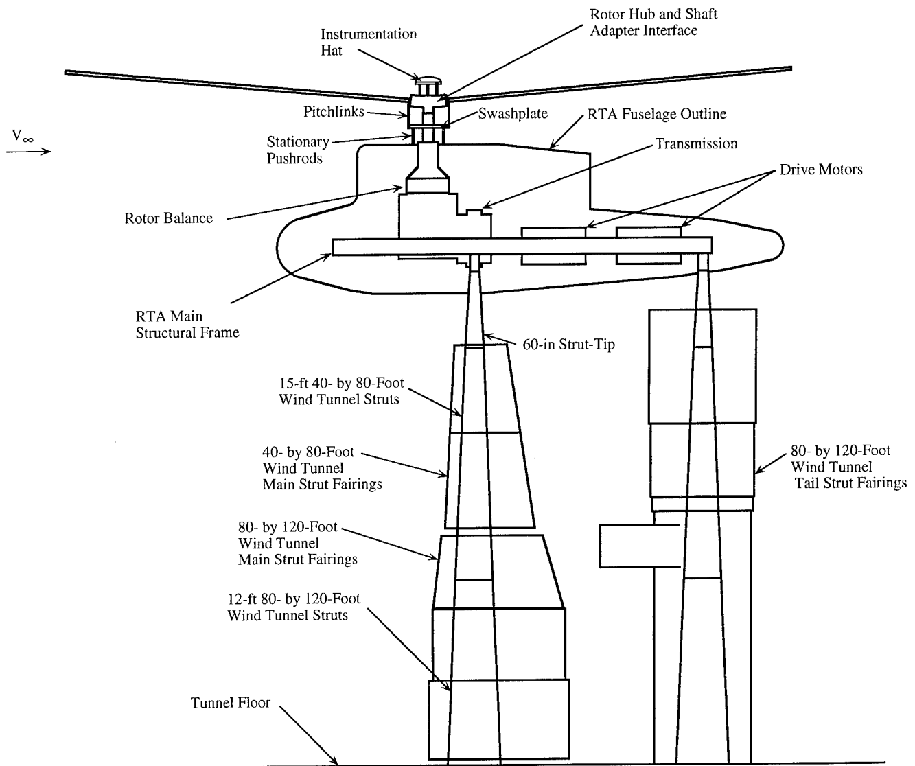
Figure 3a. Schematic of RTA/S-76 rotor test set-up in the 80- by 120-Foot Wind Tunnel.
