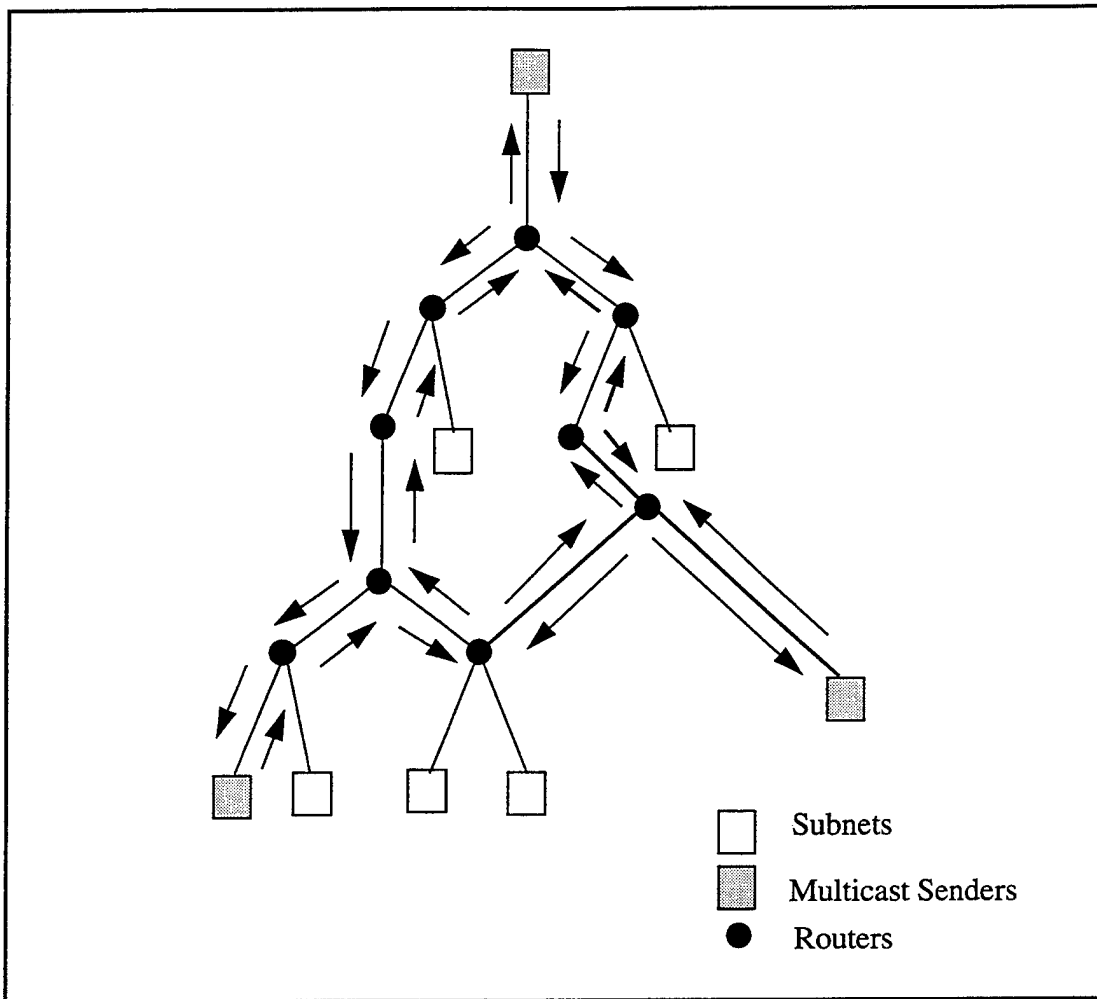
Figure 39. Source-based multicast trees.
