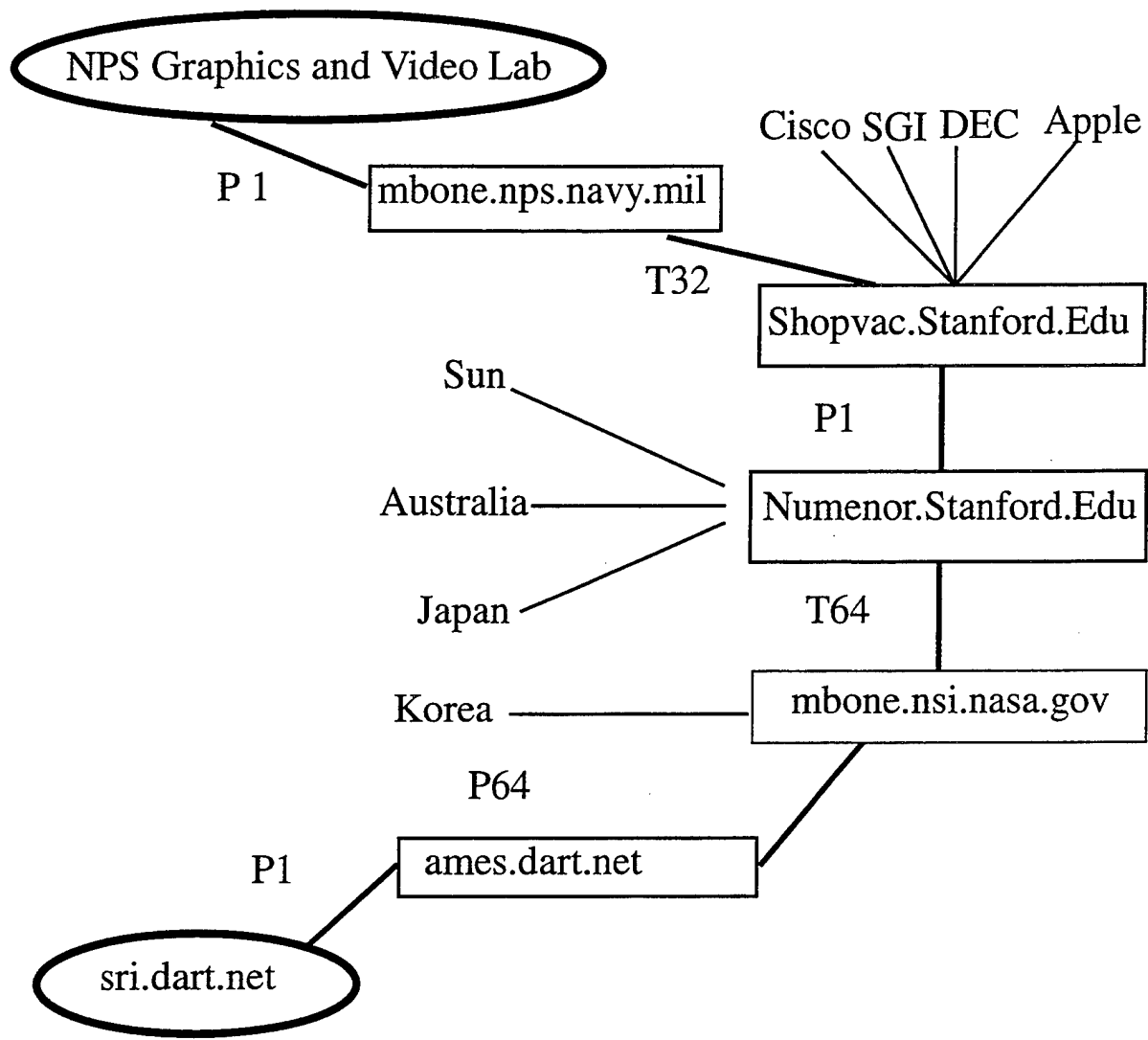
Figure 44. MBONE routing between NPS and SRI.
