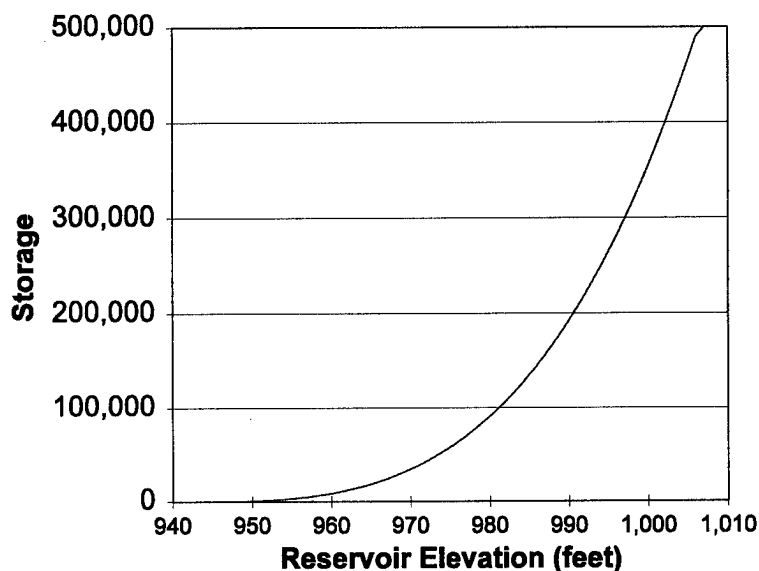
Figure B-1. - Storage Volume (Acre-Feet)
