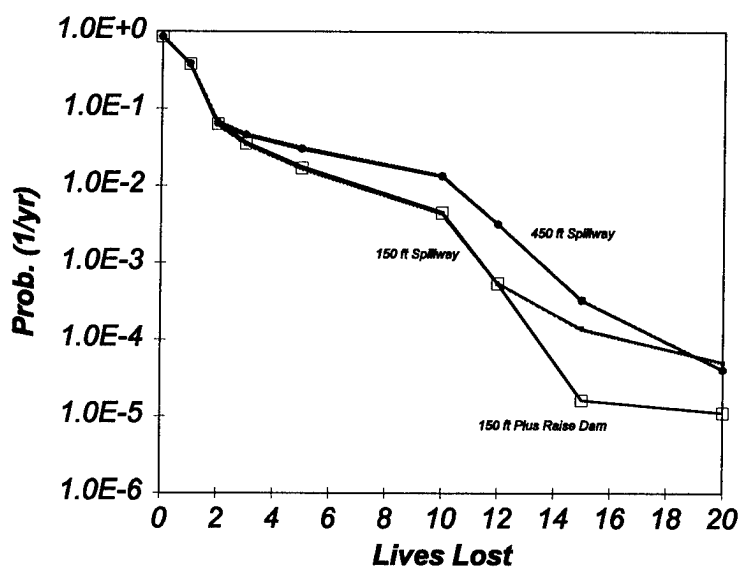
Figure 7b. - Distribution of Loss-of-Life As a Plot of the Exceedance Probabilities Thick-Tailed Rainfall Distribution
