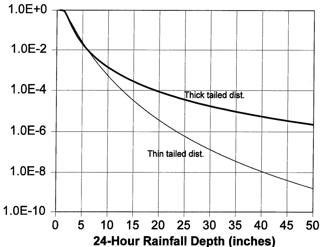
Figure 4. - Exceedance Probability for 24-Hour Rainfall Depth.
