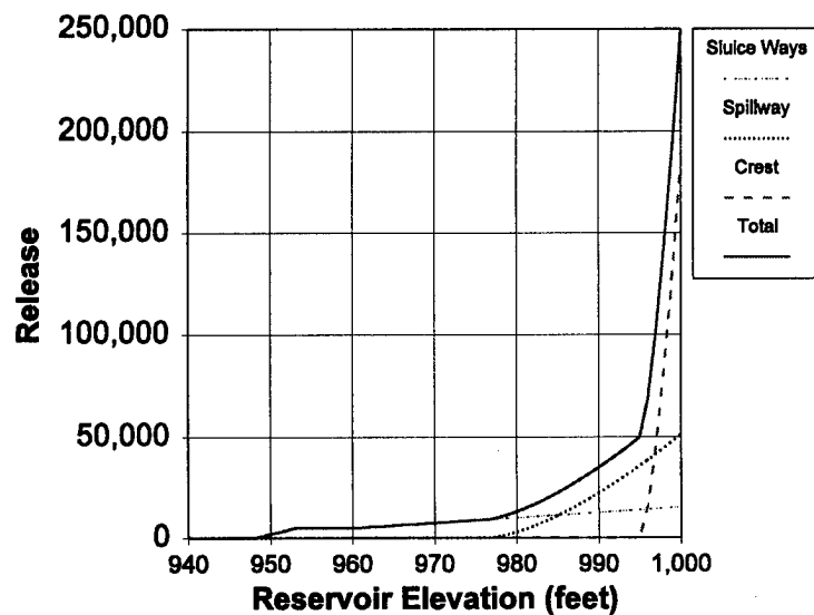
Figure B-2. - Reservoir Releases as Function of Elevation for 150-foot Spillway
