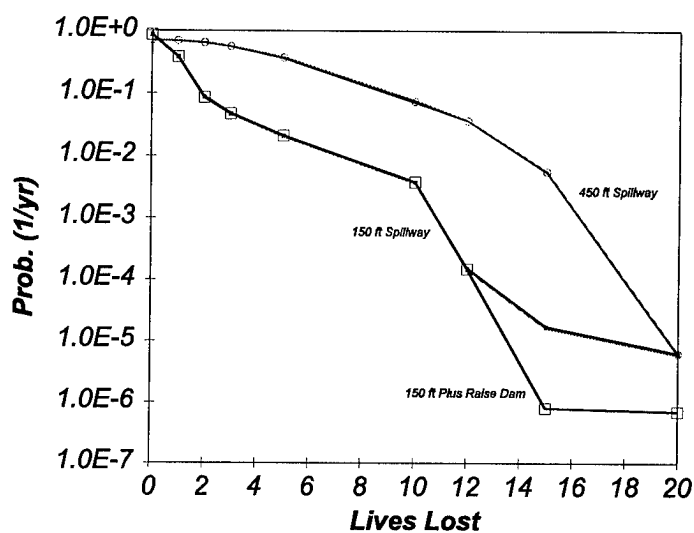
Figure 5b. - Distribution of Loss-of-Life As a Plot of the Exceedance Probabilities Thin-Tailed Rainfall Distribution
