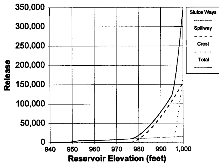
Figure B-3. - Reservoir Releases as Function of Elevation for 450-foot Spillway
