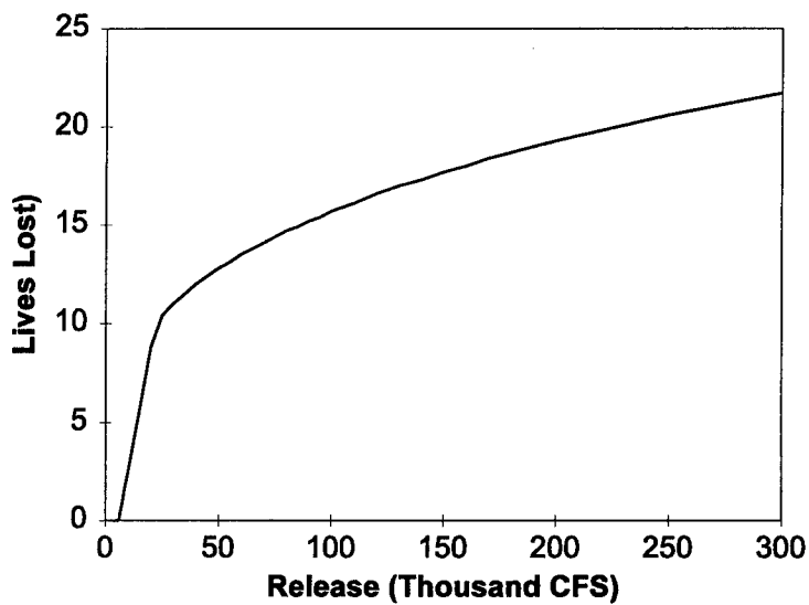
Figure B-5. - Lives Lost as Function of Release
