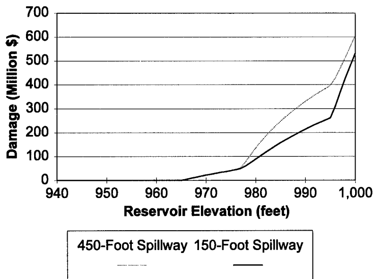
Figure B-6. - Dollar Damage in Million $
