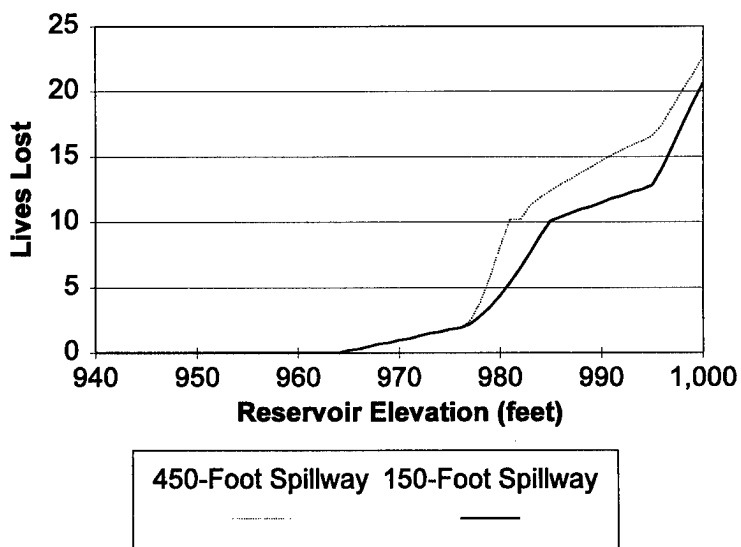
Figure B-7. - Loss-of-Life as Function of Elevation
