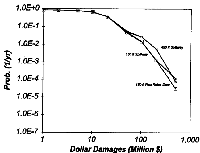
Figure 7a. - Distribution of Damage As a Plot of the Exceedance Probabilities Thick-Tailed Rainfall Distribution
