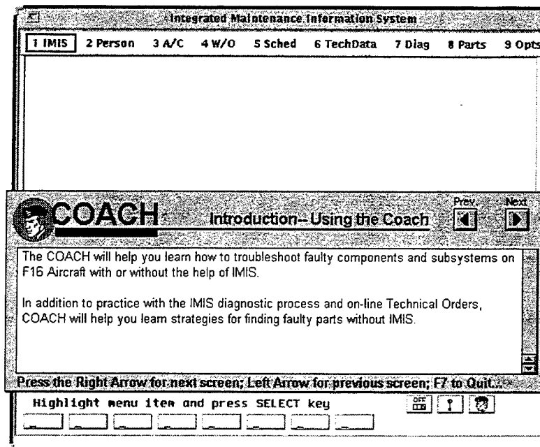
Fig. 7. Introduction screen 2.
