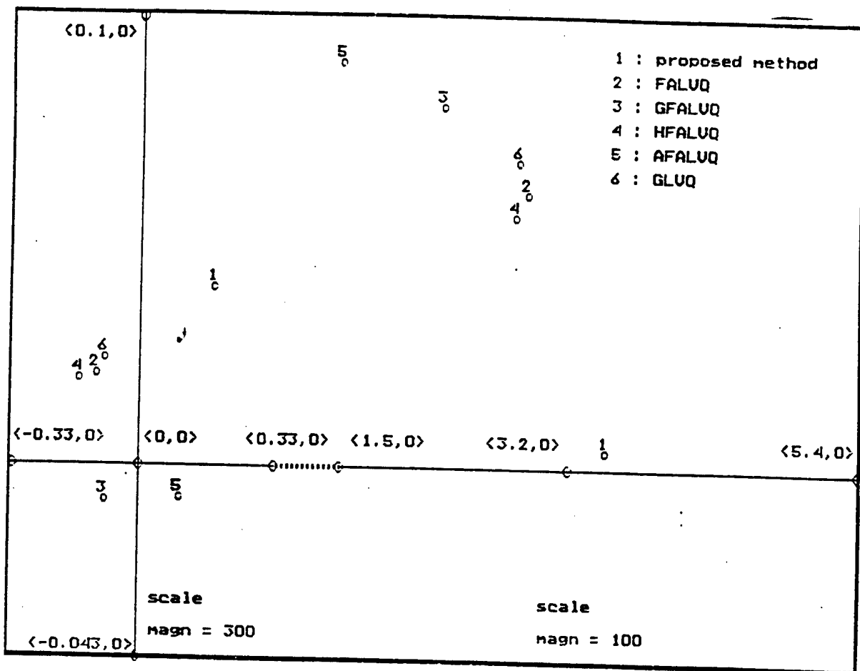
Fig. 25 : Cluster centers produced for artificial data set by different algorithms
