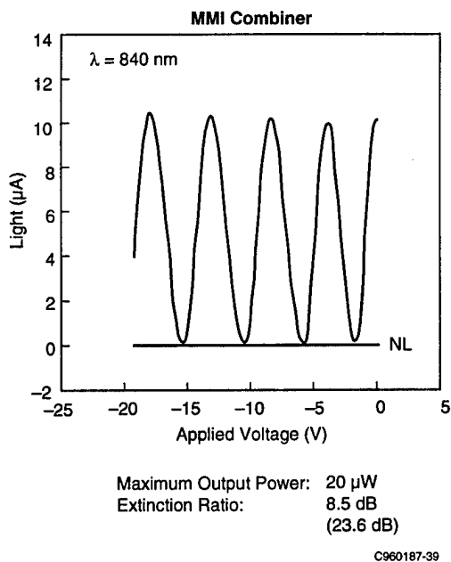
Figure 4-1b. Measured Mach-Zehnder DC Characteristics
