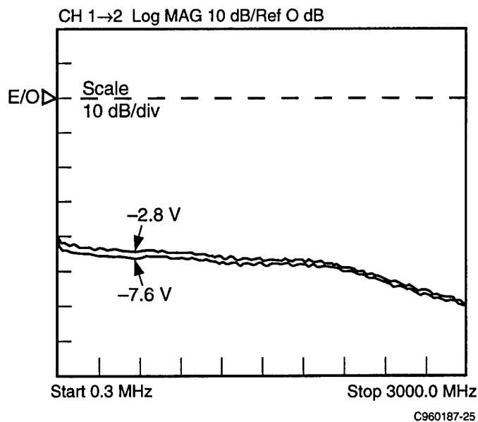
Figure 4-10. Measured E/O Response of the Modulator at a Bias of -2.8 V and -7.6 V
