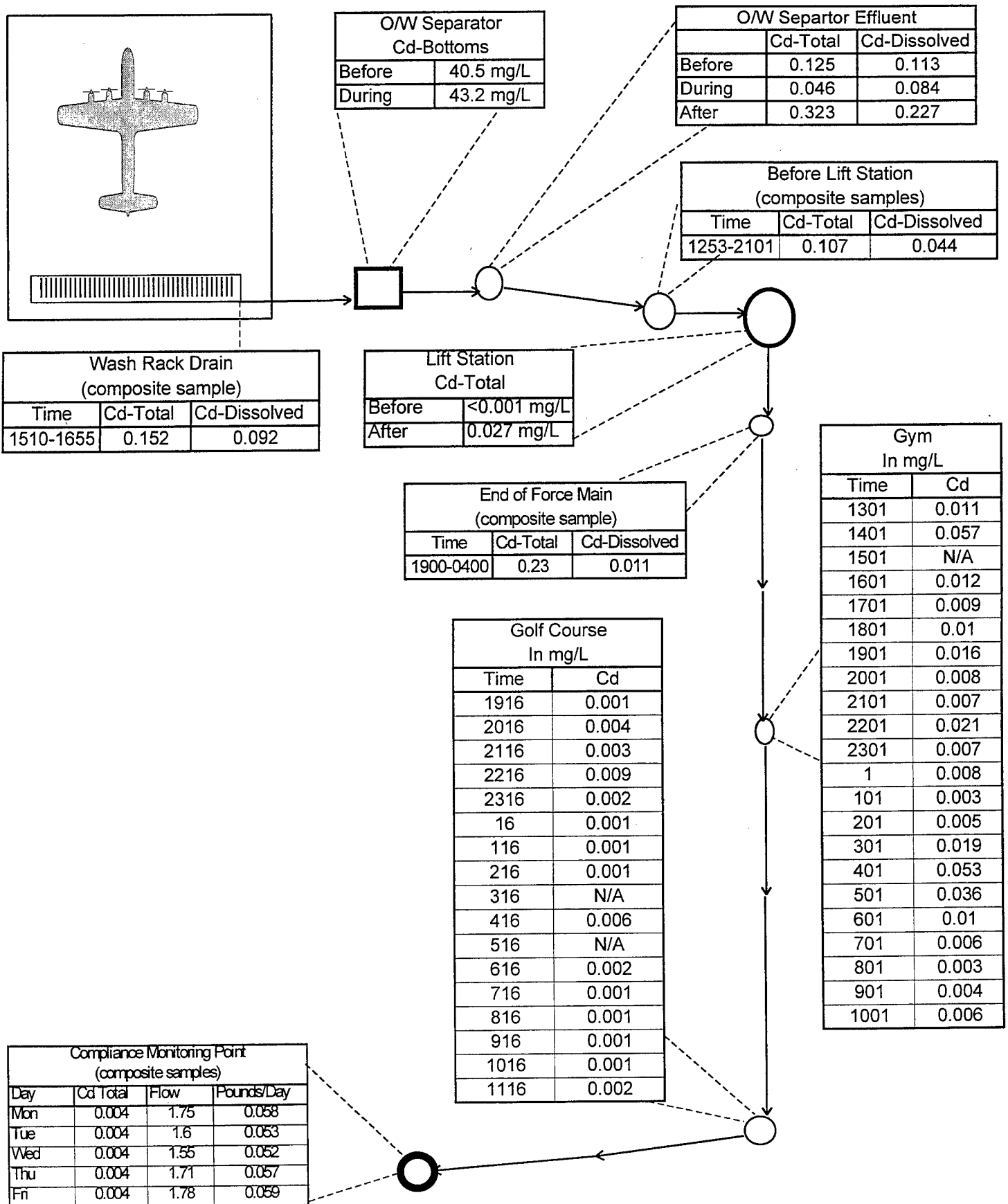
Figure 9: Compressor Wastewater Flow from Washrack Facility 228
