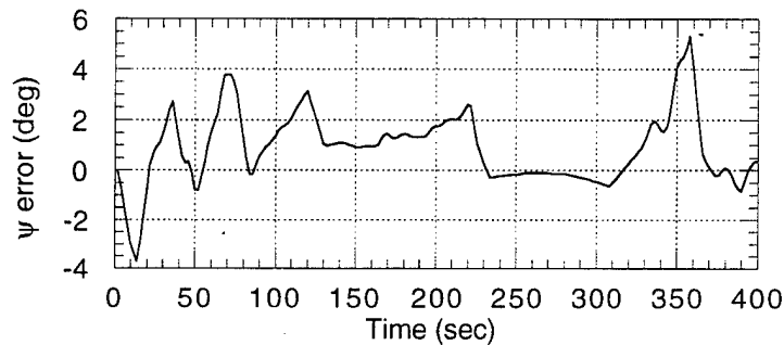
Figure 4.2-2: Heading Errors vs. Time during Hover
