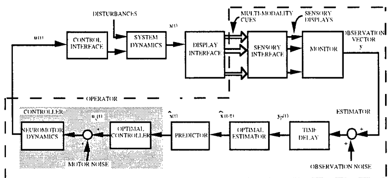
Figure 2.3-1: Optimal Control Model of Pilot/Vehicle System
