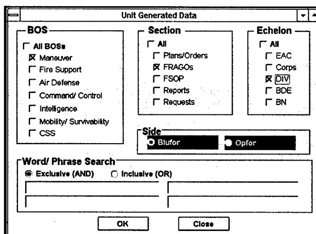
Figure 18 - Unit Generated Data
