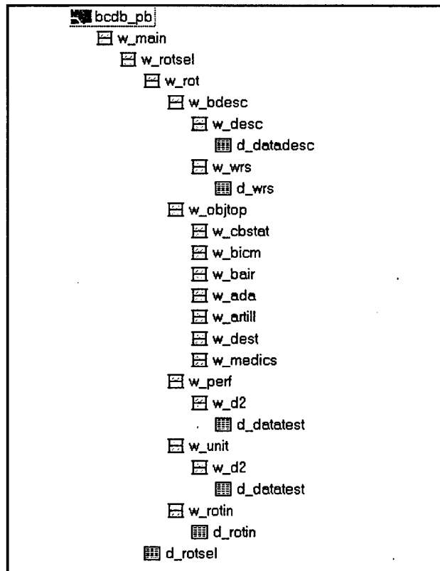
Figure 1 - BCTPdb Hierarchy
