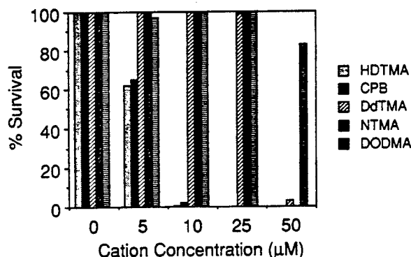
Figure 6. Relative toxicities of five quaternary ammonium compounds to P. putida assayed as the percent survival following a 1-h treatment at various cation concentrations.
