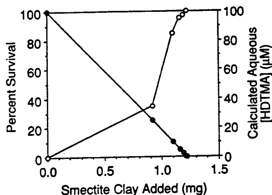
Figure 3. Influence of smectite clay additions on the survival of P. putida (open circles) in 100 μM HDTMA solutions (2 mL) following a 1-h treatment. The calculated equilibrium aqueous-phase HDTMA concentrations (solid circles) are shown on the right-hand ordinate.
