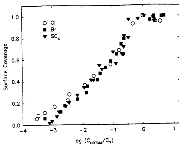
FIGURE 3. Normalized adsorption isotherms for HDTMA in Ca-Oshtemo B 1 soil (as shown in Figure 2a).
