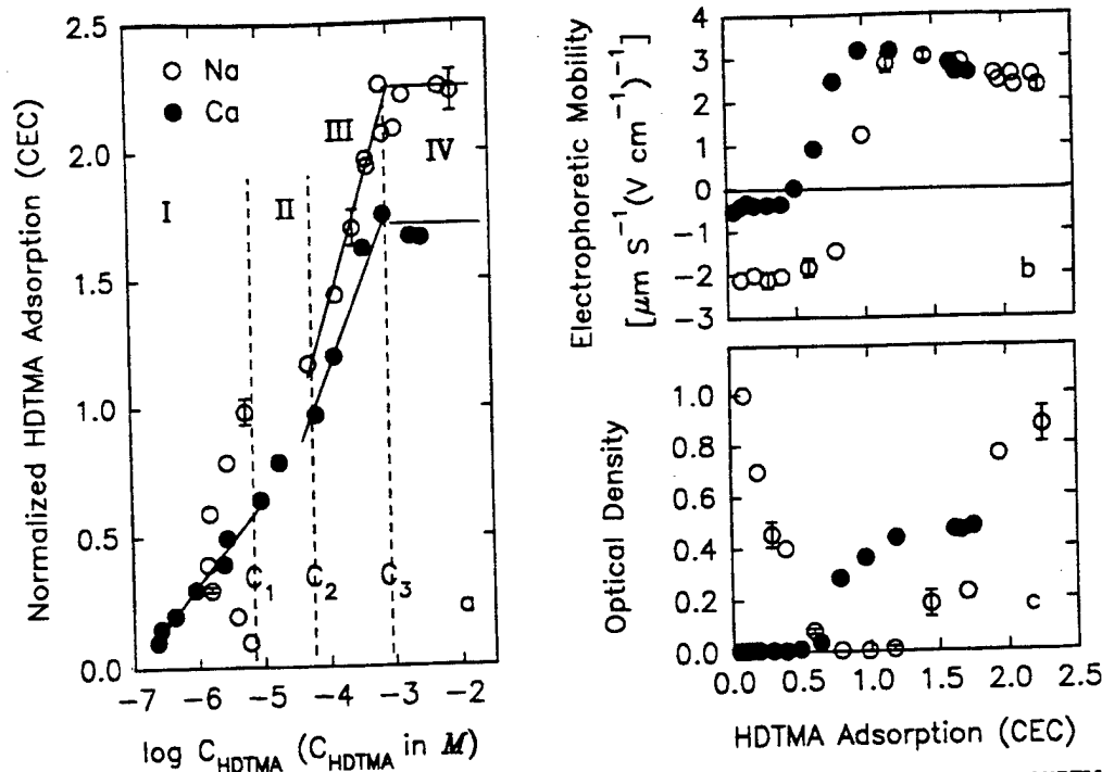
FIGURE 1. (a) Adsorption isotherms of HDTMA Cl in Na- and Ca-saturated Oshetemo B 1 ; (b) the electrophoretic mobility of HDTMA-soil clays; and (c) the relative turbidity of soil suspension as affected by HDTMA adsorption. The final electrolyte concentrations in all cases were 23 mM Cl - .
