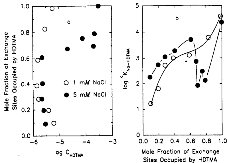
Fig. 2. (a) Sodium-hexadecyltrimethylammonium (HDTMA) exchange isotherms for Na-saturated Oshtemo B at two initial NaCl concentrations and (b) the dependence of cation selectivity coefficients ( K_{\text{Na-HDTMA}} ) on the HDTMA loading level.
