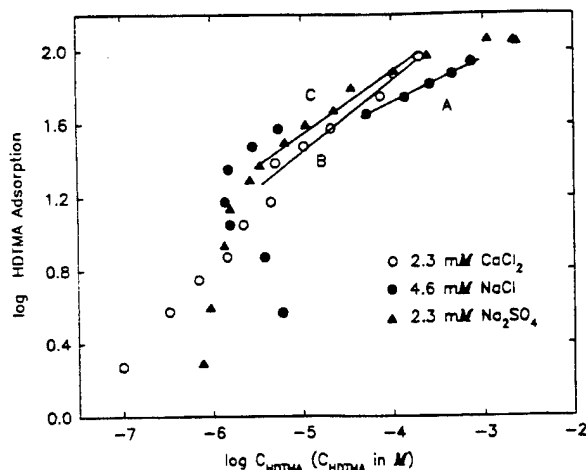
FIGURE 7. Illustration of simple linear relationship between logarithm of HDTMA adsorption and logarithm of HDTMA solution concentration at high HDTMA loadings (lines A, B, and C) in Oshitemo B 1 soil.
