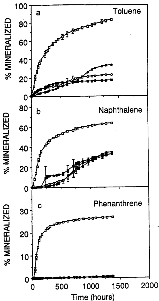
Figure 2. Time courses for the mineralization of toluene (a, 5 \mu\text{g mL}^{-1} ), naphthalene (b, 1 \mu\text{g mL}^{-1} ), and phenanthrene (c, 0.5 \mu\text{g mL}^{-1} ) in Eielson soil slurries treated with HDTMA at 0 (controls, open squares), 10% (open circles), 30% (solid squares) or 70% (solid circles) of the cation-exchange capacity.
