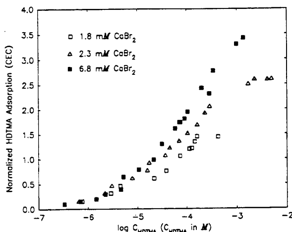
FIGURE 4. Influence of ionic strength on HDTMA adsorption in Ca-Oshtemo B 1 .
