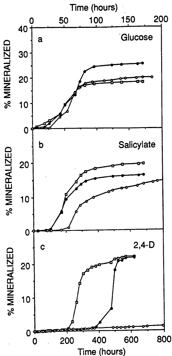
Figure 1. Time courses for the mineralization of glucose (a, 200 \mu\text{g mL}^{-1} ), salicylate (b, 5 \mu\text{g mL}^{-1} ), and 2,4-D (c, 10 \mu\text{g mL}^{-1} ) in Marlette A soil slurries (10 g soil, 50 mL of PBS) treated with HDTMA at 0 (controls, open squares), 30% (solid circles), or 70% (open circles) of the cation-exchange capacity. The upper time scale applies to panels a and b; the lower time scale applies to panel c.
