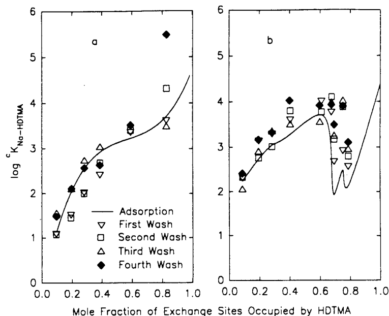
Fig. 4. (a) Comparison between cation selectivity coefficients of Na-hexadecyltrimethylammonium (HDTMA) exchange on Oshtemo B obtained from adsorption (Na-HDTMA) with (b) those from desorption (HDTMA-Na).
