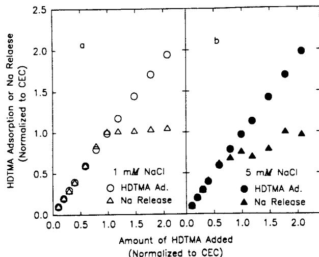
Fig. 1. Comparison of the amount of hexadecyltrimethylammonium (HDTMA) adsorbed to the amount of Na liberated in Na-saturated Oshemo B soil at two initial NaCl concentrations (a and b). All of the variables (HDTMA adsorption, Na release, and the amount of HDTMA added to soil suspension) are normalized to the soil CEC (38 mmol c kg -1 ).
