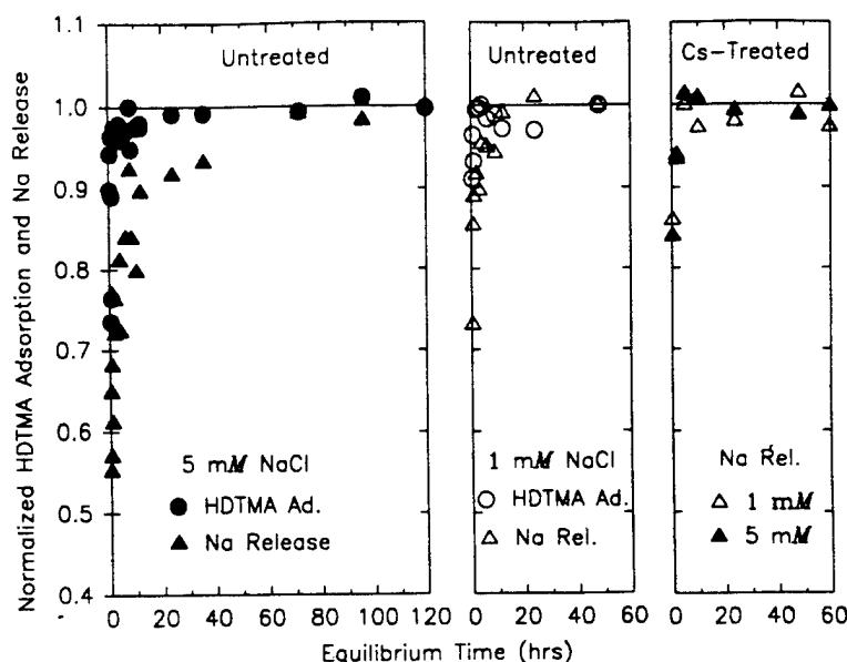
Fig. 6. Kinetics of hexadecyltrimethylammonium adsorption and Na release on Na-saturated untreated Oshtemo B soil and on Na-saturated Cs-treated Oshtemo B soil as affected by initial NaCl concentrations.
