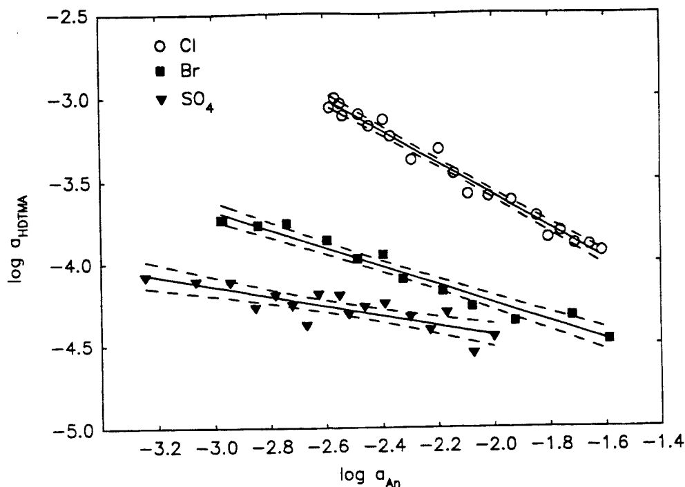
FIGURE 5. Influence of ionic strength on activity of residual HDTMA in NaCl, NaBr, and Na 2 SO 4 solutions after a fixed amount of HDTMA (2 equiv of the soil CEC) was added to Na-Oshtemo B 1 soil suspension. Dashed lines indicate the 95% confidence intervals.
