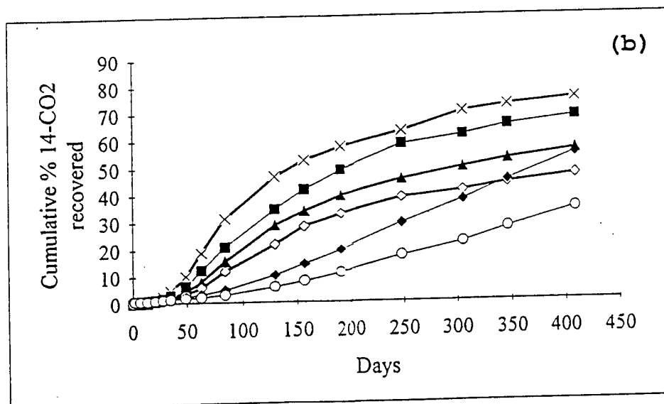
Figure 5. a. Biostability of DODMA added as a free cation in Marlette A (x,▲,+) and B (●,◇,■) soils. DODMA added as the equivalent amount bound to 100 mg of smectite clay and exchanged at 30 % (x;●), 70 % (▲;◇) or 100 % (+;■) of the CEC of the clay. b. Biostability of DODMA added as a free cation in Spinks A (x,▲,◇) and Spinks B (◆,■,o) soils. DODMA was added as an equivalent amount bound to 100 mg of smectite clay and exchanged at 30 % (x;■), 70 % (▲;◆) or 100 % (◇;o) of the CEC of the clay.
