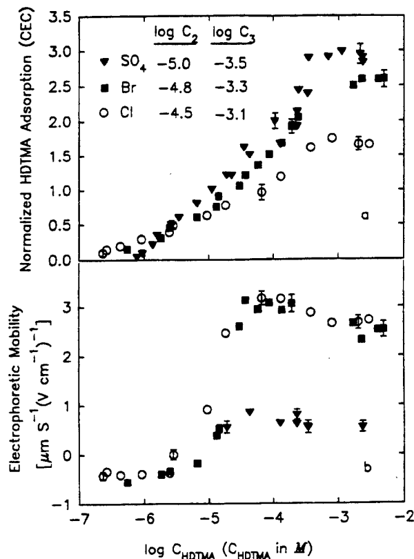
FIGURE 2. (a) Adsorption isotherms of HDTMA in Ca-saturated Oshemo B 1 soil and (b) electrophoretic mobility of HDTMA-soil clay as affected by different companion anions.
