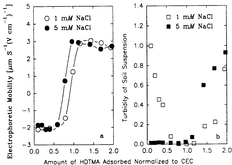
Fig. 5. (a) Electrophoretic mobility of soil clay in Oshtemo B soil and (b) turbidity of soil suspension as affected by hexadecyltrimethylammonium loading.
