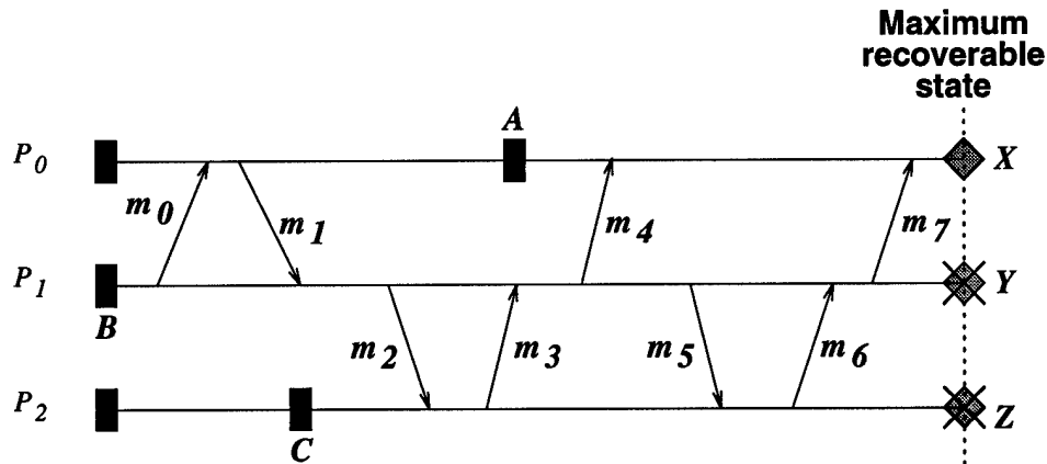
Figure 11: Pessimistic logging.
