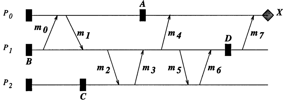
Figure 12: Optimistic logging.
