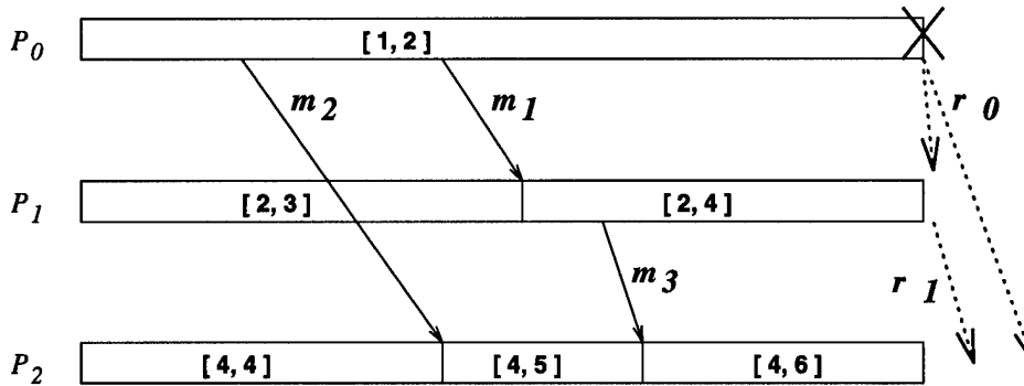
Figure 13: Exponential rollbacks.
