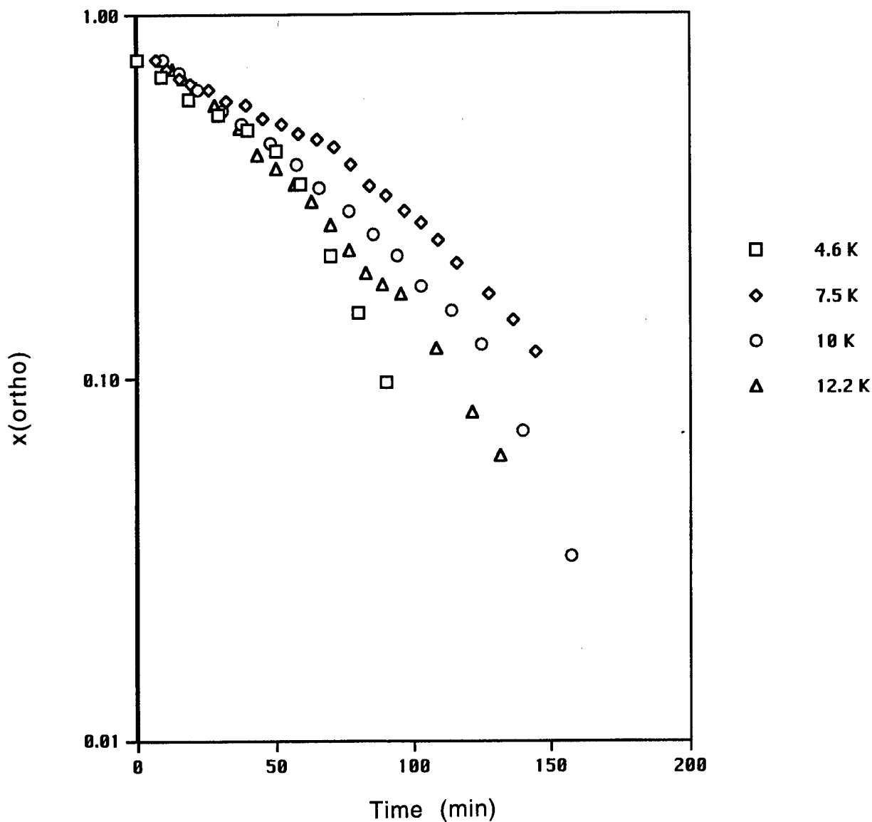
Figure 12 Ortho H_2 Concentration versus Time
