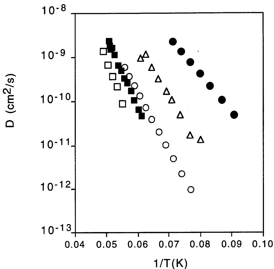
Figure 2 D versus the Reciprocal Sensor Temperature, T^{-1} The plot symbols are: T_2 [M□], D-T [■], D_2 [○], HD [△], and H_2 [v].
