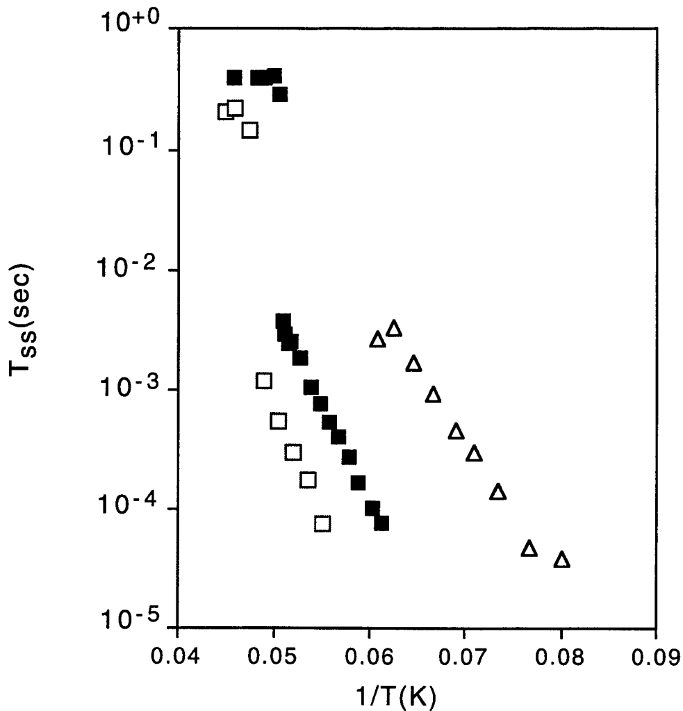
Figure 1 T_{ss} Versus the Reciprocal Sensor Temperature, T^{-1} The plot symbols are: for HD [Δ]; D-T [■□]; and T_2 [M□].
