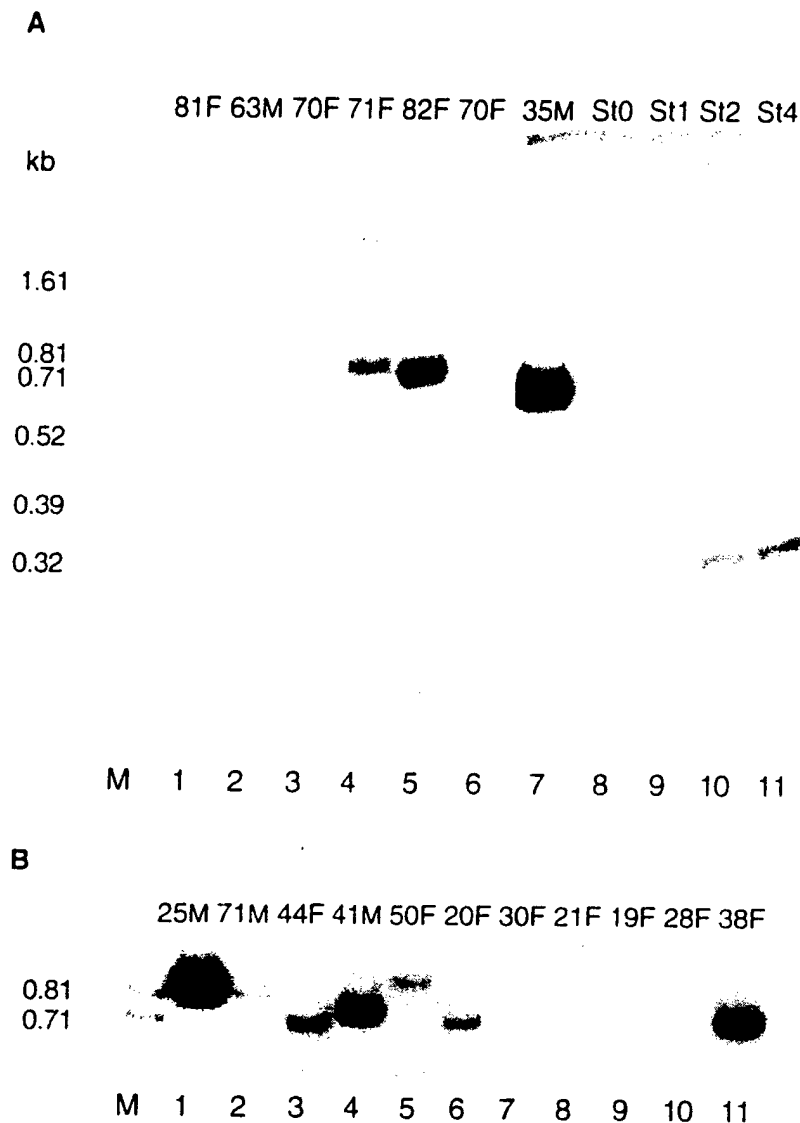
FIG. 2 Characterization of bcl-2/J H translocation-derived PCR products from Blood samples. Fourteen of 7 \mu g of PBM DNA from 18 individuals were amplified, and the PCR products were electrophoresed on a 6% polyacrylamide gel and visualized by autoradiography. The age and sex of each blood donor is indicated. A, Lanes 4, 5, and 7, and B, Lanes 1-6, and 11, translocation-positive ( bcl-2/J H + ) PBM samples. A, Lanes 1-3 and 6, and B, Lanes 7-10, translocation negative PBM samples. A, Lanes 9-11 (St1, St2, and St4), aliquots of a bcl-2/J H + standard, SU-DHL-4 DNA, that should contain an average of 1, 2, or 4 molecules of the bcl-2/J H translocation; Lane 8 (St0), 14 \mu g of human brain DNA alone, as a negative control, subjected to PBM samples. The amplification experiment in A and that in B were done with different batches of 32 P-labeled primer; therefore, they are not comparable. M, molecular weight DNA markers.
