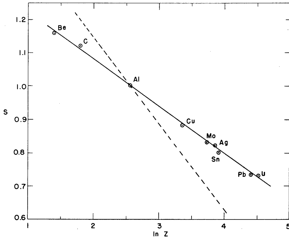
Figure 2. Experimental relation between the average relative stopping power per electron, S, averaged over the energy range 0-200 Mev and relative to Al = 1, and the atomic number, Z, of the absorber. The dotted line indicates the results obtained by R. R. Wilson at 2-4 Mev and adjusted to Al = 1.
