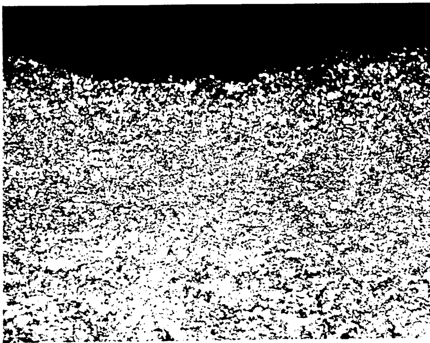
Figure 45. 92CPC0801, Procedure #4. Etched with Keller's Reagent, 15 Seconds. 500X.
