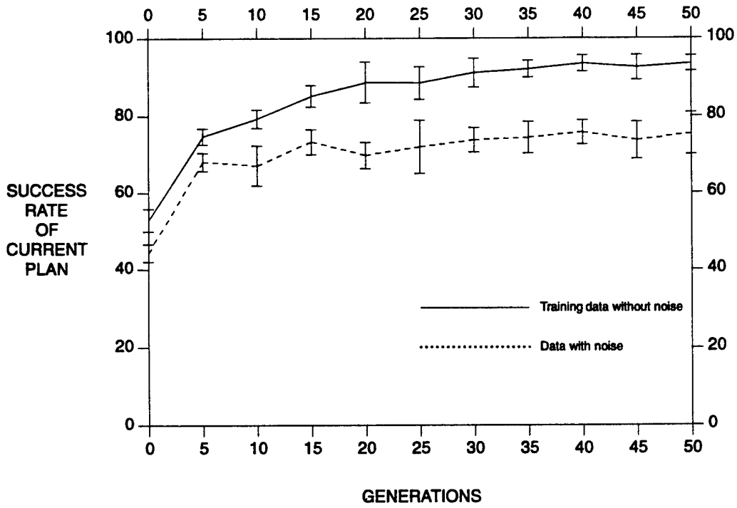
Fig. 5 - Comparison plot for EVADE problem when SAMUEL uses its default rule-matching mechanism
