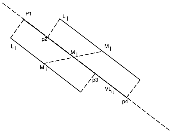
Figure 11: Line grouping
