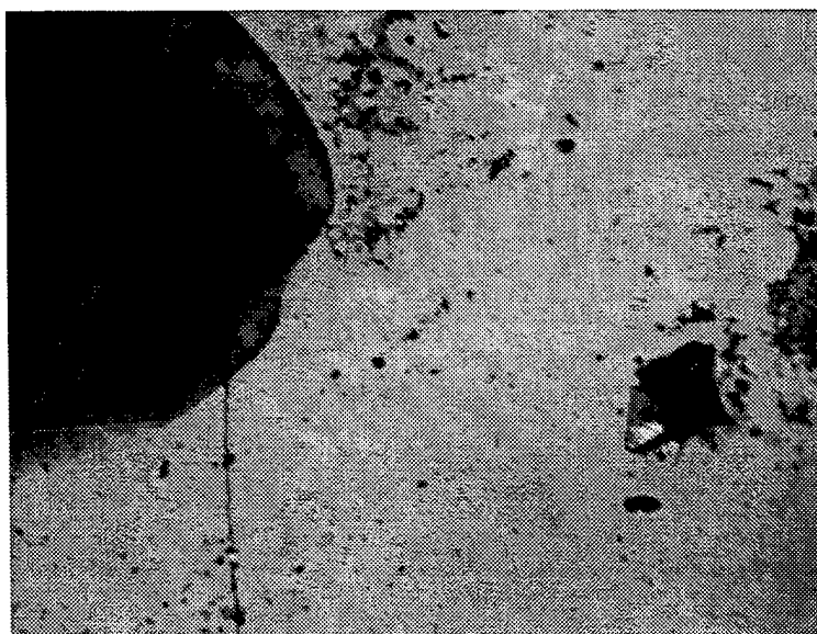
Figure 18. Crack extension from an intrinsic flaw (on the left) was obtained on a quenched bearing ball rather than from the large Vicker's indent flaw on the right. The dark carbonized area is an artifact from the charring of peanut oil.
