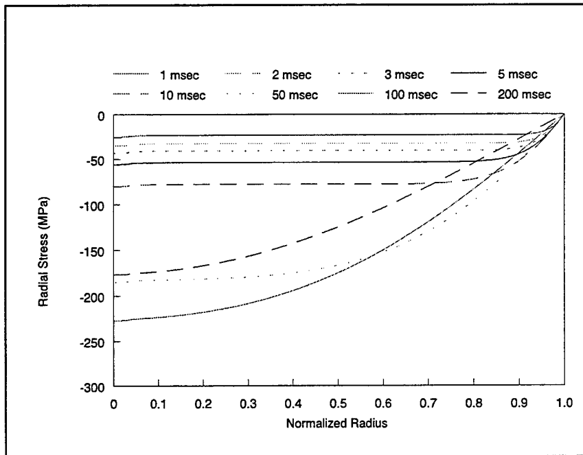
Figure 12. Closed form solution of the radial stress profile of a 11.11 mm diameter ball from a thermal quench temperature \Delta T of 666^{\circ}\text{C} .
