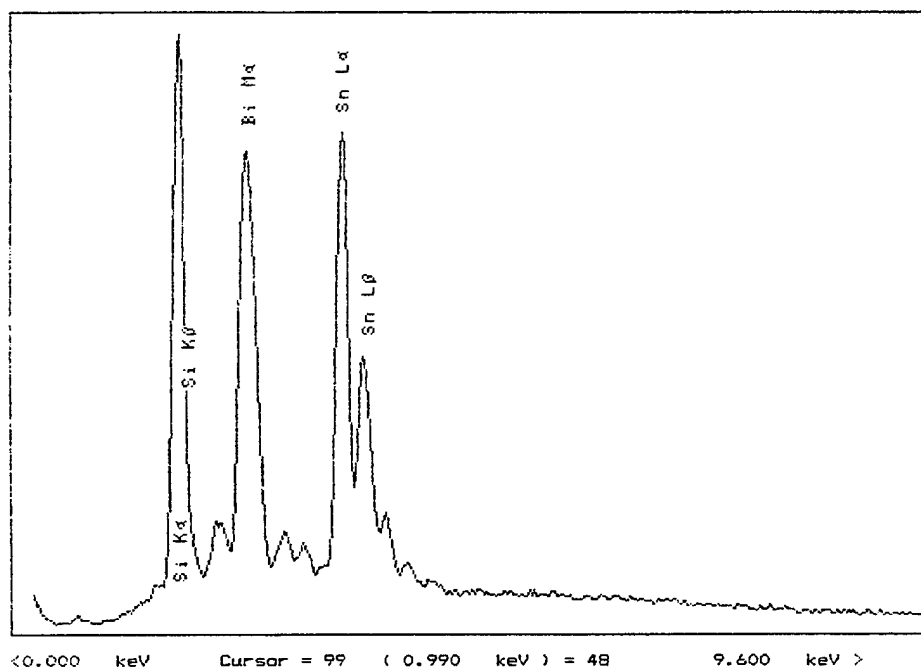
Figure 27. EDS spectrum of Figure 26 which indicates the presence of bismuth-tin at this 2 mm depth.
