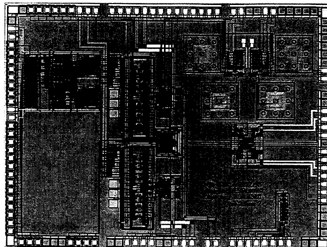
Fig. 8. Transmitter IC microphotograph
