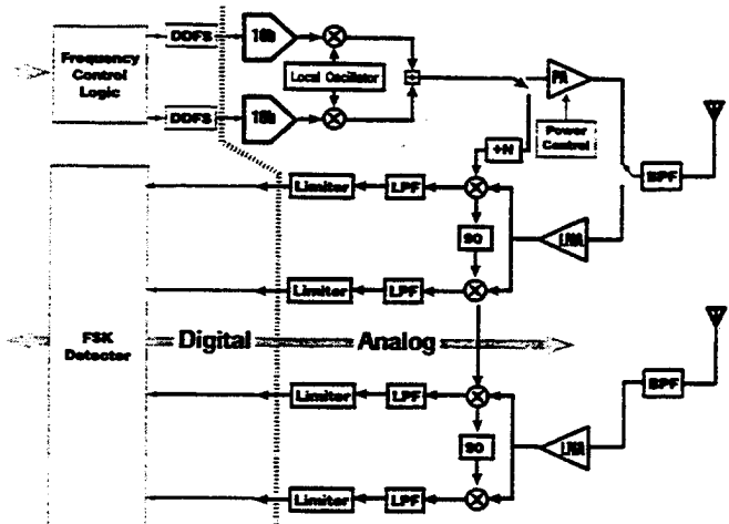
Fig. 5. Architecture of the UCLA Frequency-Hopped FSK Transceiver. Two entire receive channels connected to the antennas help to combat multipath fading with spatial diversity.
