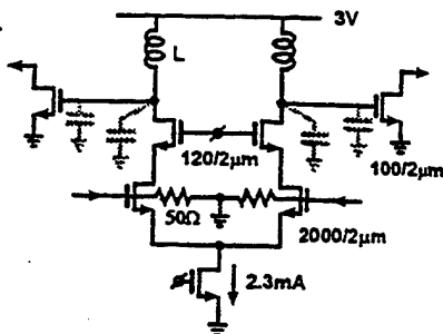
Fig.3. Circuit diagram of monolithic RF amplifier. Open drain output MOSFETs are biased off-chip.
