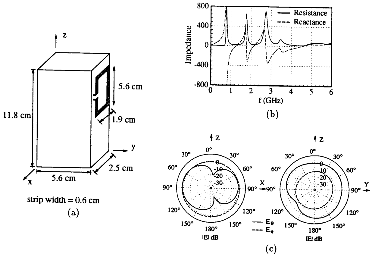
Figure 7: FDTD analysis of a strip loop on a hand-held transceiver: (a) transceiver geometry; (b) input impedance versus frequency; (c) directivity patterns at f = 915 MHz.
