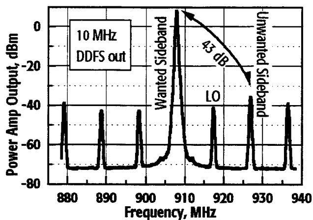
Fig. 9 Measured output spectrum from power amplifier, with single 10 MHz tone generated by DDFS.
