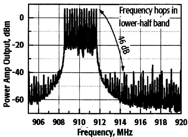
Fig. 10 Measured output spectrum from power amplifier, with DDFS hopping over 14 frequency slots in lower half of 902-928 MHz band.
