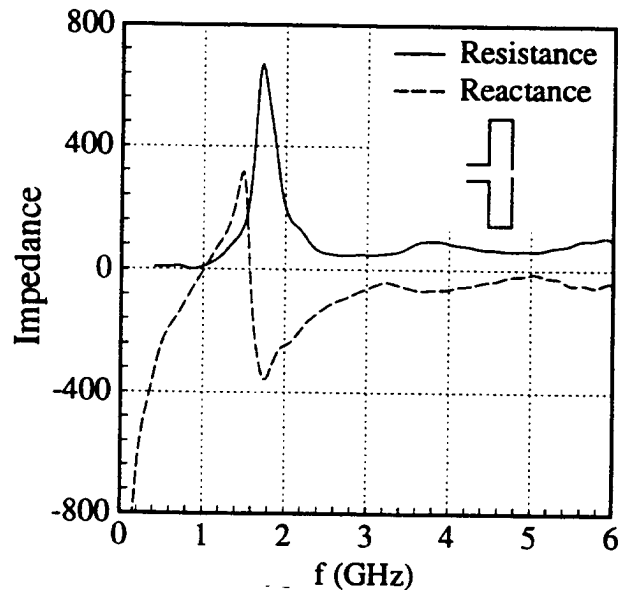
Figure 8: FDTD result of the input impedance versus frequency for a rectangular loop with a = 0.86 cm, b = 2.56 cm, and r_w = 0.75 mm loaded with an open circuit.
