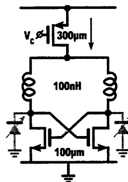
Figure 12: Tuning method
