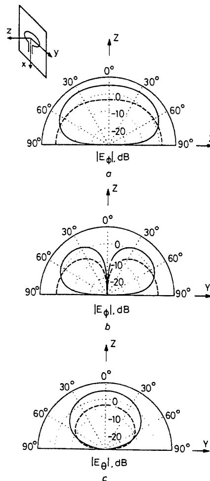
Fig. 8 Directivity pattern for 0.25\lambda elliptical loop of aspect ratio b/a = 2 both isolated and located 0.1\lambda from infinite ground plane
