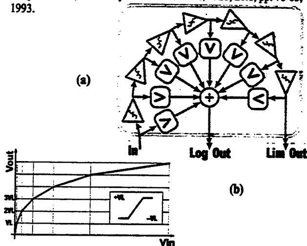
Fig. 1. (a) Principle of successive-detection logarithmic amplifier. Yields both logarithmic and limited outputs. (b) Piecewise-linear approximation to log function. VL is clipping-level of each amplifier.
