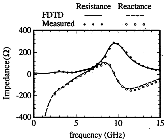
Fig. 4. Computed and measured input impedance versus frequency for the monopole on the handset illustrated in Fig. 1(b) for the parameters a = 1 cm, b = 2 cm, c = 3 cm, h = 1.25 cm, and \alpha = 1 cm. These small dimensions result from frequency scaling the handset to operate at 6 GHz.
