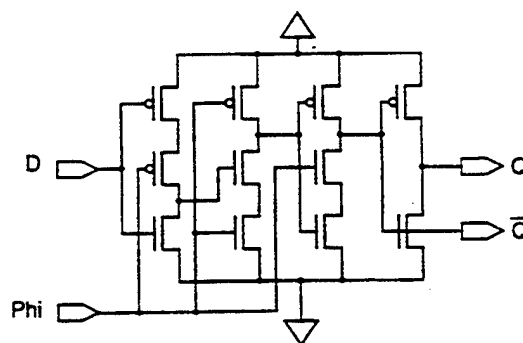
Fig. 2. Single-phase positive-edge triggered register.
