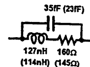
Fig.2. Equivalent circuit of suspended inductor. Measured parameter values are compared with values obtained from 3D simulations (in parentheses).
