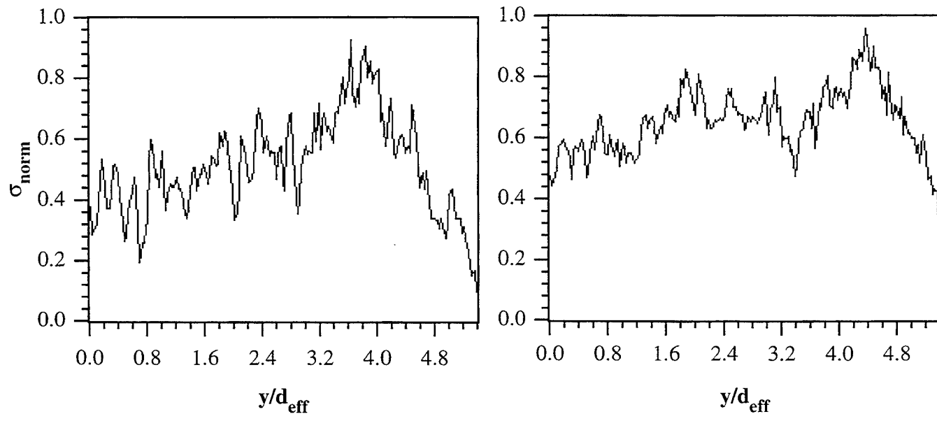
c) x/d_{\text{eff}} = 8, z/d_{\text{eff}} = 0
