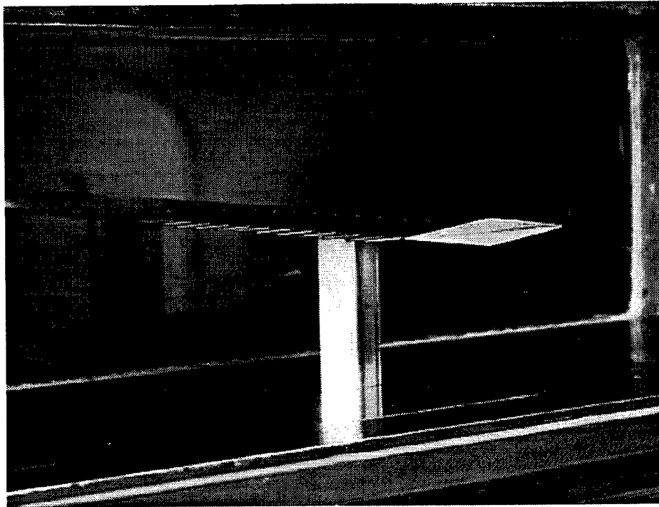
Figure 3.11 Photograph of Pitot Pressure Rake
