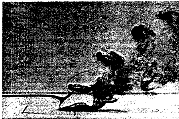
Figure 2.4 Dye Injection Visualization of Low Speed Jet in Crossflow Showing Shear Layer Vortices ( J = 4.8 ) [from Perry, et al. 52 ]
