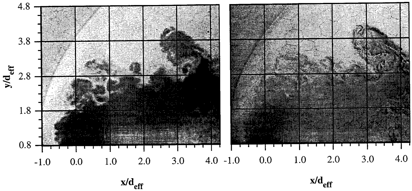
Figure 5.95 Instantaneous Double-Pulsed Image Pair from Circular Injection Using Air (Case C1A) with Laser Pulse Delay of \Delta t = 2 \mu\text{s}
