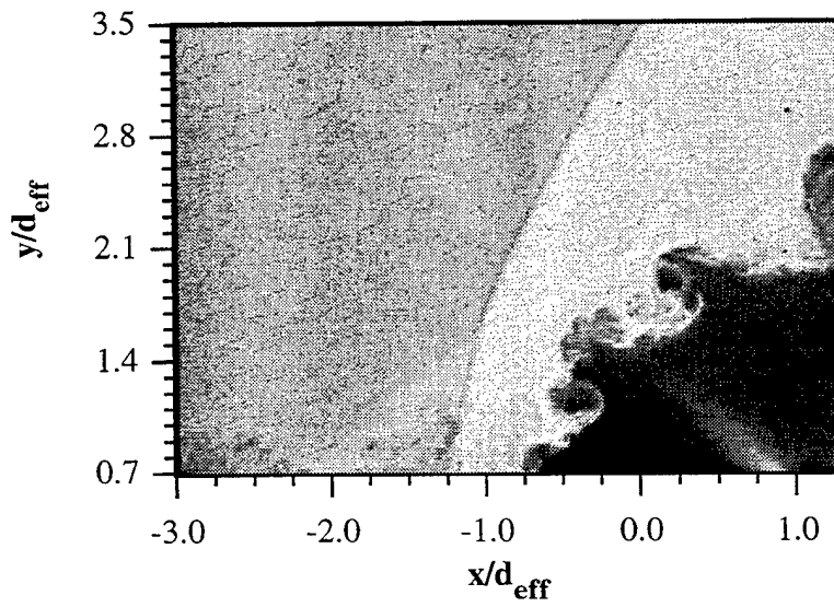
Figure 5.87 Instantaneous Images of Bow Shock/Jet Boundary Interaction Upstream of Elliptical Injector Using Air (Case E1A)
