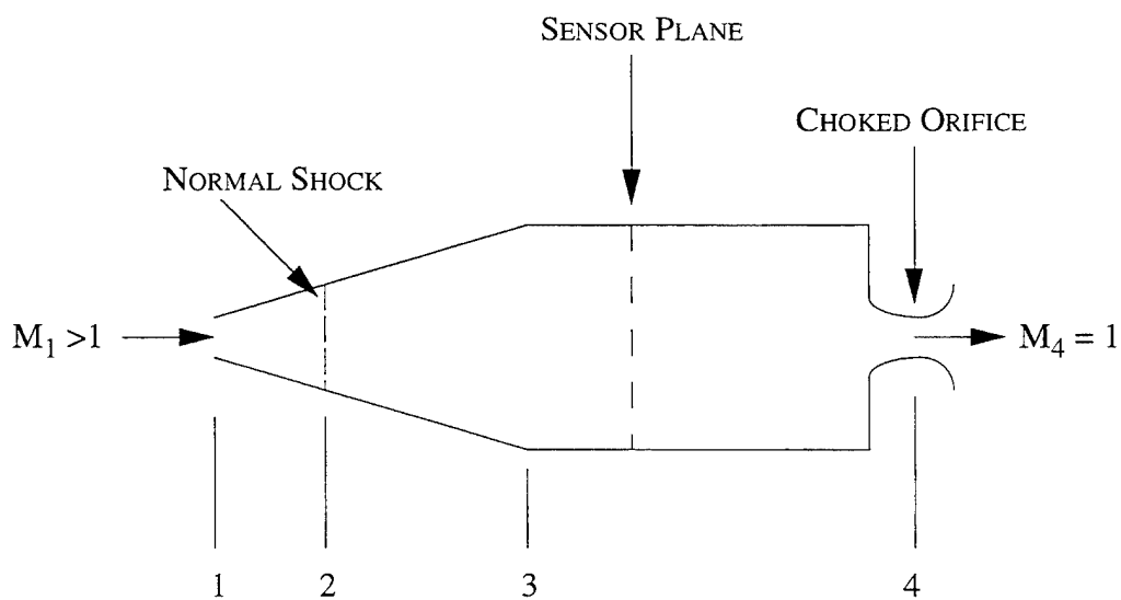
Figure 4.16 Model of Concentration Probe
