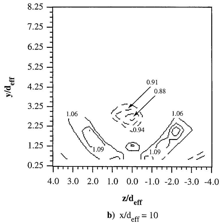
Figure 5.110 Contour Plots Showing Measured Pitot Pressure Ratio \Pi_{ce} a) x/d_{\text{eff}} = 4 and b) x/d_{\text{eff}} = 10
