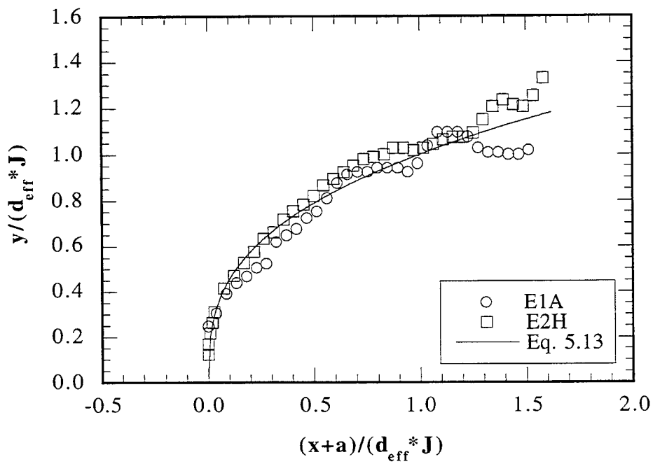
b) Elliptical Injection
