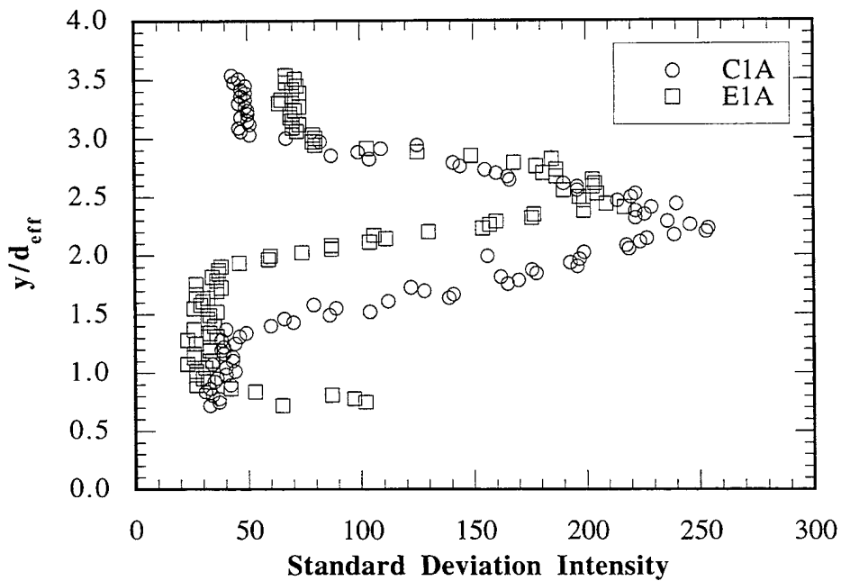
Figure 5.93 Intensity Profiles from Standard Deviation Bow Shock/Jet Boundary Interaction Images of Cases C1A and E1A at x/d_{eff} = 0
