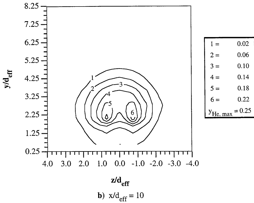
Figure 5.113 Helium Mass Fraction Contours from Circular Injection Using Helium (Case C2H) a) x/d_{\text{eff}} = 4 and b) x/d_{\text{eff}} = 10
