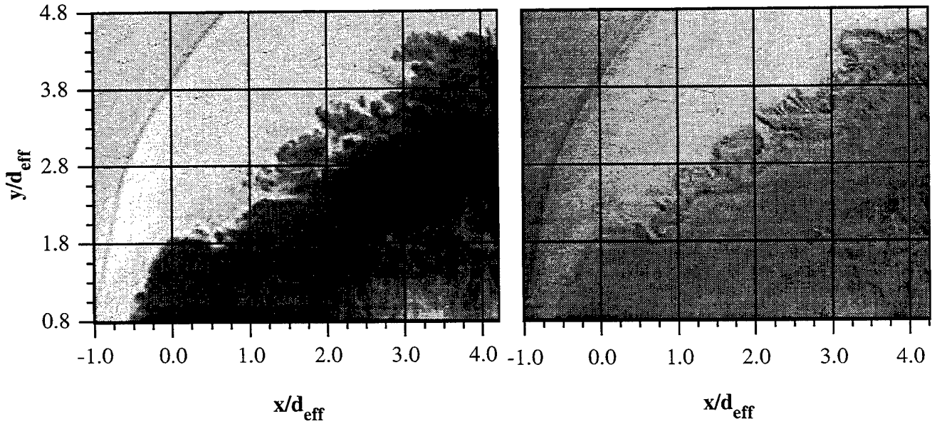
Figure 5.96 Instantaneous Double-Pulsed Image Pair from Circular Injection Using Helium (Case C2H) with Laser Pulse Delay of \Delta t = 1 \mu\text{s}
