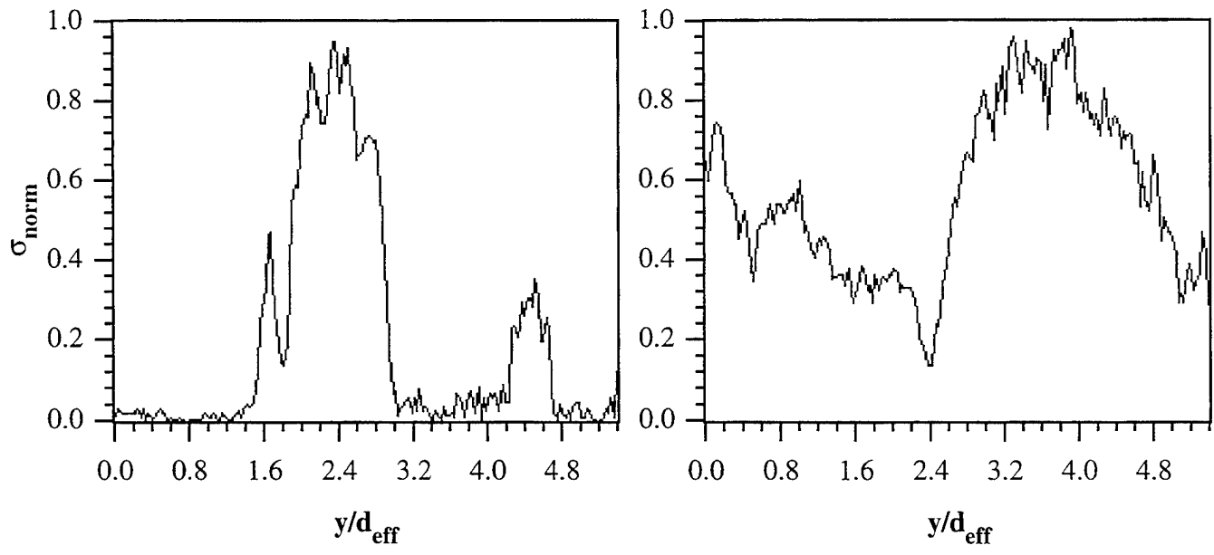
a) x/d_{\text{eff}} = 0, z/d_{\text{eff}} = 0
