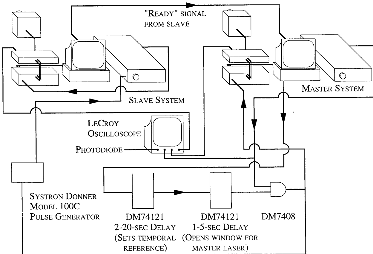
Figure 4.10 Delay System Electrical Schematic
