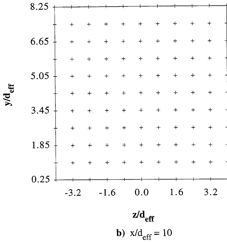
Figure 5.107 Measurement Locations for Probe-Based Studies a) x/d_{\text{eff}} = 4 and b) x/d_{\text{eff}} = 10
