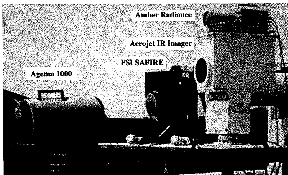
Figure 1-2. Sensor Array Used During July 1995 Field Test
