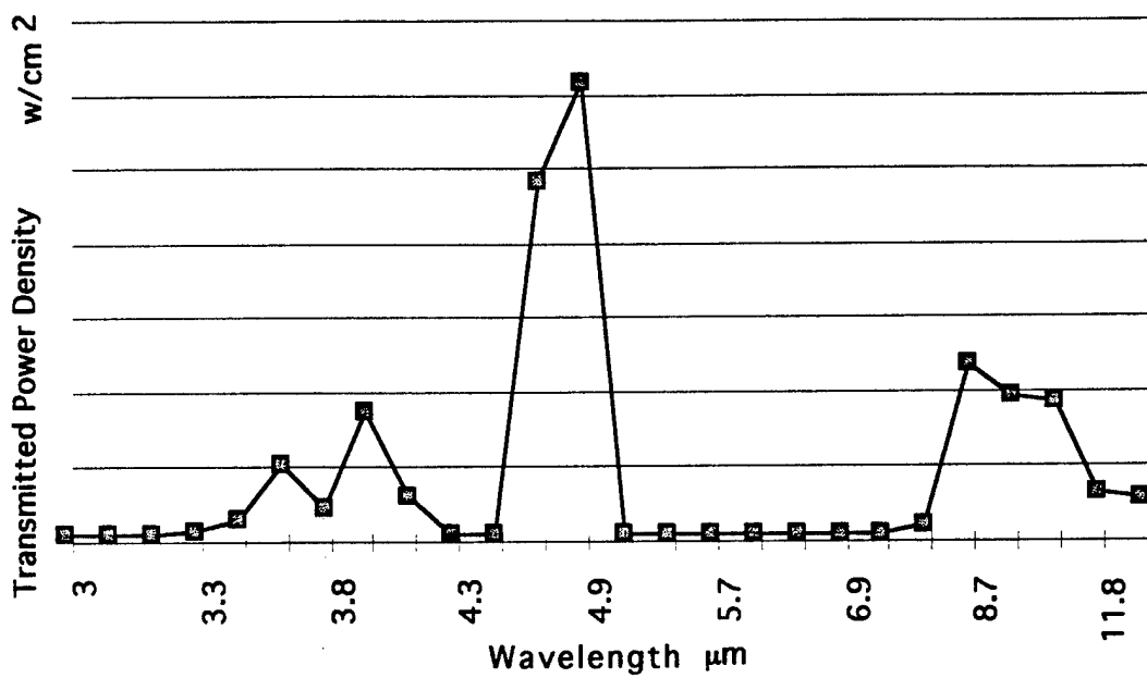
Figure A-5. Transmitted Power Density versus Wavelength (Range = 12 km, RH = 76%)
