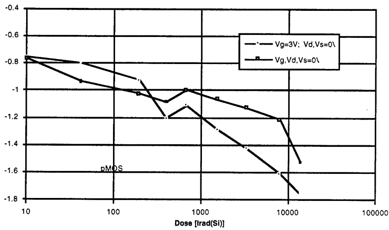
Figure 8: Variation of p-channel device threshold voltage (volts) with dose
