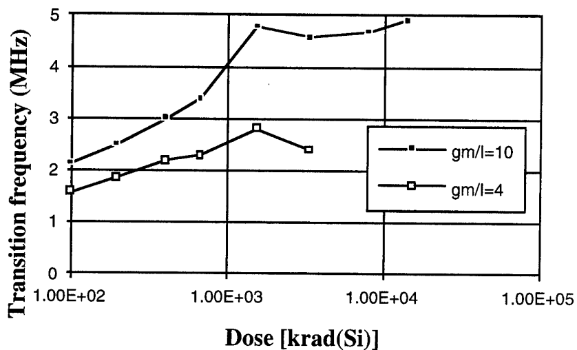
Figure 12: Variation of the transition frequency with dose
