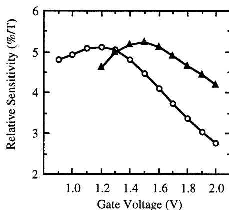
Figure 3. Relative Sensitivity as a function of the Gate Voltage for SOI ( \circ ) and bulk ( \blacktriangle ) split-drain devices. V_D = 3V , V_{TSOI} = 0.85V , V_{TBULK} = 1V .
