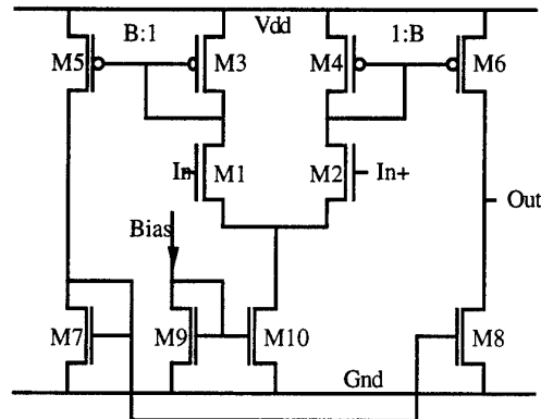
Figure 5: Operational Transconductance Amplifier
