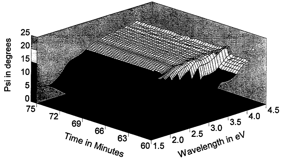
Figure 4.13. 3D plot of insitu SE data during HgCdTe growth initiation.
