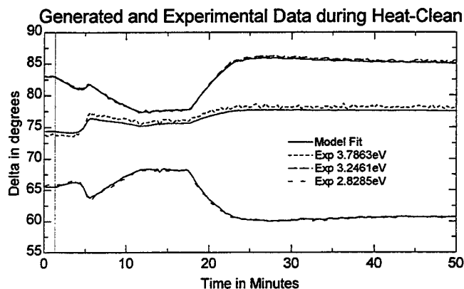
Figure 6.4. SE data fit vs. time during the substrate heat-clean procedure.
