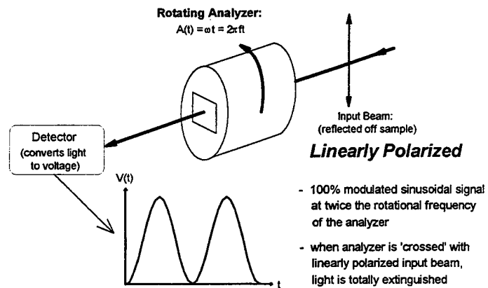
Figure 3.1. Detector signal for a linearly polarized beam entering the rotating analyzer polarization detector.
