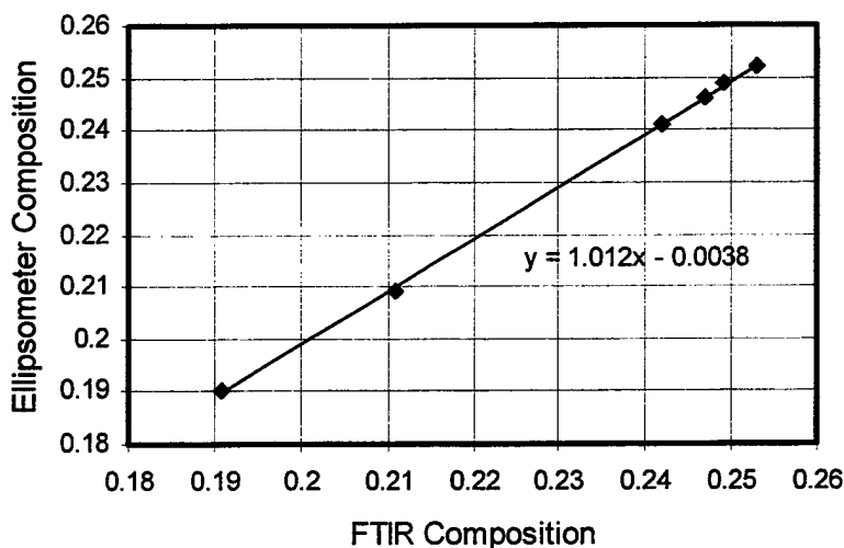
Figure 6.42. Correlation between ellipsometer and FTIR compositions, using best fit model which included surface roughness and the final MCT optical constant library.
