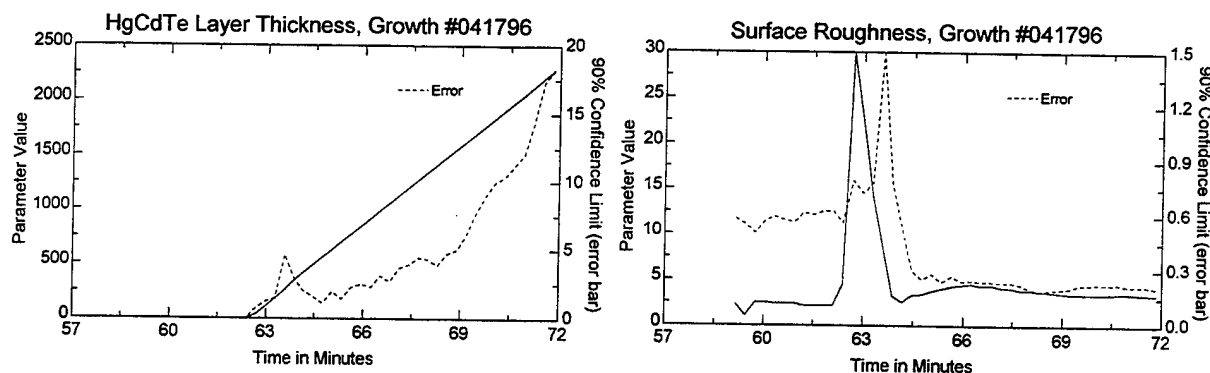
Figure 6.25. Parameters from Point-by-Point fit of HgCdTe growth #041796 with surface roughness model.
