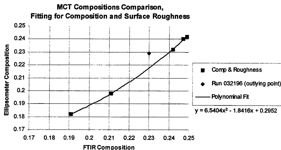
Figure 6.36. Correlation between ellipsometer and FTIR compositions for the best fit model.
