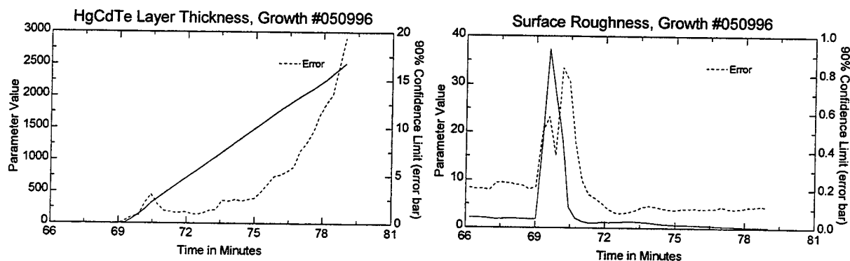
Figure 6.26. Parameters from Point-by-Point fit of HgCdTe growth #050996 with surface roughness model.
