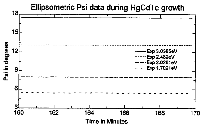
Figure 4.9. Real-time insitu ellipsometric Psi data during a typical HgCdTe growth run.
