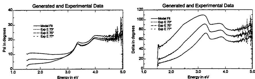
Figure 5.3. VASE data fits for the CdZnTe substrate measured exsitu.
