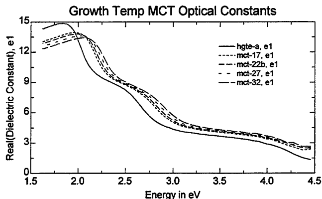
Figure 5.25. Real part of the \text{Hg}_{1-x}\text{Cd}_x\text{Te} dielectric constant at 180^\circ\text{C} .
