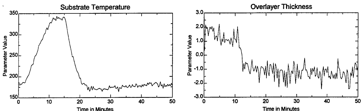
Figure 6.12. Substrate properties during heat-clean for Run #032896
