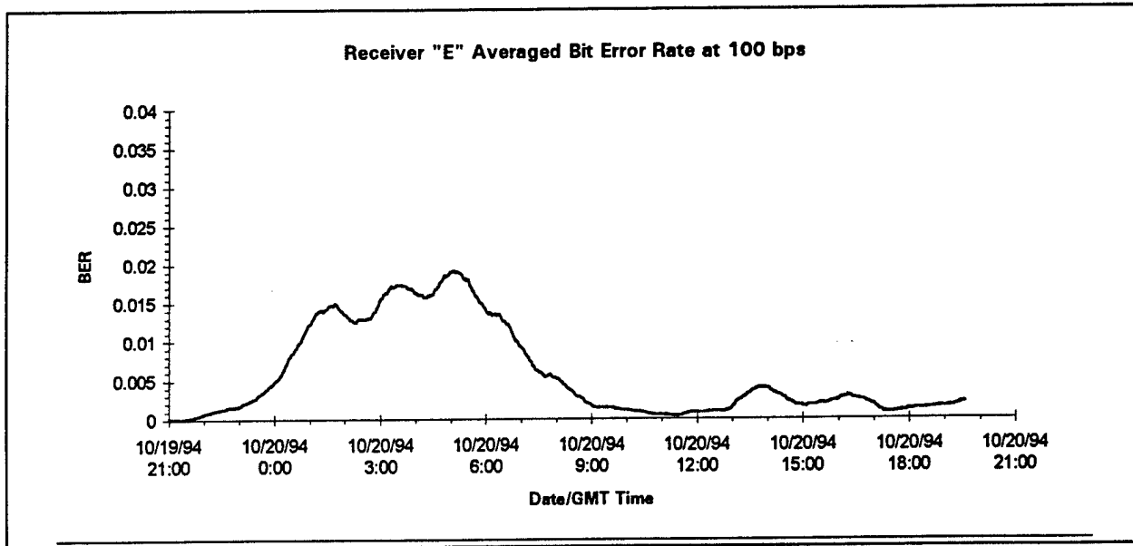
Figure 7 Receiver E Averaged Bit Error Rate at 100 BPS
