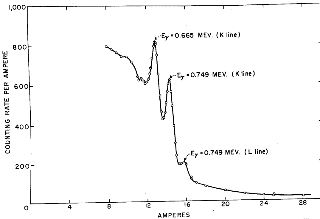
Fig. 3—Photoelectrons ejected from a 1-mil U radiator by gamma rays from Zr^{97}-Nb^{97} .
