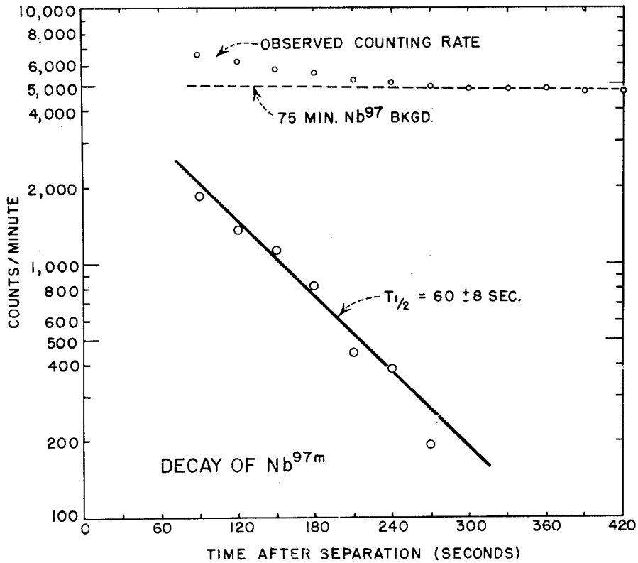
Fig. 6—Decay of Nb fraction separated from Zr 97 -Nb 97 equilibrium mixture.
