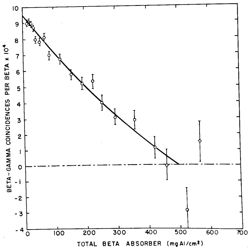
Fig. 4—Beta-gamma coincidences as a function of beta absorber thickness, Zr^{97}-Nb^{97} .
