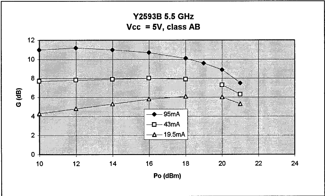
Figure 6 Power Sweep Performance
