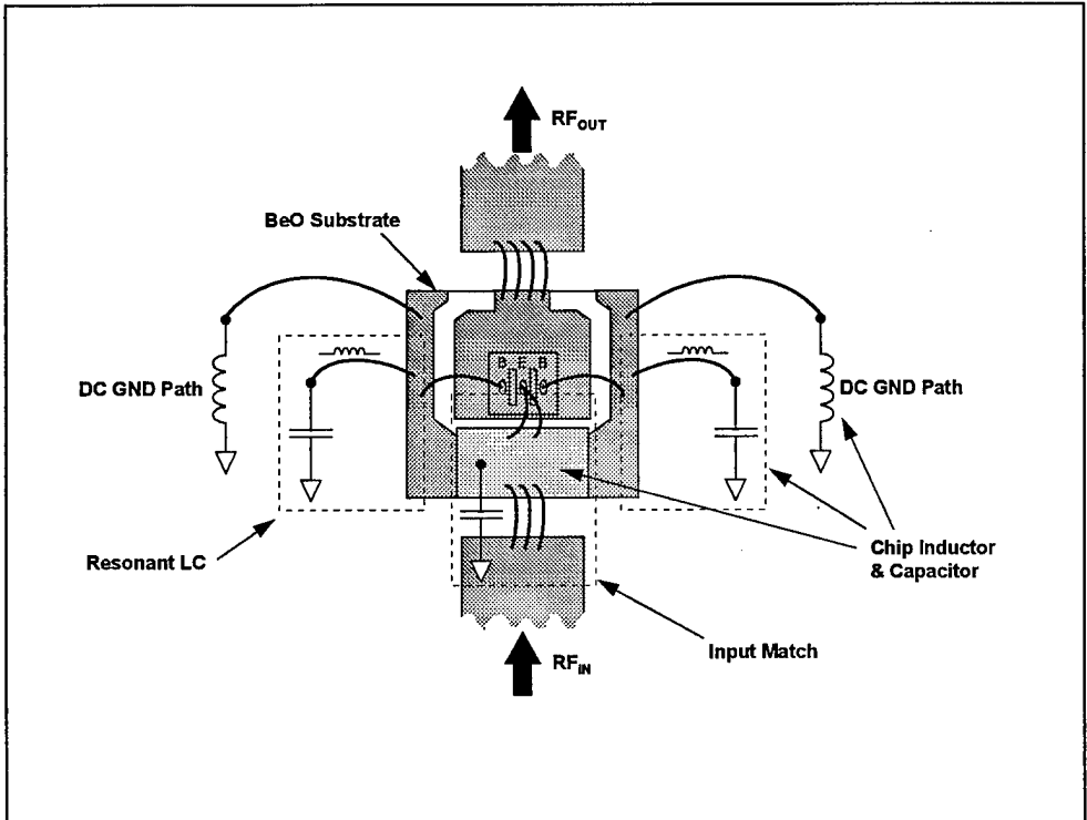
Figure 5 Bonding Diagram of BJT in CR&D Test Fixture @ 6 GHz
