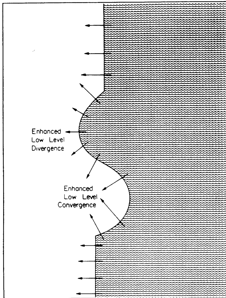
FIGURE 2.3 Schematic of the influence of coastline shape on the sea breeze in the absence of large-scale flow (from Pielke, 1984).
