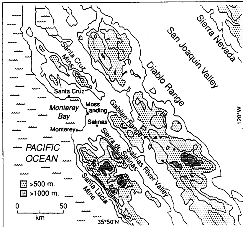
FIGURE 3.2 Topographical map of the Monterey Bay region. The coastal mountains and the valleys impacting the coastal wind flows are shown. Terrain above 500 m has light shading and terrain greater than 1000 m has dark shading (from Banta et al., 1993).
