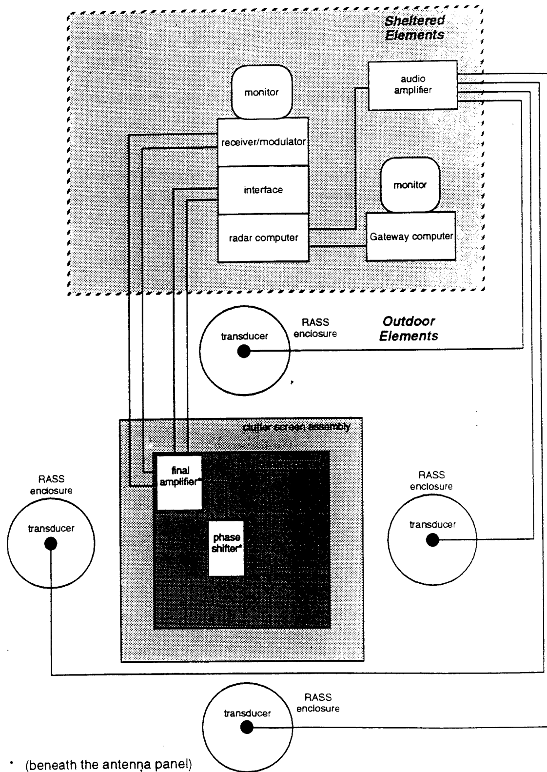
FIGURE 4.2 Diagram displays the location of the RASS transducers in relation to the radar wind profiler when its added as an option. Additionally, the diagram depicts which equipment is sheltered and which equipment remains unprotected from the elements (from Radian Corp., Training Guide for the LAP-3000 , 1994 with permission).
