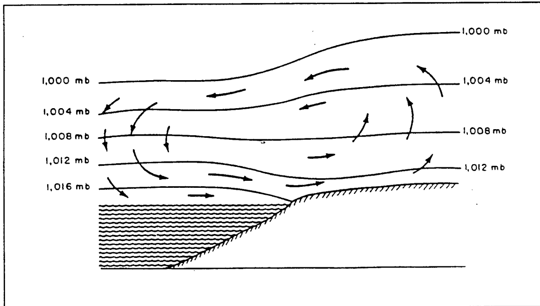
FIGURE 2.1. This Sea-Breeze schematic demonstrates the upward bending of the isobars over the land and the subsequent seaward flow of the upper air. Completing this circulation, low-level air over the sea is flowing landward (from Blair and Fite 1965).
