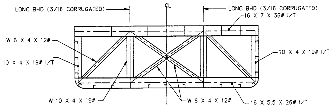
SECTION M-M
