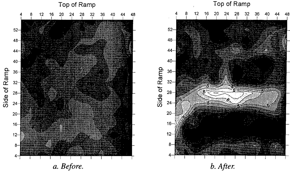
Figure 27. Contour plots of the model riprap before and after test 5. These contour plots show both extent and amount of rock movement during test 5. The numbers along contour lines denote measured distance from the string in the grid frame.
