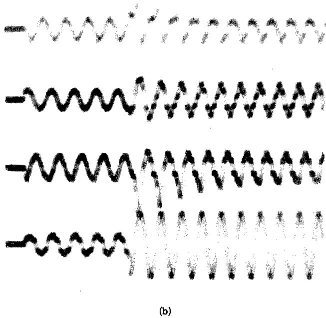
Fig. 6.19—Alpha II decell-rectifier inrush-current oscillograms. (a) Without step-start equipment. (b) With step-start equipment. (See Table 6.3 for details.)
