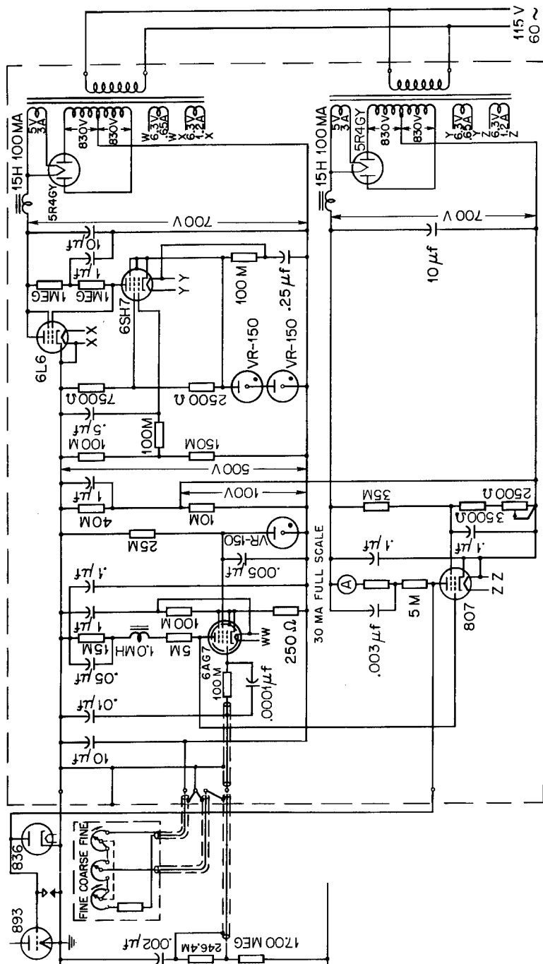
Fig. 7.5—Schematic diagram of Alpha I and Beta (type 1) decell voltage regulator.
