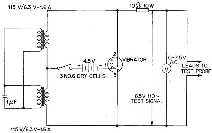
Fig. 20.6—Schematic diagram of a gap tester.
