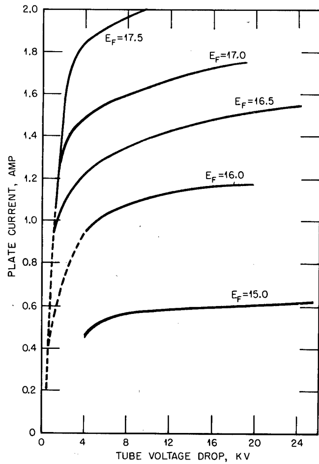
Fig. 2.22 — Characteristic curves for General Electric GL-605 rectifier tube. E_F is the filament voltage.
