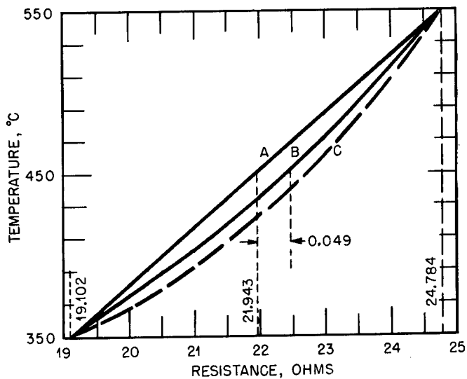
Fig. 14.2 — Resistance-temperature characteristic of Thermohm used in Alpha II and Beta. Nonlinearity exaggerated 10 times. Curve A, linear. Curve B, Thermohm. Curve C, Thermohm and transformer combination.
