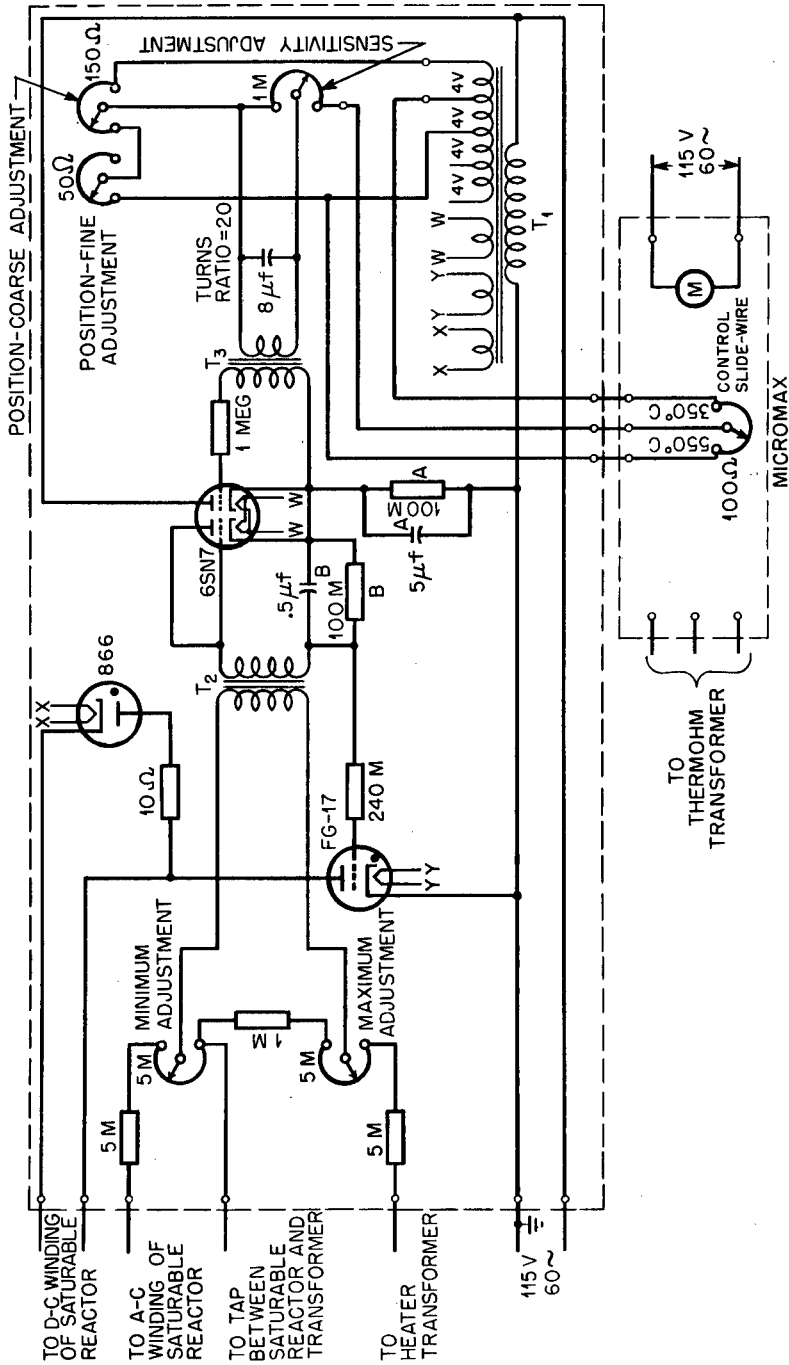
Fig. 14.5—Schematic diagram of General Electric Reactrol control panel.
