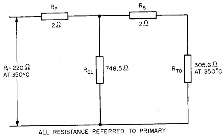
Fig. 14.1 — Equivalent circuit of the Thermohm transformer and Thermohm used in Alpha II and Beta.
