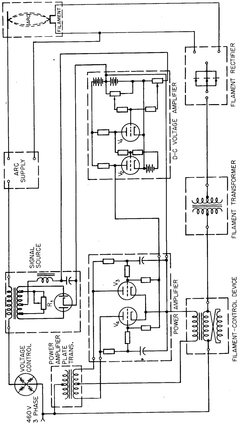
Fig. 13.4 — Simplified schematic diagram of Beta filament-arc regulator.
