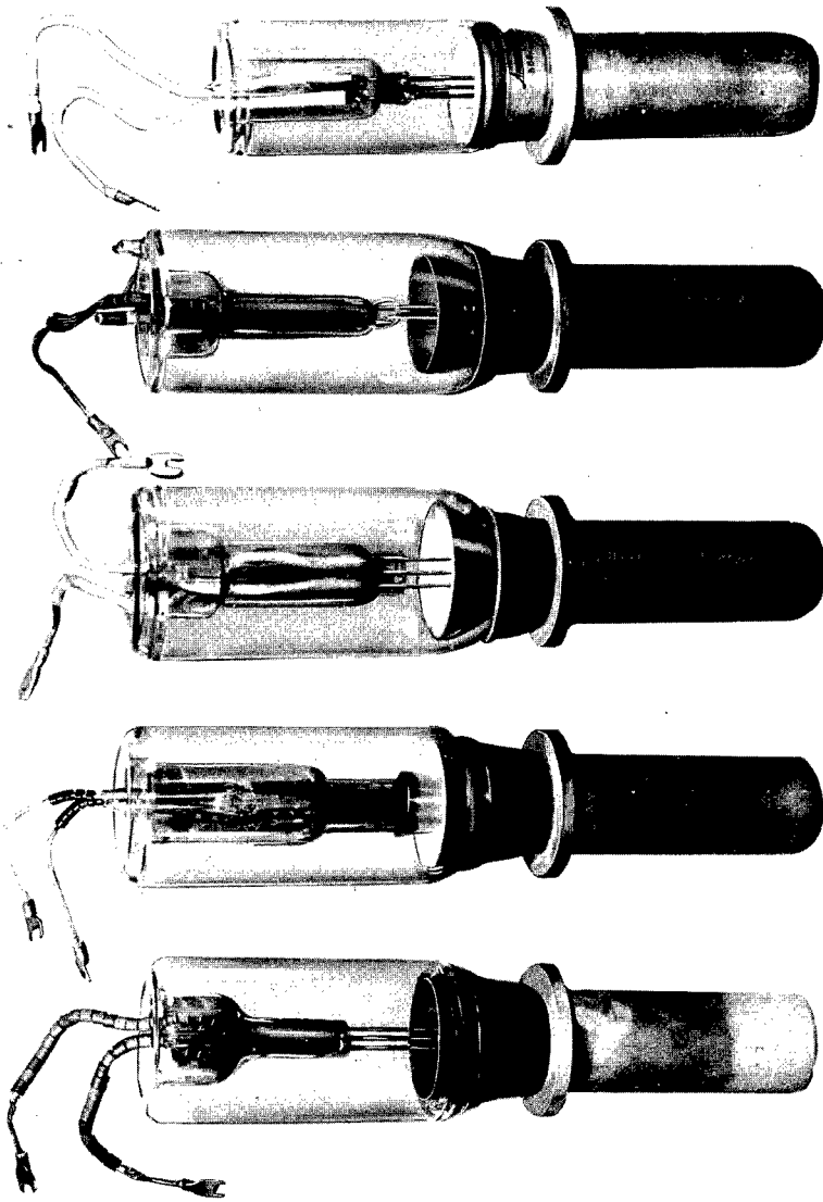
Fig. 5.18 — Water-cooled rectifier tubes.
