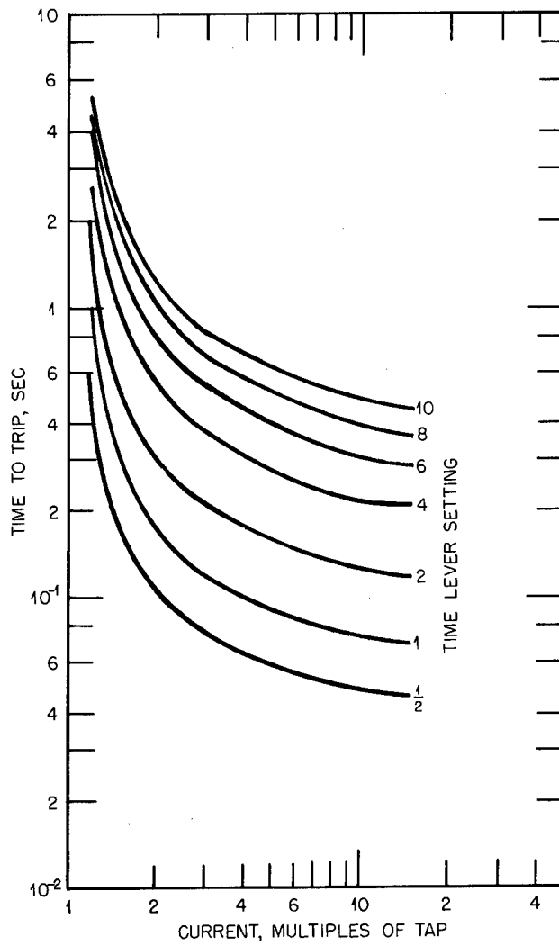
Fig. 6.16—General Electric IAC relay induction time element, approximate time-current characteristic curves.
