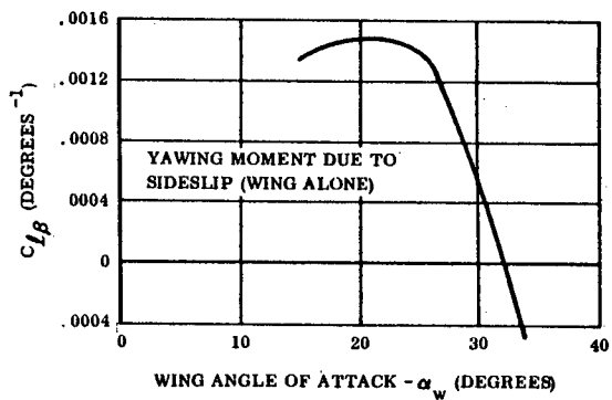
Figure 23. Directional Stability For Wing Alone
