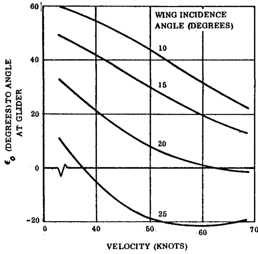
Figure 28. Glider Tow Angle and Associated Altitude Separation
