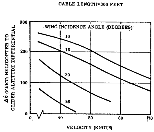
Figure 28. Glider Tow Angle and Associated Altitude Separation
