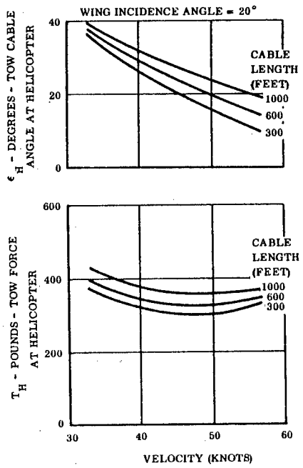
Figure 26. Two Characteristics of the Helicopter
