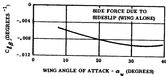
Figure 24. Side Force Variation For Wing Alone
