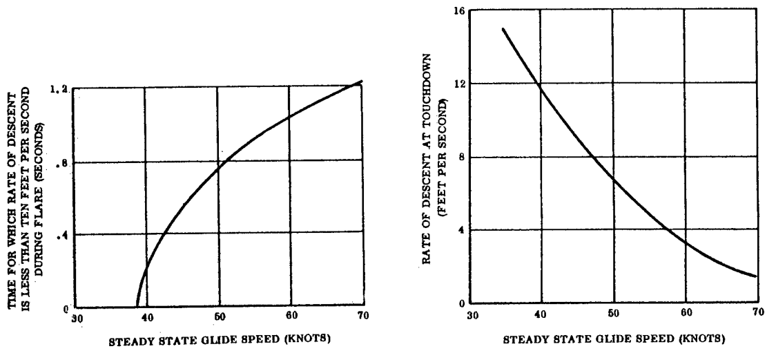
Figure 33. Touchdown Characteristics
