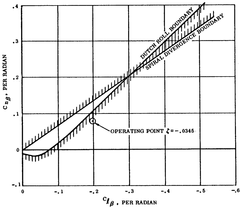
Figure 39. Lateral Directional Stability Boundaries (Two Vertical Tails)
