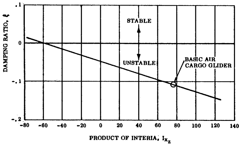
Figure 40. Dutch Roll Damping Ratio as a Function of Product of Inertia
