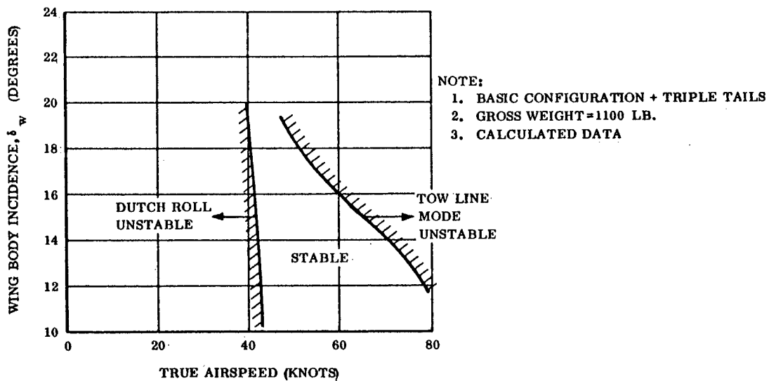
Figure 38. Tow-Speed Boundaries
