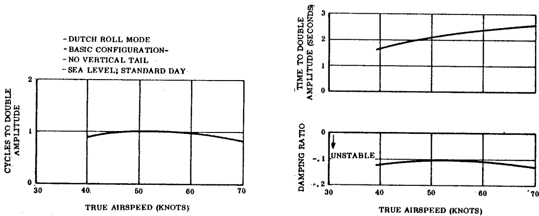
Figure 36. Dynamic Stability
