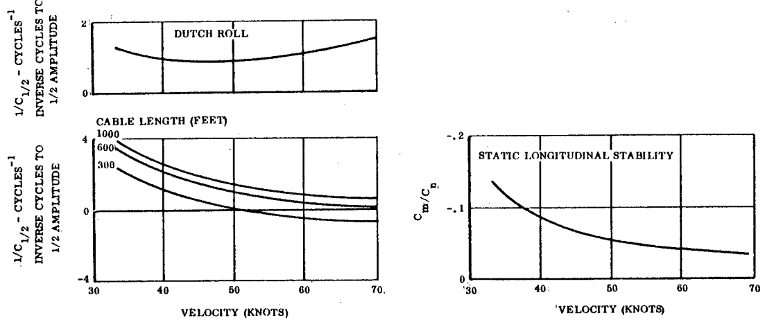
Figure 27. On-Tow Stability
