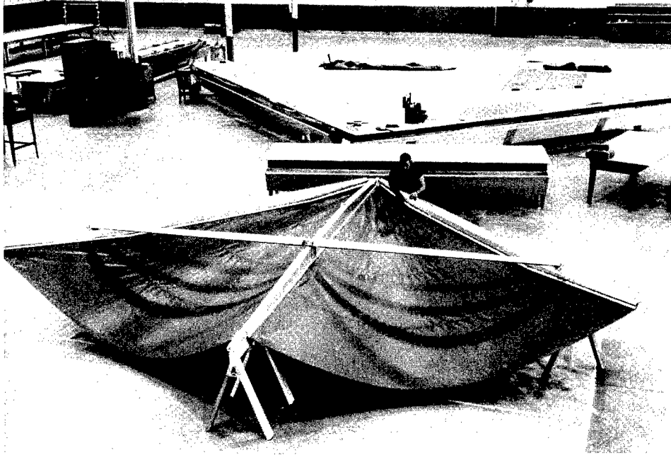
Figure 3. Wing Assembly From Rear
