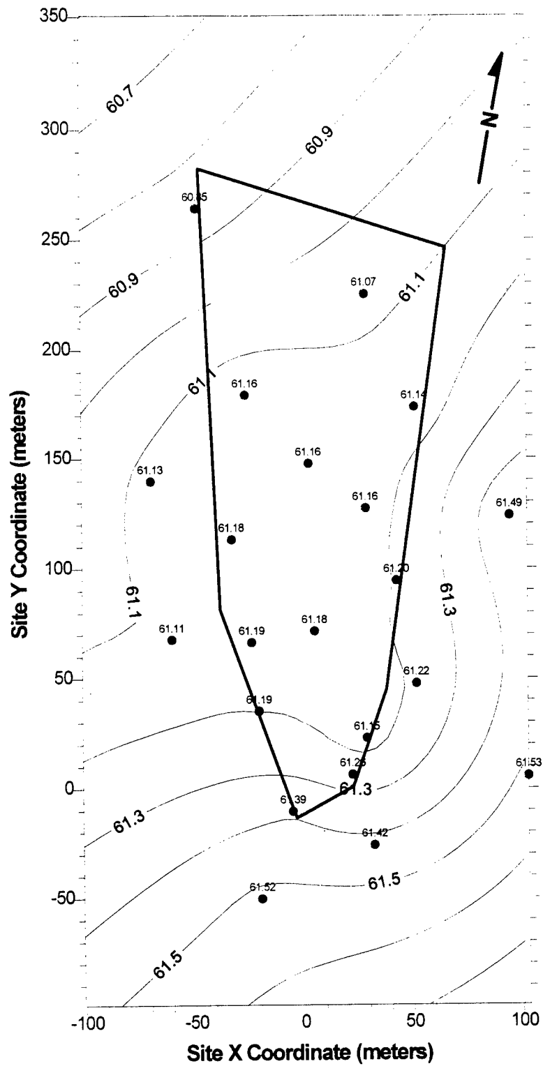
Figure A- 6. Potentiometric Surface Based on Water Levels Measured in A Wells on 11/07/90.
