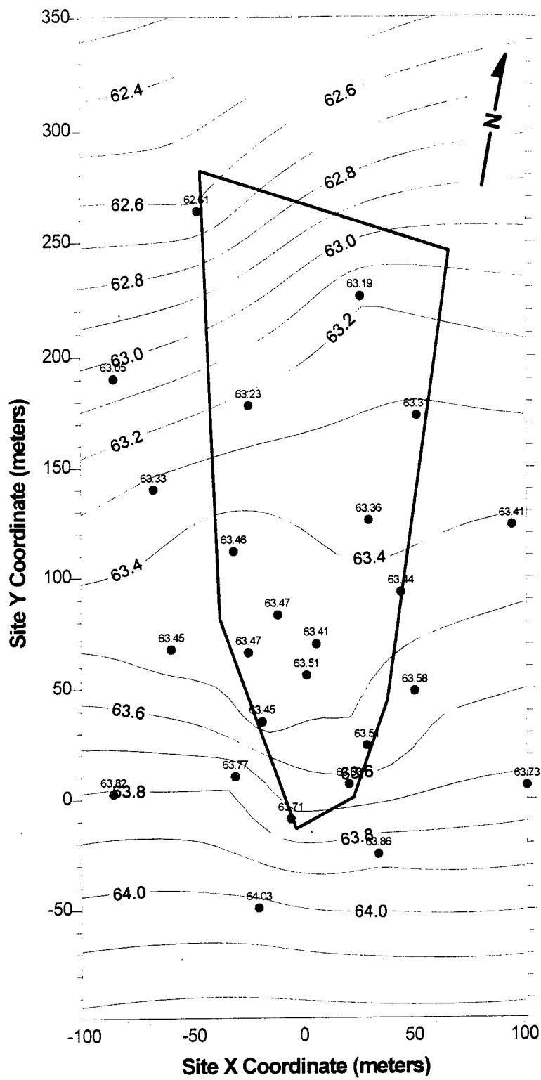
Figure A- 25. Potentiometric Surface Based on Water Levels Measured in B Wells on 01/08/91.
