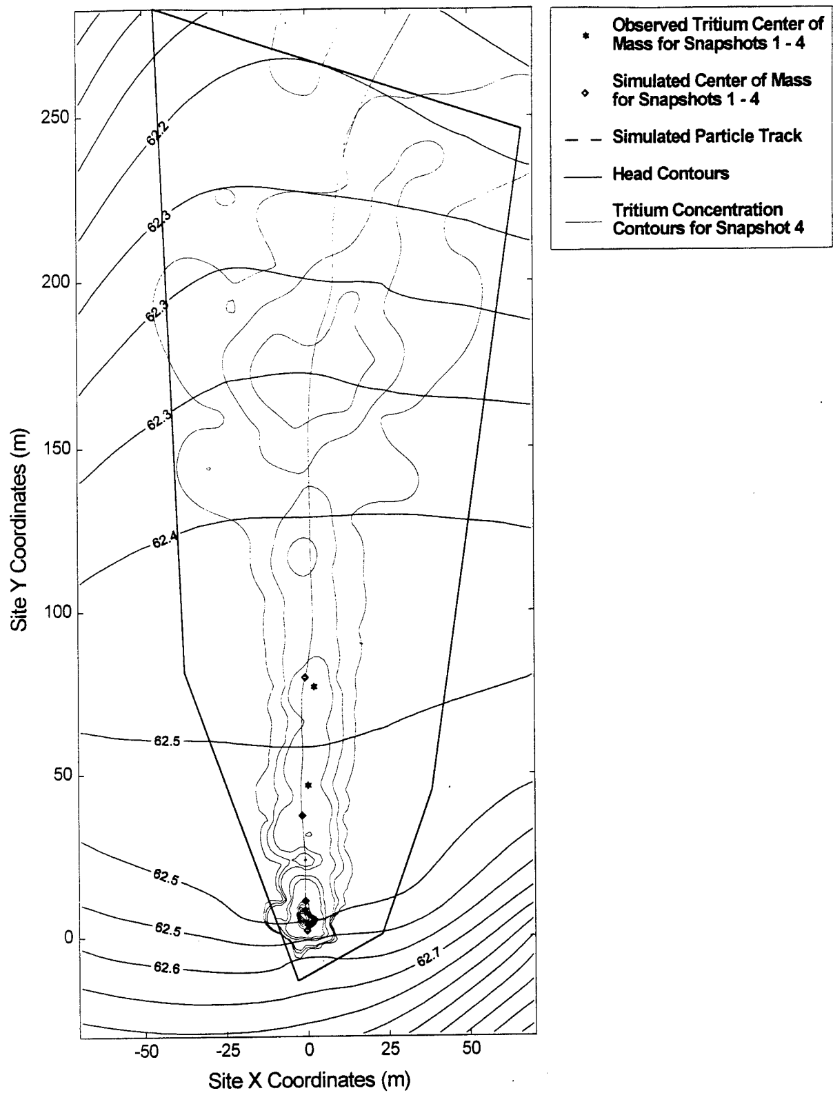
Figure B-20. Simulation 11 : Steady-State Simulated Heads (m amsl) from Refined Grid Model.
