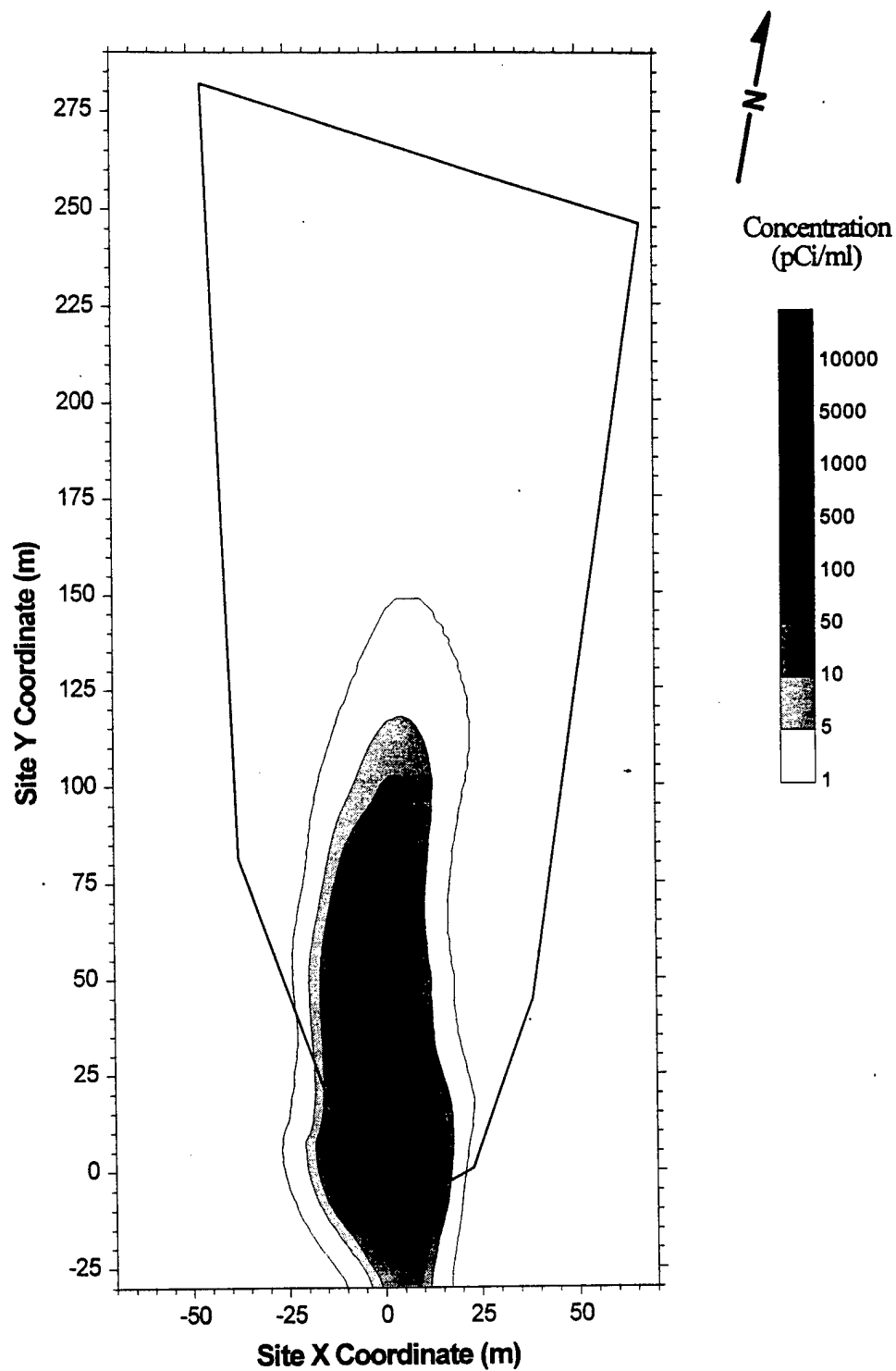
Figure 23. Simulated Tritium Concentration for Snapshot 2 (132 Days After Injection, Pulse Injection Model).
