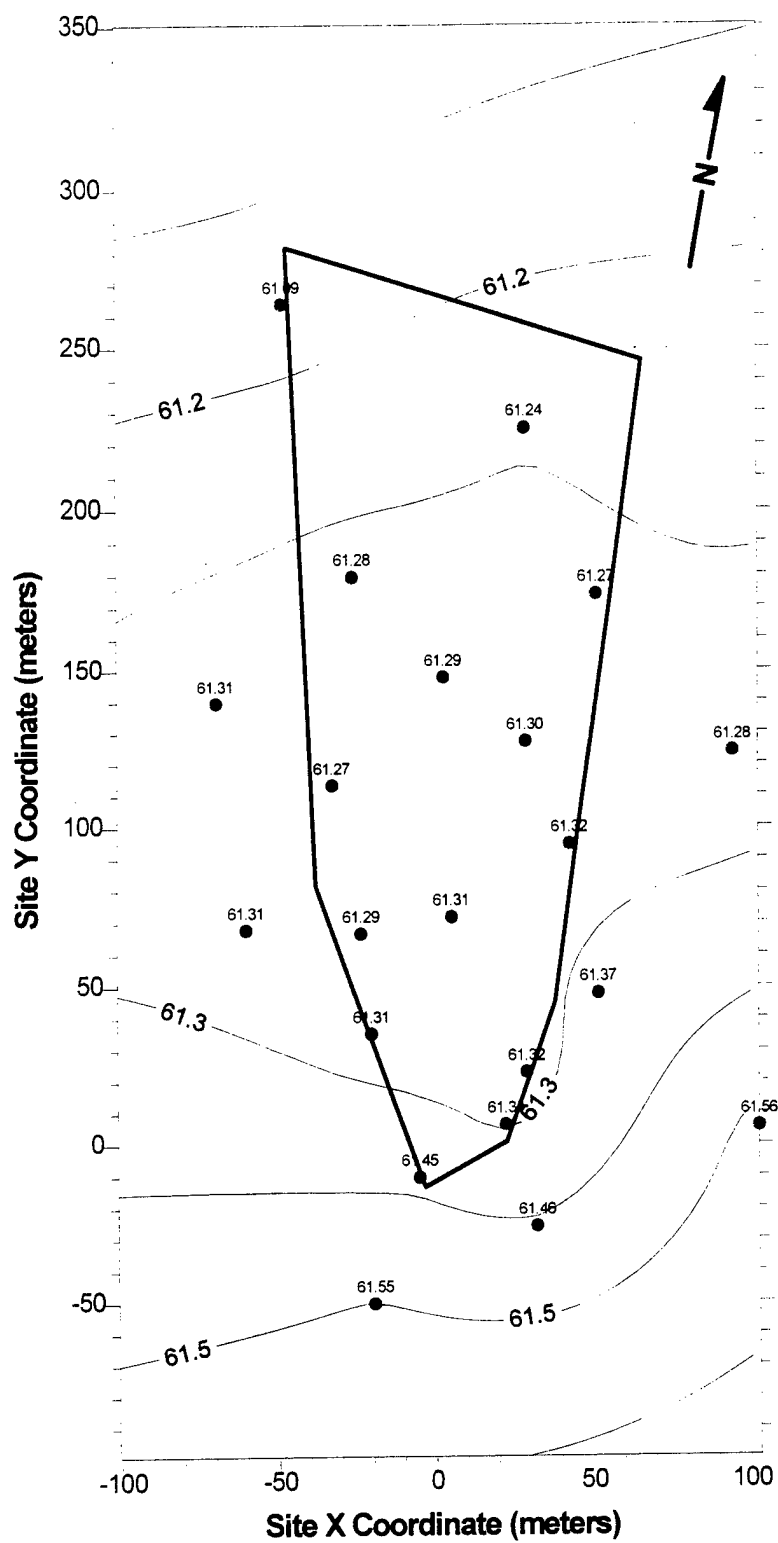
Figure A- 7. Potentiometric Surface Based on Water Levels Measured in A Wells on 12/05/90.
