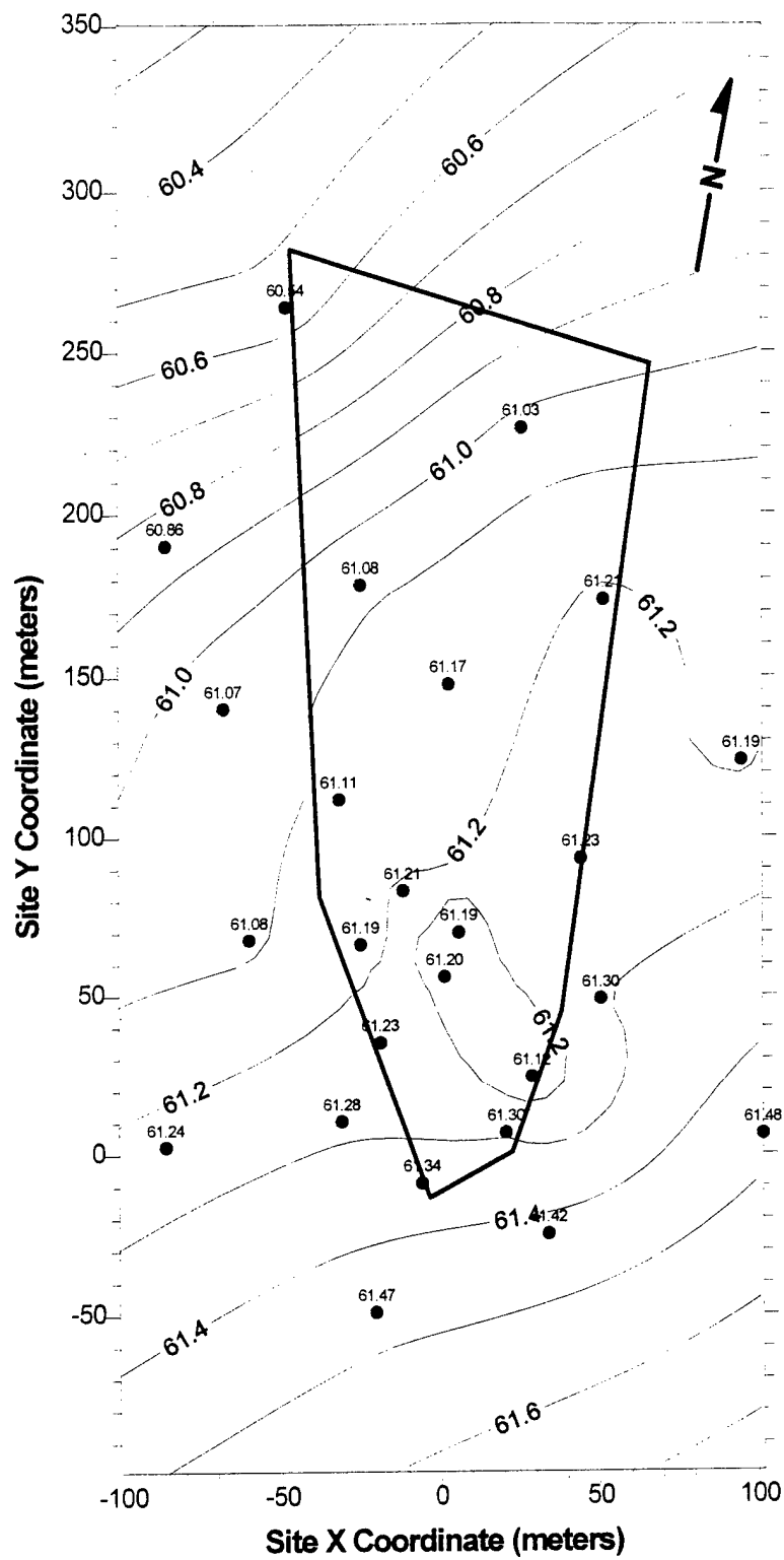
Figure A- 23. Potentiometric Surface Based on Water Levels Measured in B Wells on 11/07/90.
