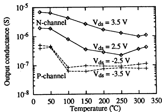
Fig. 5: Output conductance of SOI transistors as a function of temperature. W/L=50\mu\text{m}/10\mu\text{m} , V_{gs}=\pm 1.5\text{V} .
