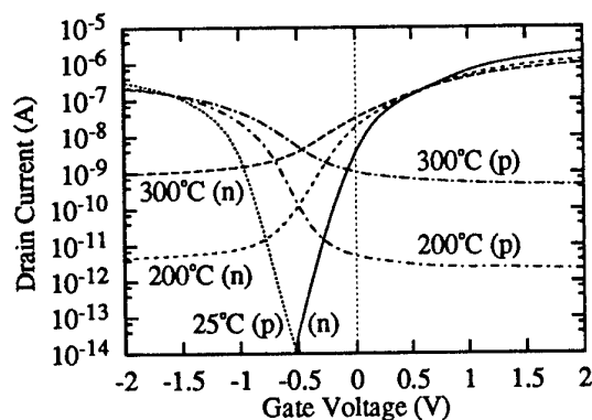
Fig. 2: \log I_d(V_g) of n- and p-channel SOI MOSFETs at different temperatures. W/L=3\mu\text{m}/3\mu\text{m} , V_{ds}=\pm 50\text{ mV} .
