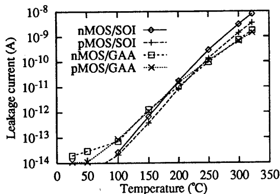
Fig. 3: Leakage current in regular SOI and GAA transistors as a function of temperature. W/L=3\mu\text{m}/3\mu\text{m} , V_{gs}=\pm 1.5\text{V} , V_{ds}=\pm 1\text{V} .
