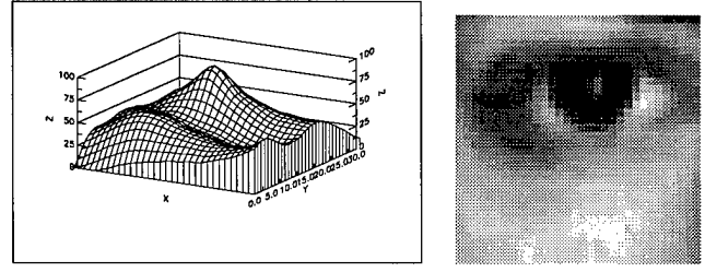
Figure 2: The cross-correlation of the template reported on the right. Note the diffuse shape of the peak that makes its localization difficult
