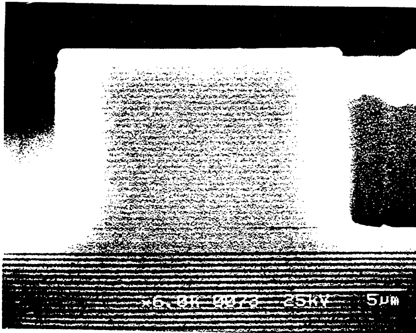
Cross-section of finished oxidized device
