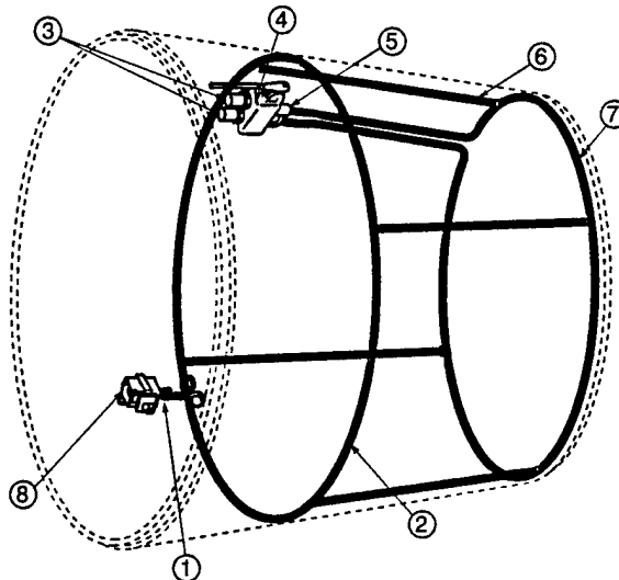
Figure 9. Interstage Ordnance Configuration
