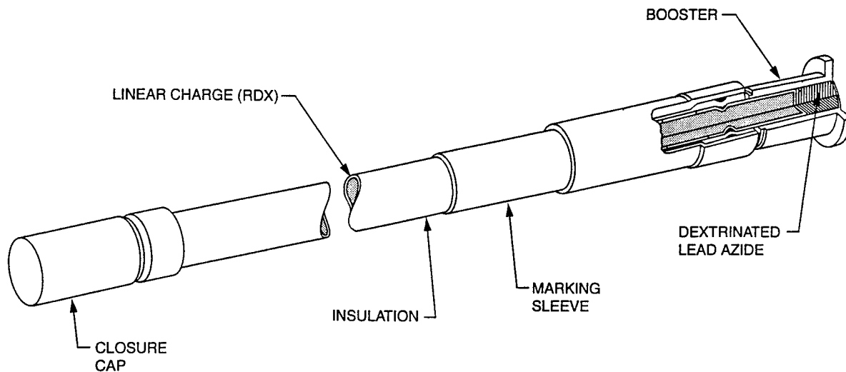
Figure 15. The Design of the Longitudinal Linear Explosive
