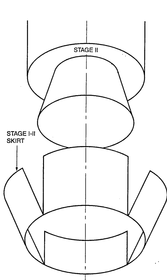
Figure 16. Completion of Skirt Removal Operation
