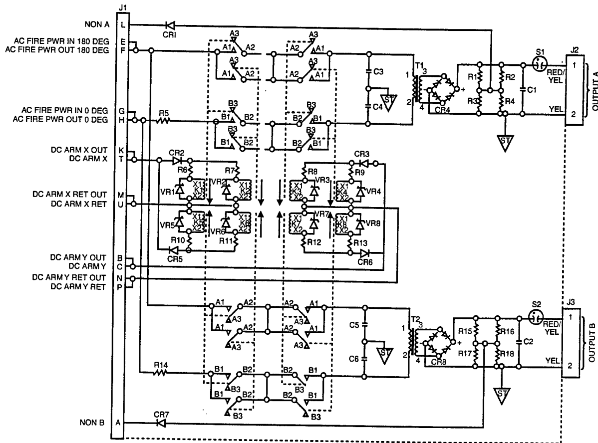
Figure 26. Peacekeeper OIS Firing Unit Schematic
