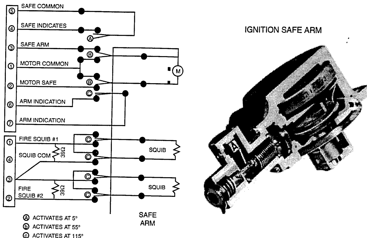
Figure 4. S&A Profile and Electrical Schematic
