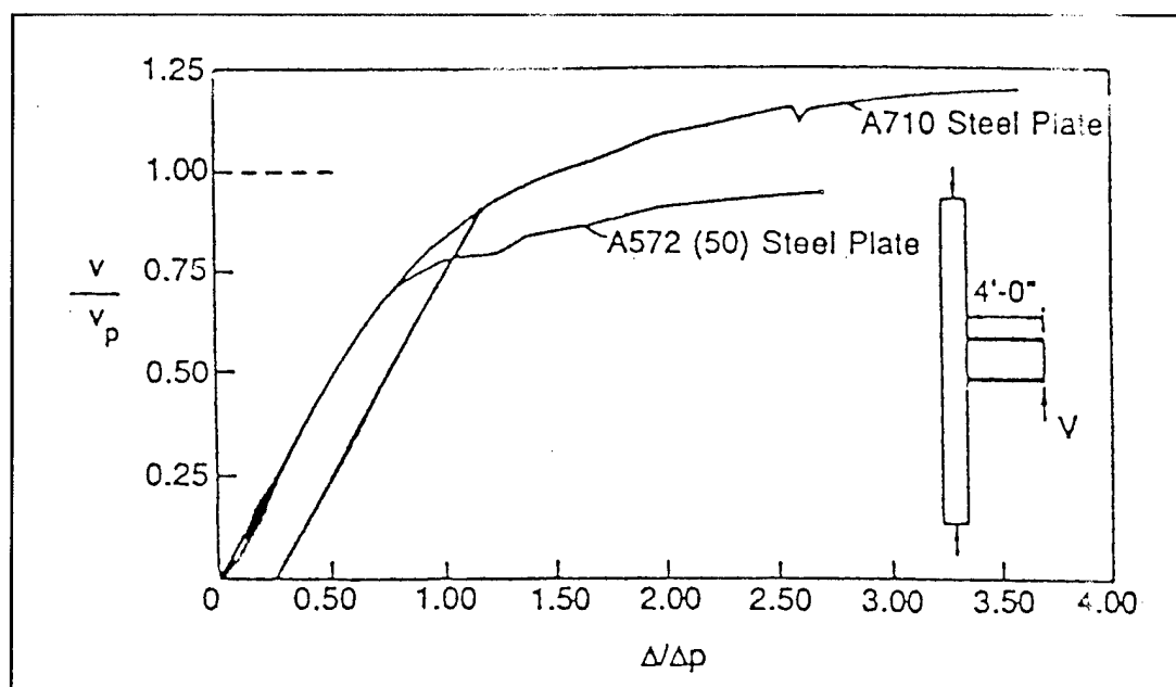
Figure 10. Load-deflection curves of beam-to-column weak axis connections.
