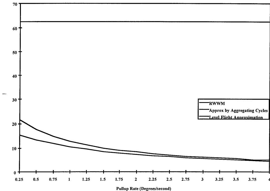
Figure 11, Computation of Weapon Launch Time with Varying Pull-up Rate
