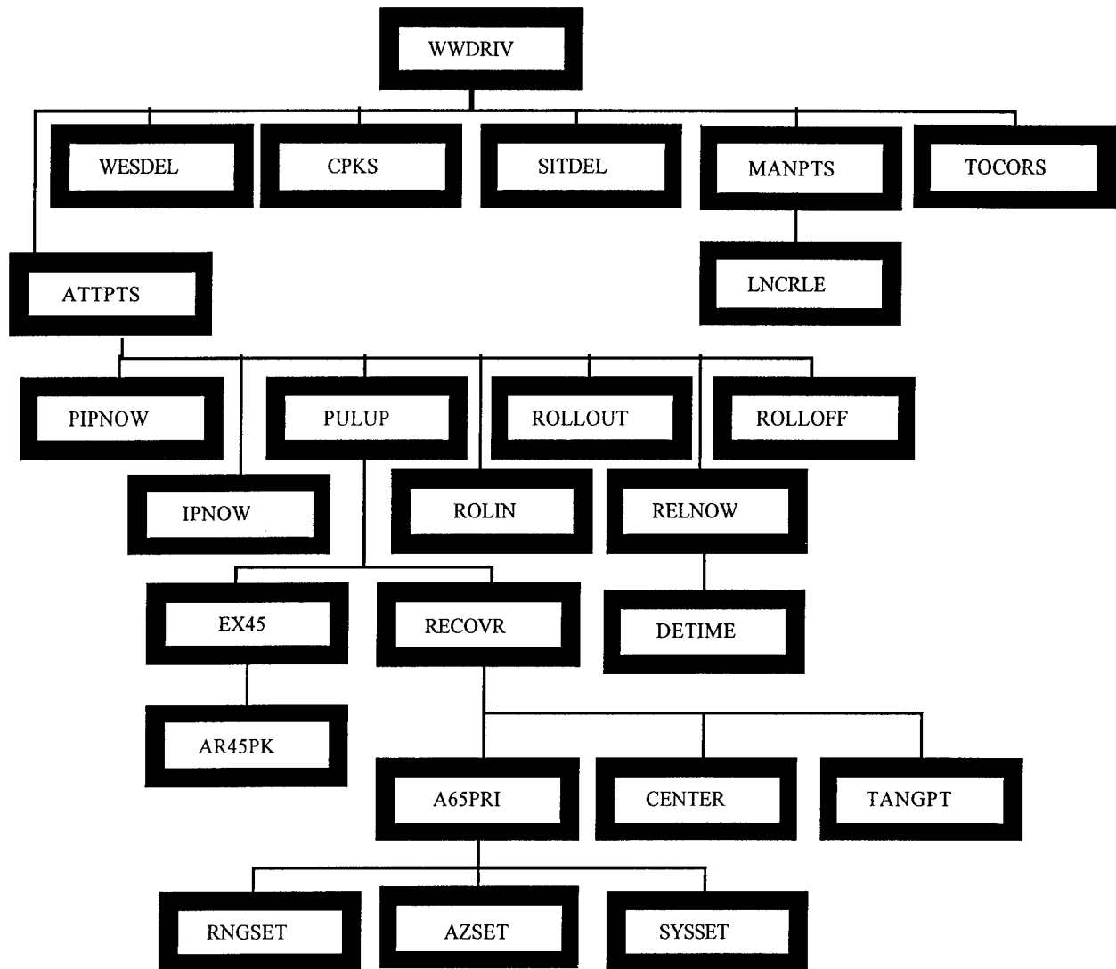
Figure B-7, WWDRIV Calling Structure
