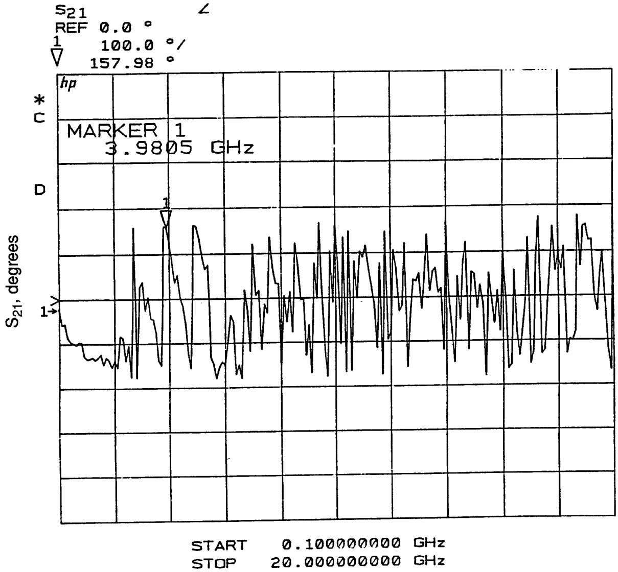
FIGURE C-2. CPW Spiral Delay Line—Withough Ribbon Bridges Transmission Phase.
