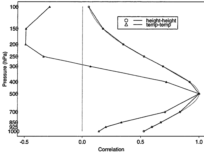
Figure 10: Vertical error correlation functions for climatology for an observation at 500 hPa . Values from table shown as symbols. At intermediate pressures, plotted values are interpolated from the table.
