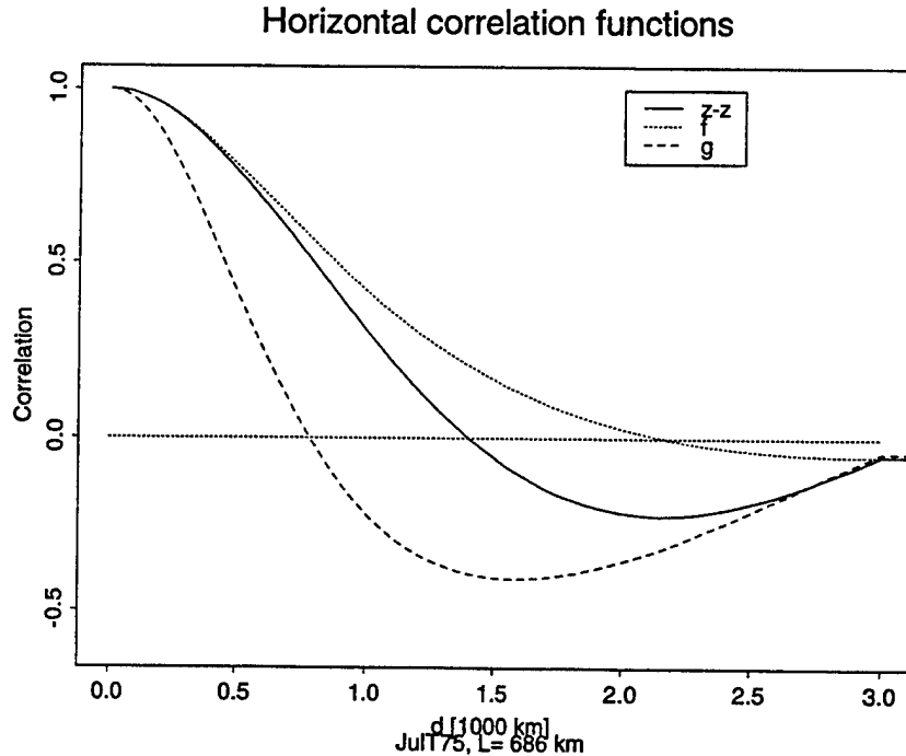
Figure 6: Horizontal height error correlation functions for climatology.
