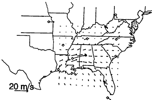
Figure 4: Wind increments at 700 hPa for hurricane Opal, from a winds-only analysis.
