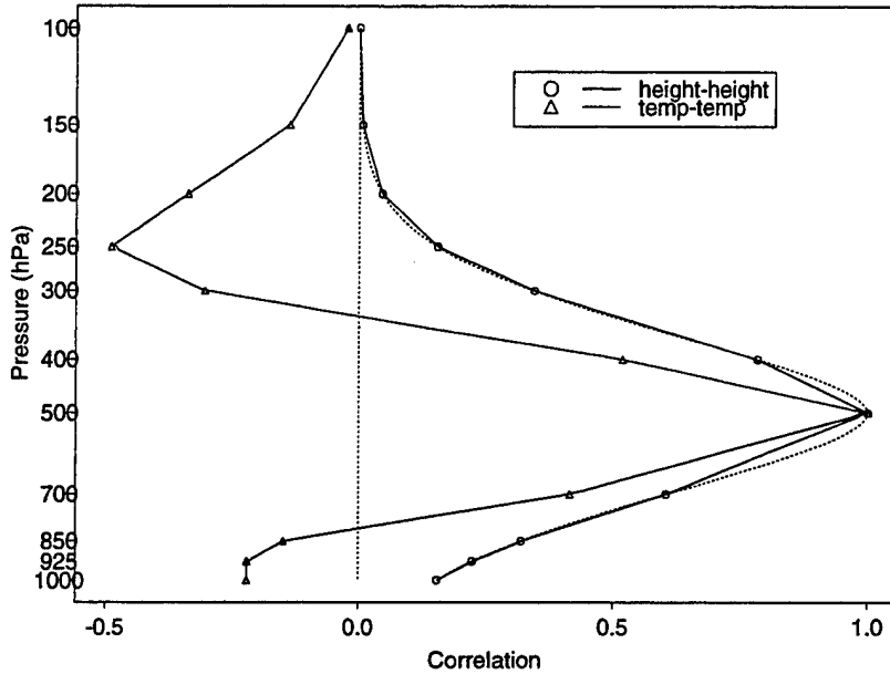
Figure 9: Vertical error correlation functions for NOGAPS for an observation at 500 hPa . Values from table shown as symbols. At intermediate pressures, plotted values are interpolated from the table (solid lines) or computed from continuous functional form (dashed line)
