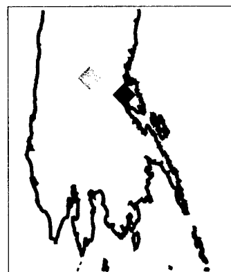
FIG 32. Conditional probability summary for snow during an El Niño JFM season. Diamonds represent the probability \bar{X}_{EN} > \bar{X}_{all} + \sigma_{all} .
