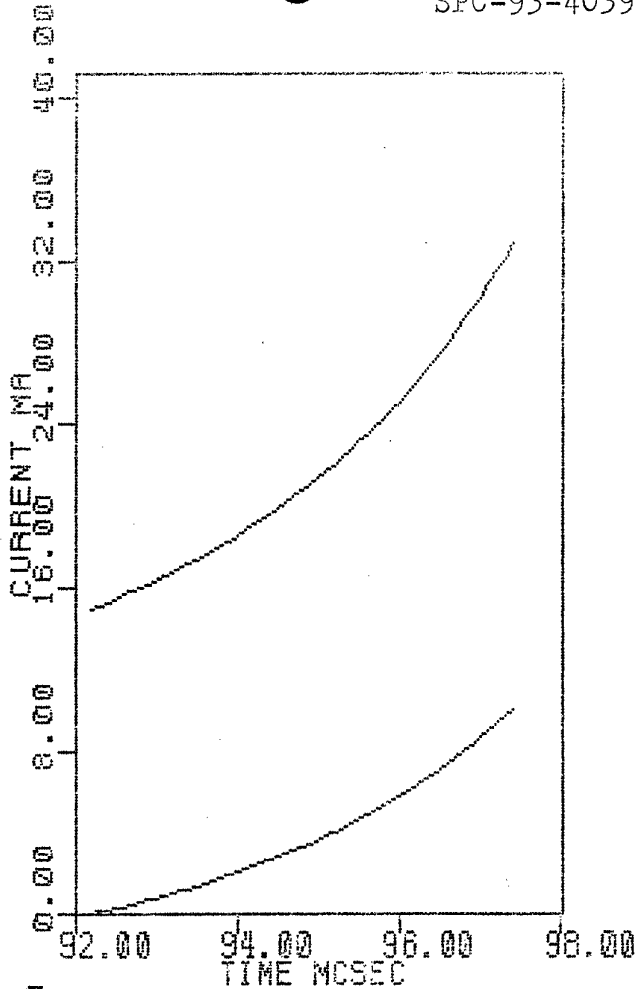
▲▲ FIG.8. CALCULATED GENERATOR HV62 COIL CURRENT JC, AND LOAD CURRENT JL, AFTER FLUX CAPTURE MOMENT.
