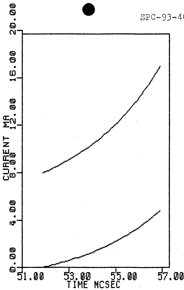
▲▲ FIG.4. CALCULATED GENERATOR HVG1 COIL CURRENT JC, AND LOAD CURRENT JL, AFTER FLUX CAPTURE MOMENT.
