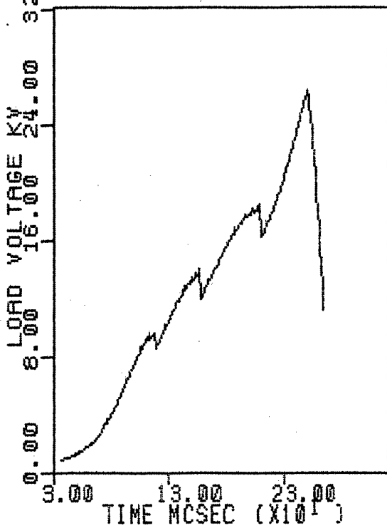
FIG.18. CALCULATED GENERATOR SG LOAD VOLTAGE.
