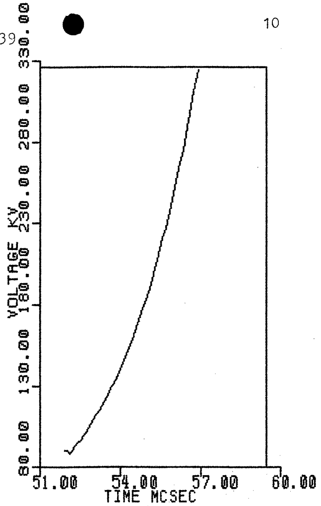
FIG.5. CALCULATED CABLE LINE VOLTAGE FOR HVG1.
