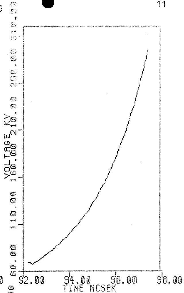
FIG.9. CALCULATED CABLE LINE VOLTAGE FOR HV62.
