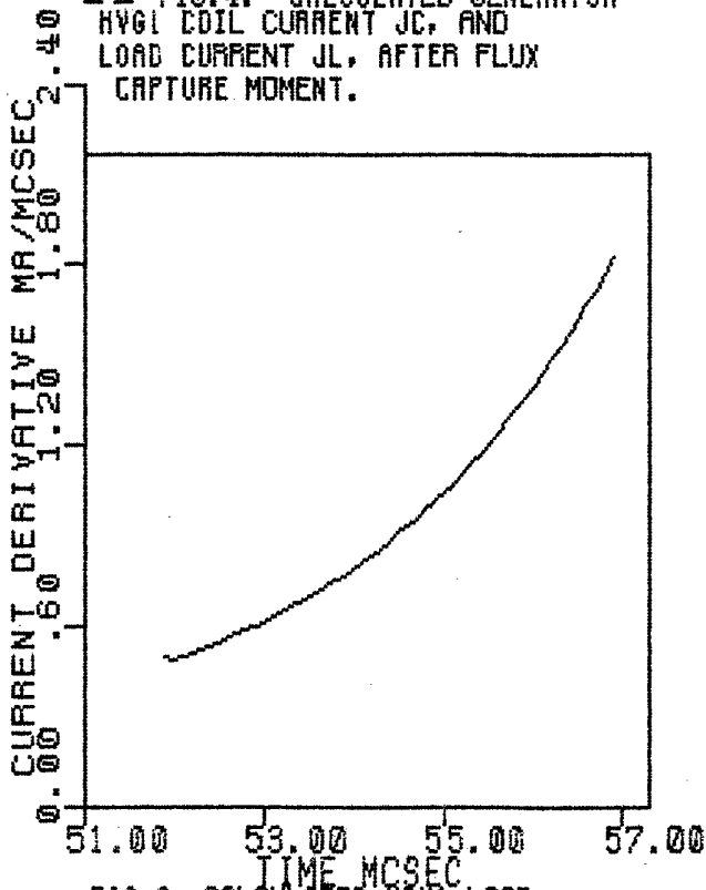
FIG.6. CALCULATED HVG1 LOAD CURRENT DERIVATIVE AFTER FLUX CAPTURE MOMENT.
