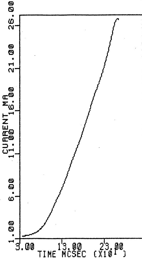
FIG.16. CALCULATED GENERATOR SG CURRENT.
