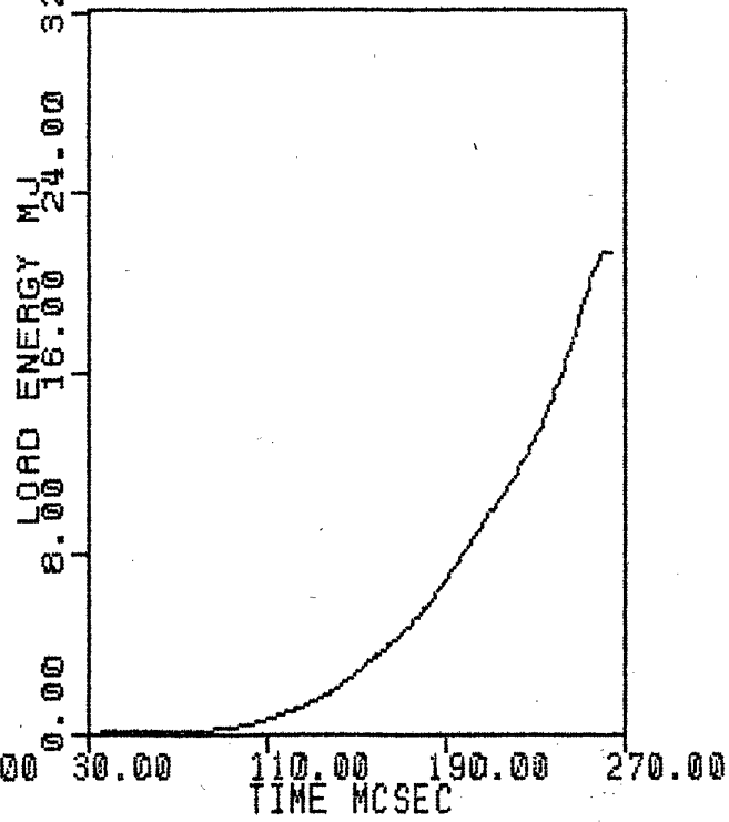
FIG.19. CALCULATED GENERATOR SG LOAD ENERGY.
