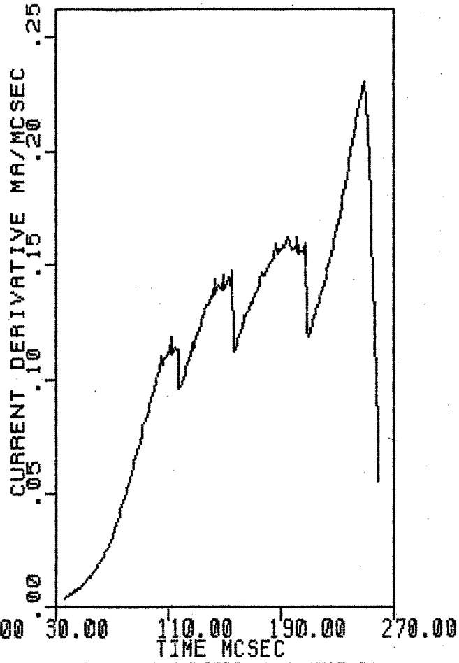
FIG.17. CALCULATED GENERATOR SG LOAD CURRENT DERIVATIVE.
