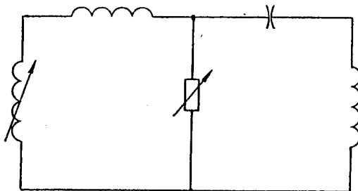
Fig. 13. Electrical scheme for energizing PFD with cascade generators and explosive driven plasma open switch.
