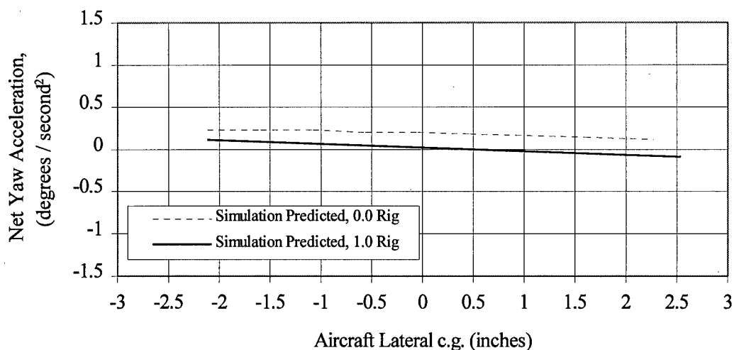
Figure 4-4. Simulator predicted effects of changing differential stabilator bias at 32,000 feet (9,754 meters) PA.
