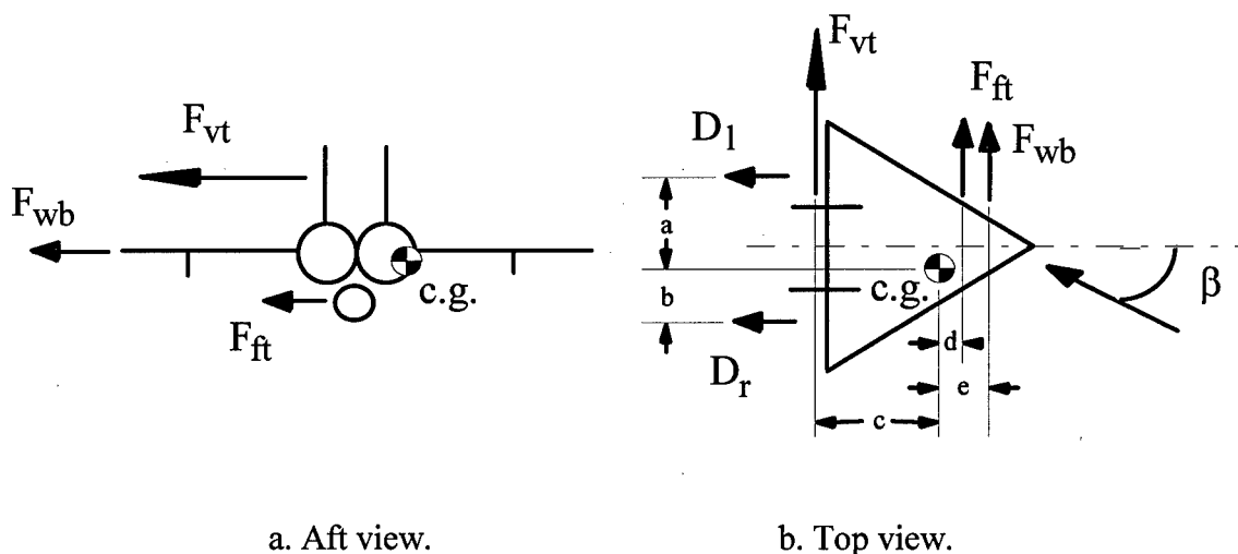
Figure 2-7. Side forces acting on F-15 during a wings level lateral weight asymmetry.
