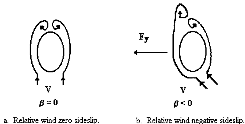
Figure 2-5. Forebody vortex flows over an aircraft nose shape at high AOA.
