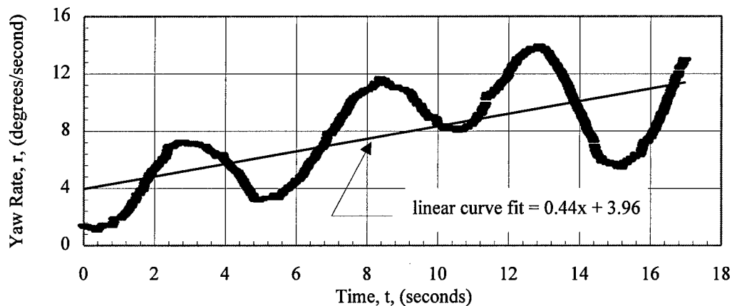
Figure 3-4. F-15B yaw rate at 32,000 feet (9,754 meters) PA for zero fuel asymmetry with 0.4 inch (10.1 millimeter) LLEU and 0.4 inch (10.1 millimeter) RLED.
