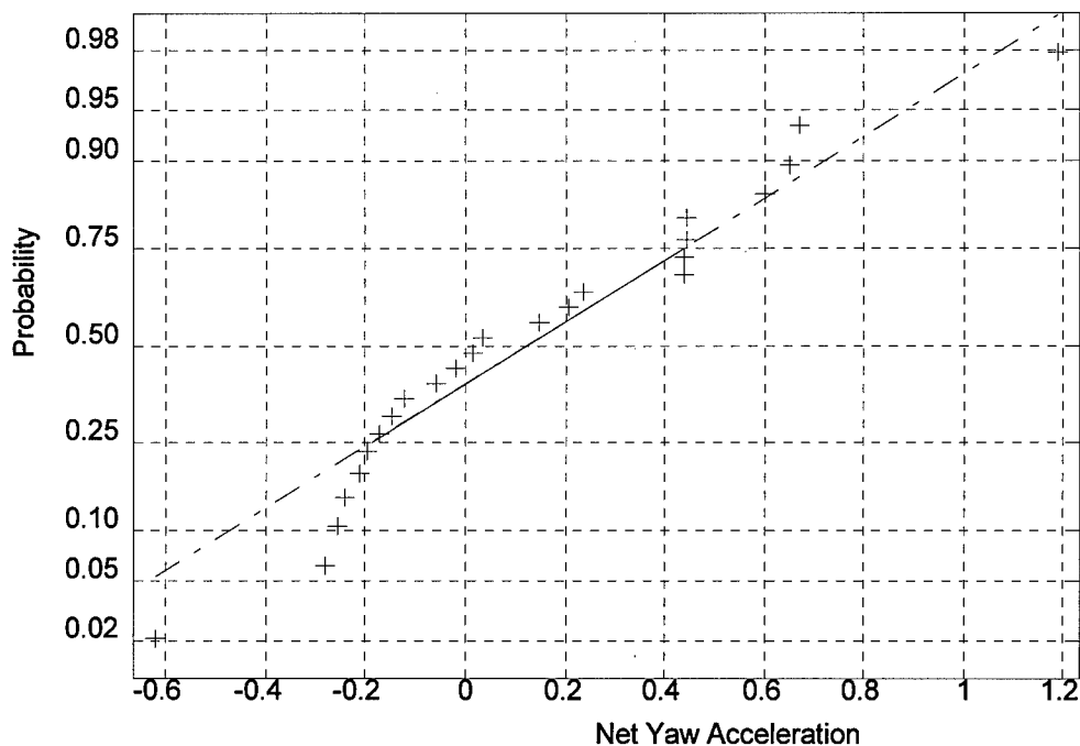
Figure 4.2. Normal probability plot of net yaw acceleration data for example F-15B.
