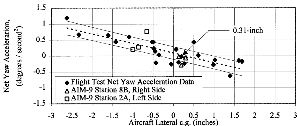
Figure 4-8. Sample AIM-9 missile effects on example F-15B.
