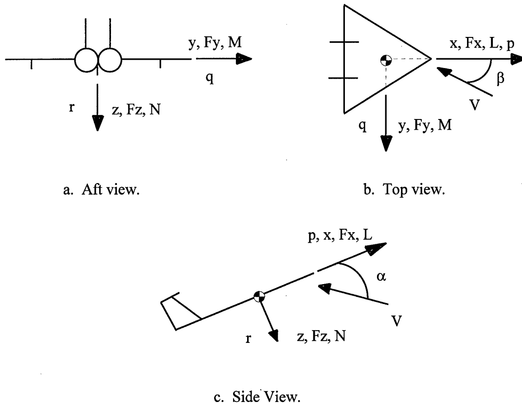
Figure 2-2. Right-handed coordinate System.
