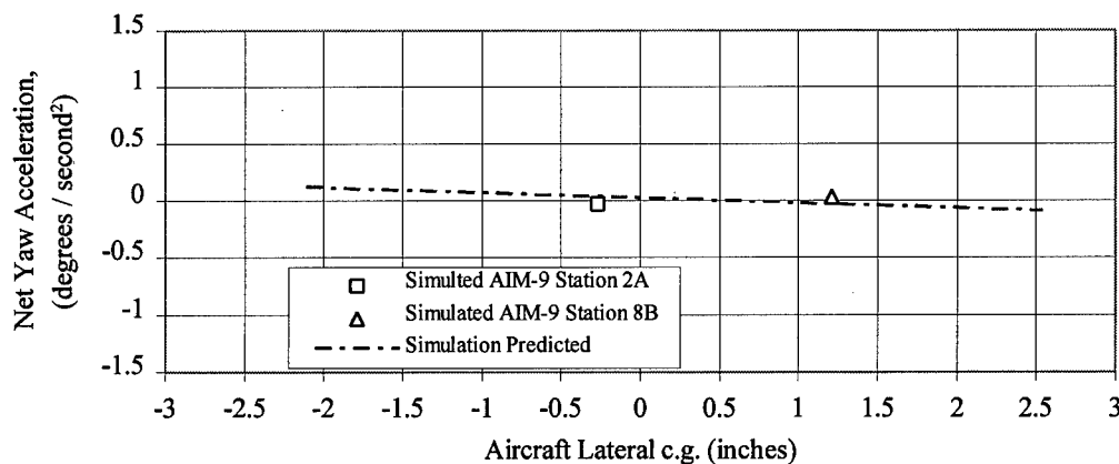
Figure 4-7. F-15 simulation net yaw acceleration predictions at 32,000 feet (9,754 meters) PA with 0.5-inch (12.7-millimeter) RLED and 0.5-inch (12.7-millimeter) LLEU.
