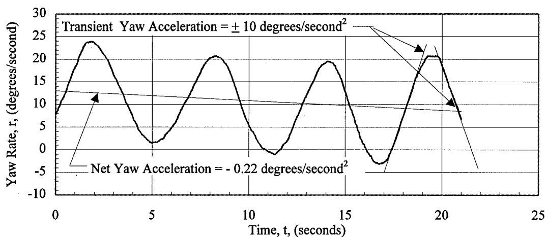
Figure 4-10. Transient yaw acceleration for sample flight test F-15B data.
