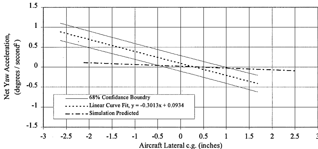
Figure 4-3. Simulation and flight test comparison of F-15 net yaw acceleration at 32,000 feet (9,754 meters) PA, with 0.4-inch (10.1-millimeter) RLED and 0.4-inch (10.1-millimeter) LLEU.
