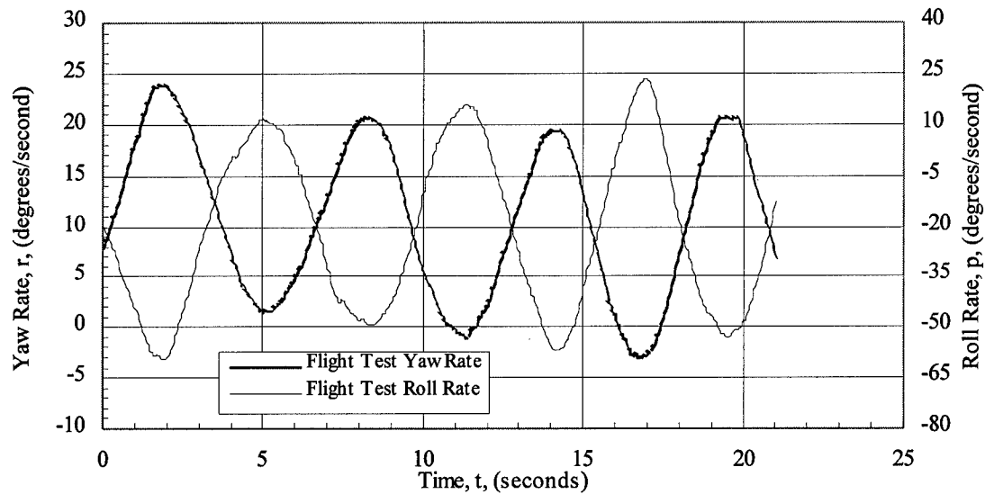
Figure 4-11a. F-15B opposite sense yaw and roll rates.
