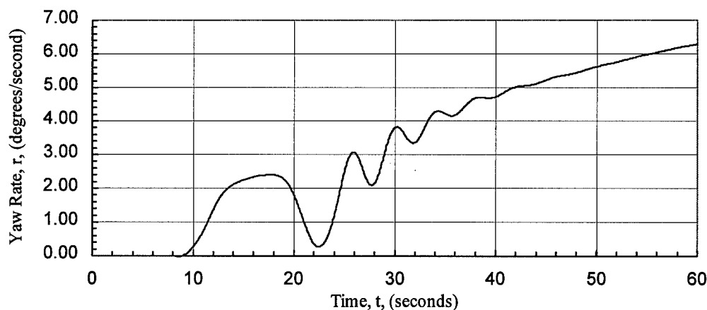
Figure 3-2. Baseline F-15A simulator yaw rate prediction at 15,000 feet (4,572 meters) PA, with symmetric stabilators.
