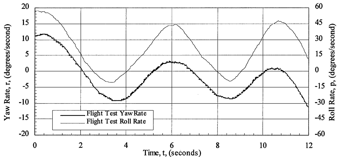
Figure 4-11b. F-15B same sense yaw and roll rates.
