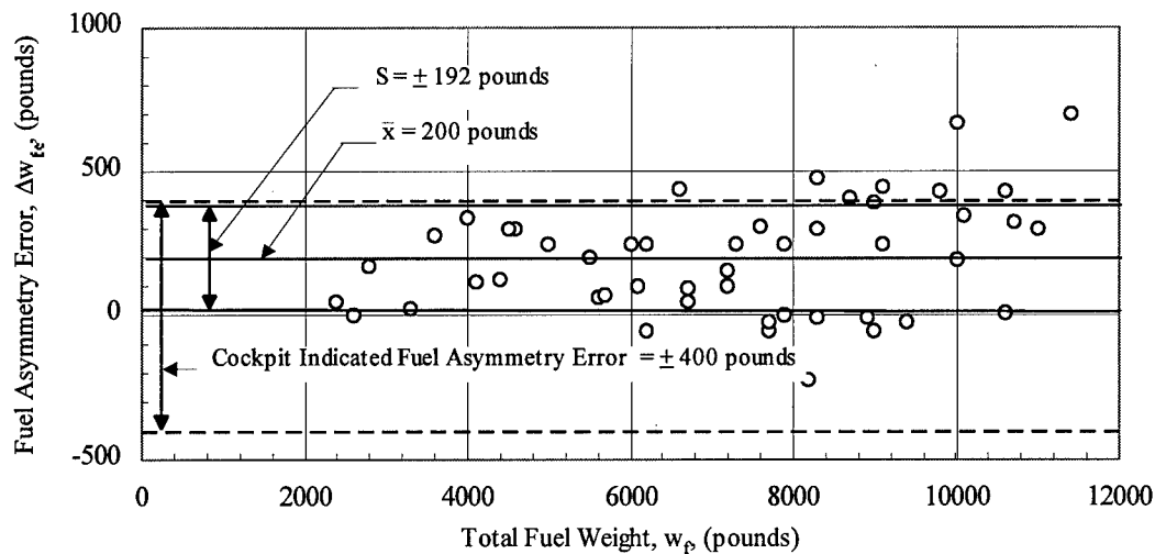
Figure 4-12. F-15B S/N 76-0130 lateral fuel asymmetry error, front cockpit indicator.
