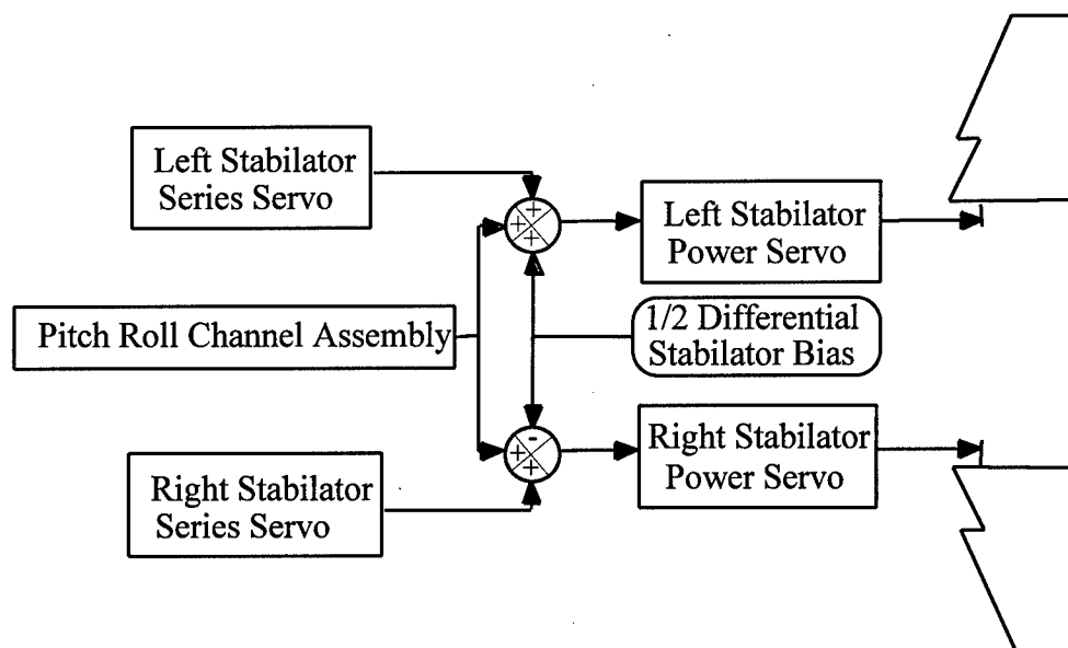
Figure 3-1. Differential stabilator bias implementation.
