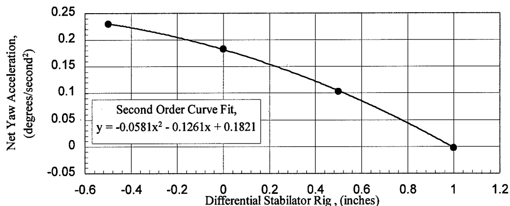
Figure 4-9. Simulator predicted net yaw acceleration for various differential stabilator rigs at 32,000 feet (9,754 meters) PA and with a 0.471-inch (12.0-millimeters) lateral c.g. shift.
