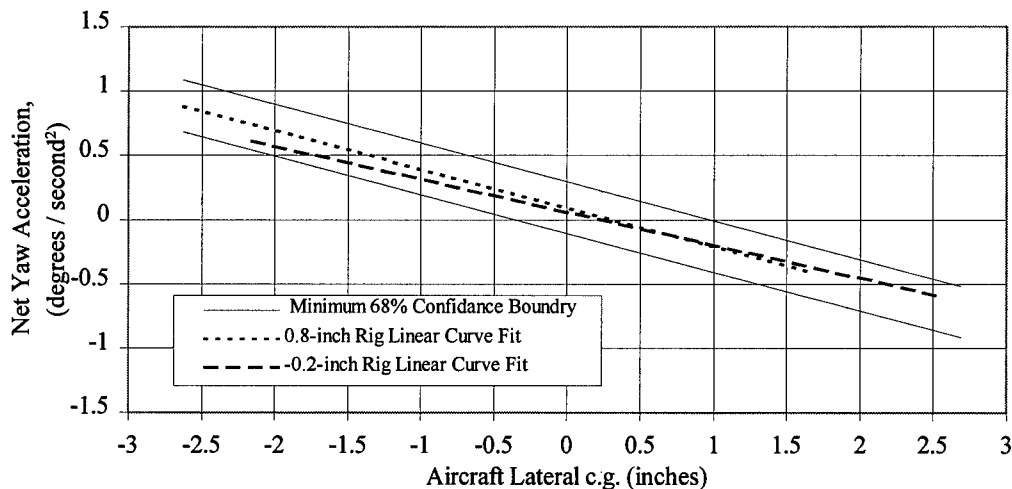
Figure 4-5. F-15B flight test effects of changing differential stabilator at 32,000 feet (9,754 meters) PA.
