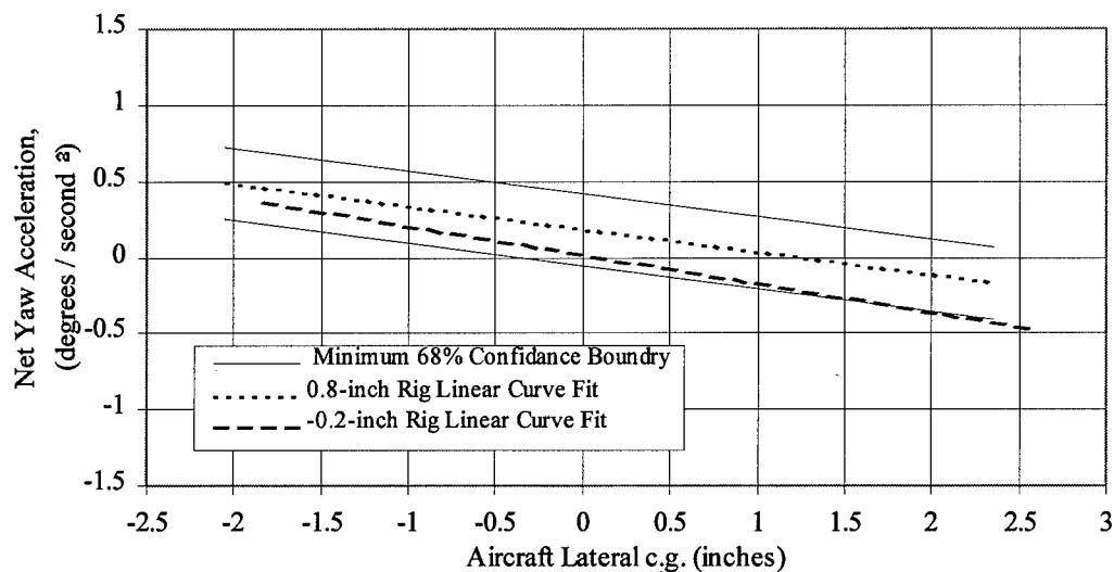
Figure 4-6. F-15B flight test effects of changing differential stabilator at 15,000 feet (4,572 meters) PA.
