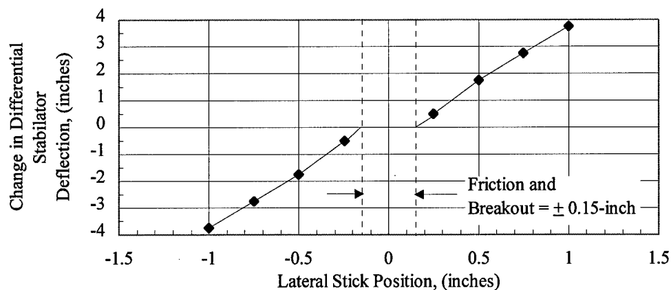
Figure 4-13. Lateral stick position effects on F-15B S/N 76-0130 differential stabilator deflection.
