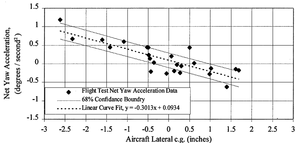
Figure 4-1. F-15B net yaw acceleration at 32,000 feet (9,754 meters) PA, with 0.4-inch (10.1-millimeter) RLED and 0.4-inch (10.1-millimeter) LLEU.
