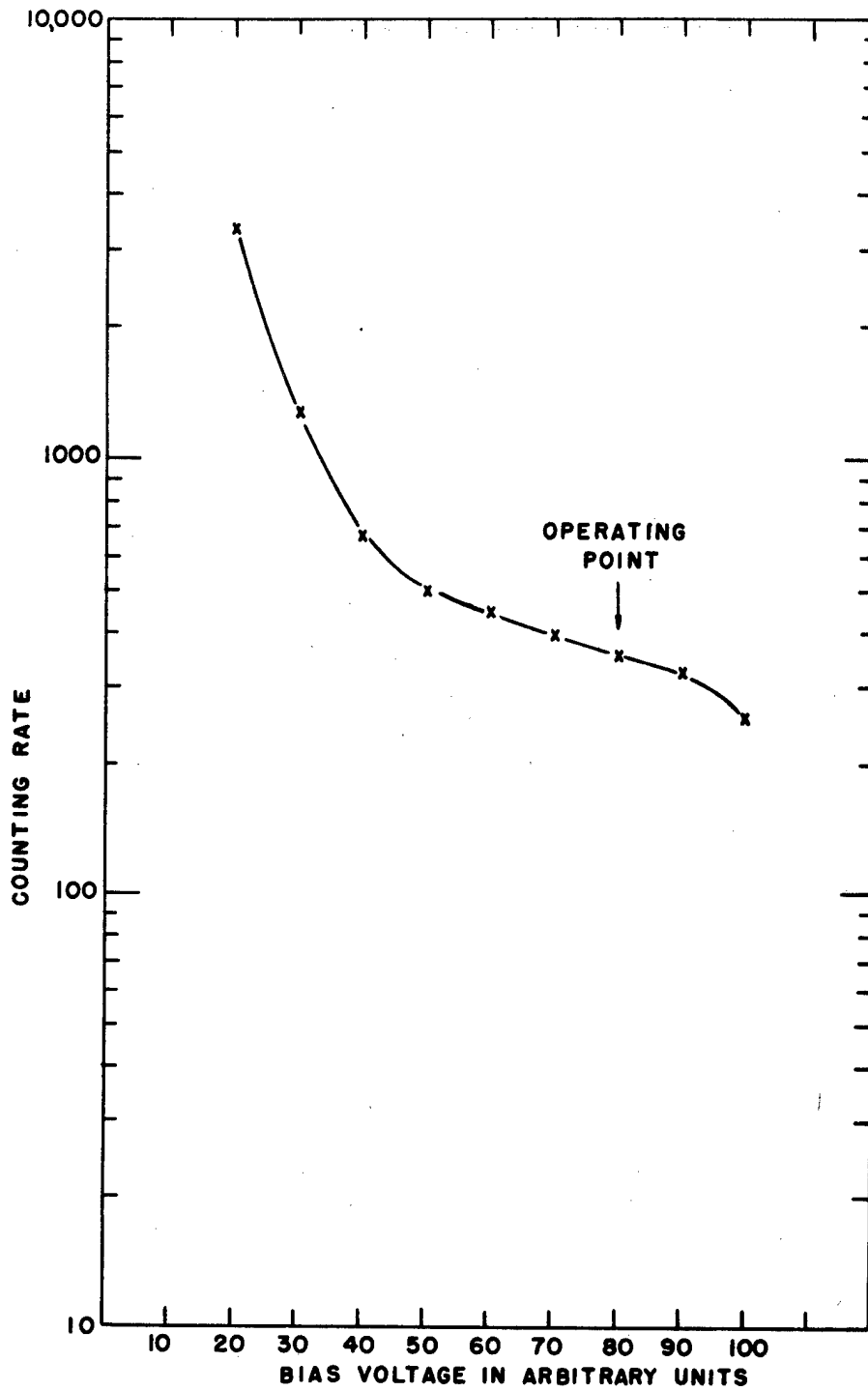
Fig. 3--Sample counting rate versus bias voltage curve for a bismuth fission chamber.
