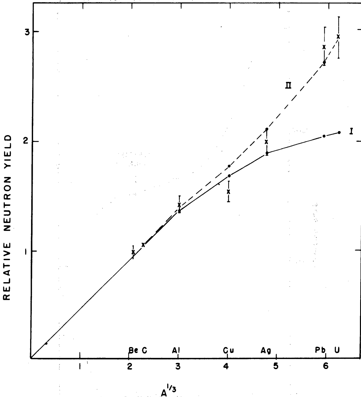
Fig. 4--Relative neutron yields in the forward direction from targets bombarded with 190 Mev deuterons. The crosses are the observed neutron yields in the forward direction in arbitrary units. Curve I (solid) shows the values predicted by stripping theory. Curve II (dotted) shows the values obtained by adding a function proportional to Z^2 to the stripping theory values. A probable error of \pm 6 per cent is shown on each point except the value for carbon to which the other values are relative.
