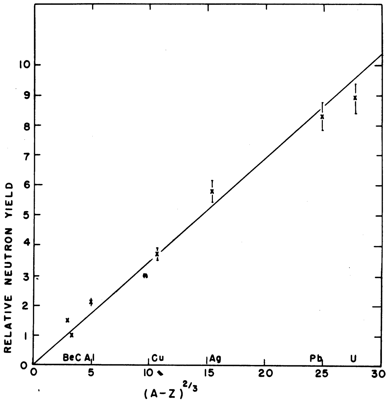
Fig. 5--Relative neutron yields in the forward direction from targets bombarded with 350 Mev protons.
