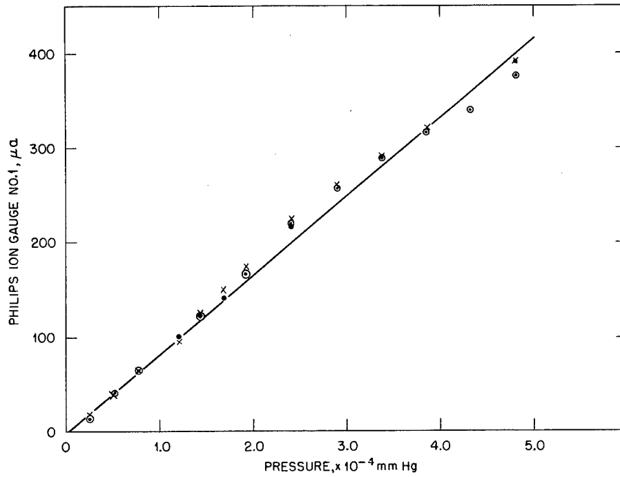
Chart No. X-1149--Philips ion gauge characteristic, range 2. Secondary E ≈ 2050 v. Primary E=115 v. H=3350 oersteds. Data taken: ○○○○, 3-17-44; xxxx, 3-18-44; ....., 3-21-44.
