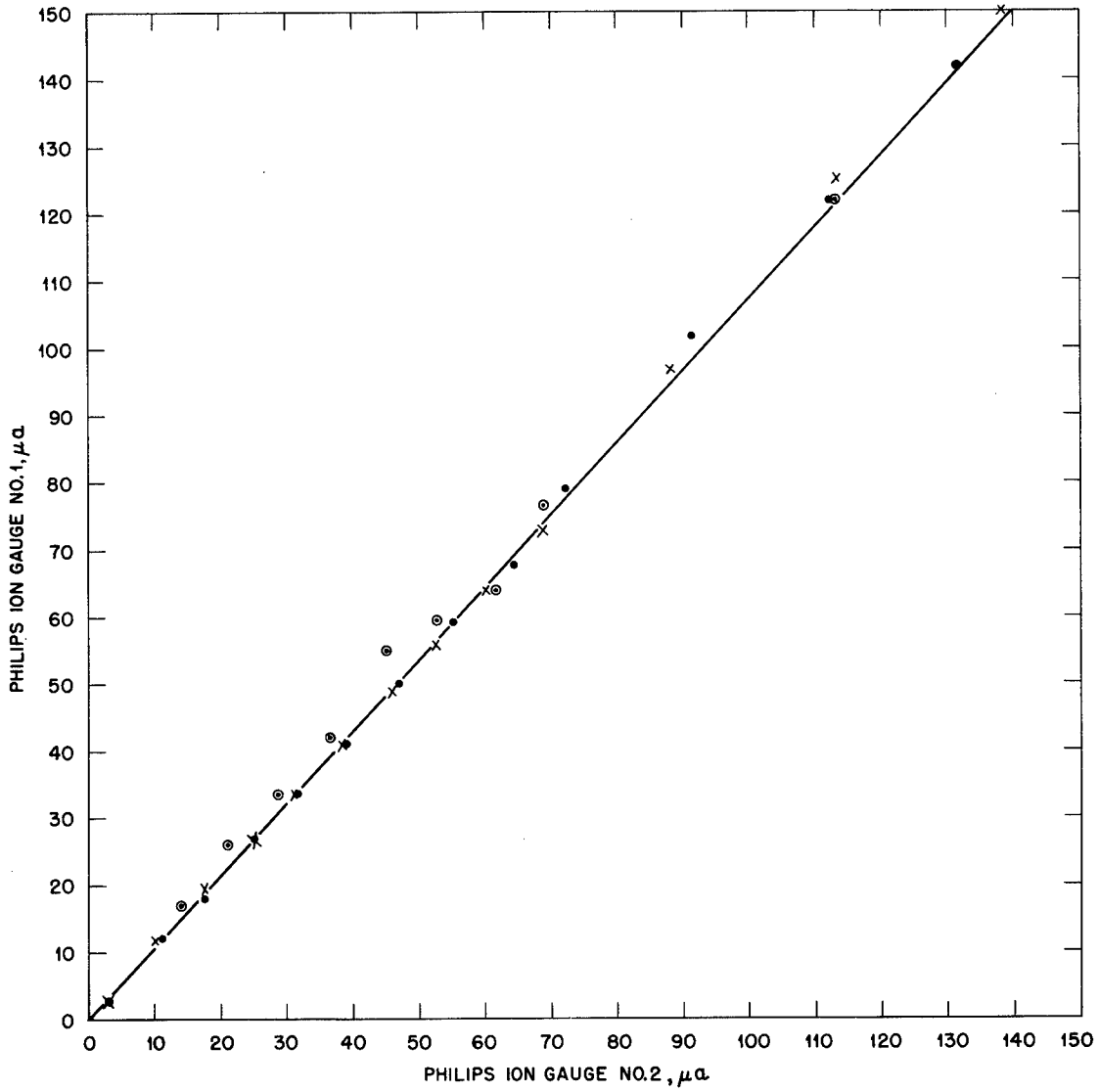
Chart No. X-1151--Comparison of Philips ion gauges, low range. Secondary E \approx 2050 v. Primary E=115 v. H=3350 oersteds. Data taken: ○○○○, 3-17-44; xxxx, 3-18-44; ....., 3-21-44.
