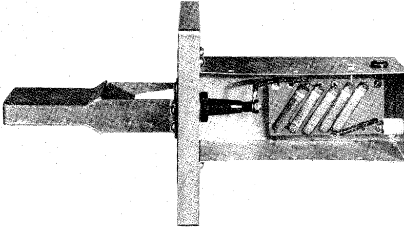
Spec. 259--A standard Philips ion gauge mounted on a small E window plate. Notice the isolantite sleeve protecting the B. G. mica spark plug. The cover for the ballast resistor box is not shown in this picture.
