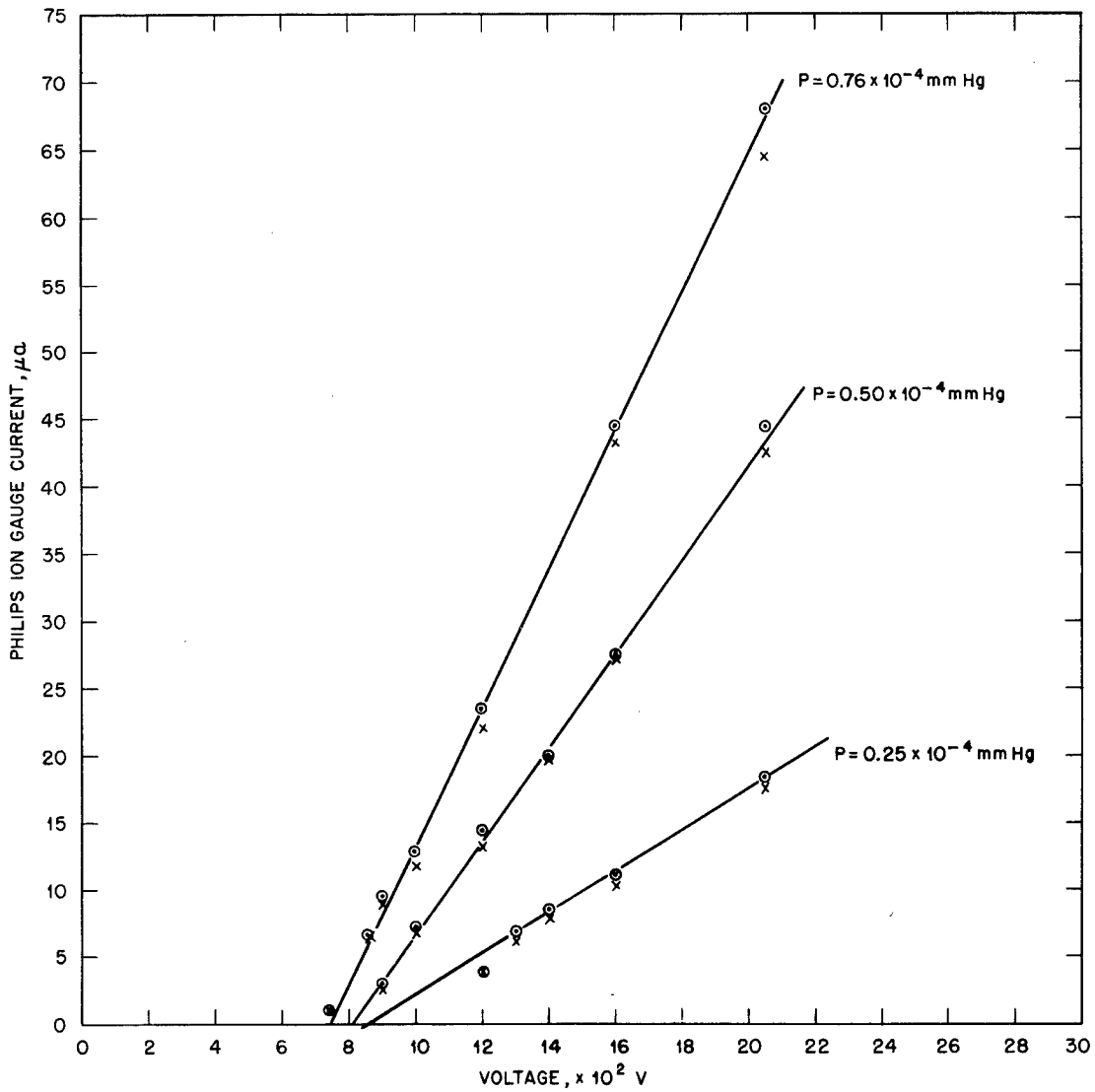
Chart No. X-1153--Philips ion gauge volt-ampere characteristic. H=3350 oersteds. \circ\circ\circ\circ , gauge No. 1. \times\times\times\times , gauge No. 2.
